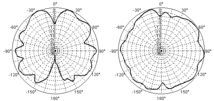
E-Plane Pattern
