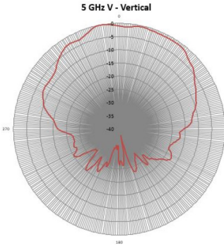
E-Plane Pattern
