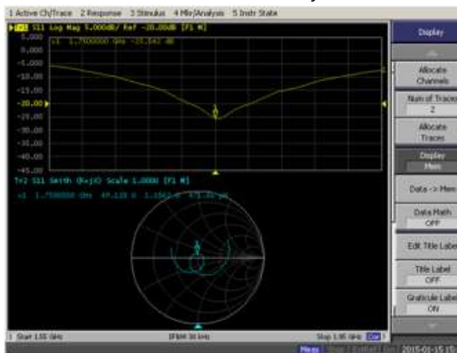
Measurement Plot for Body TSL
