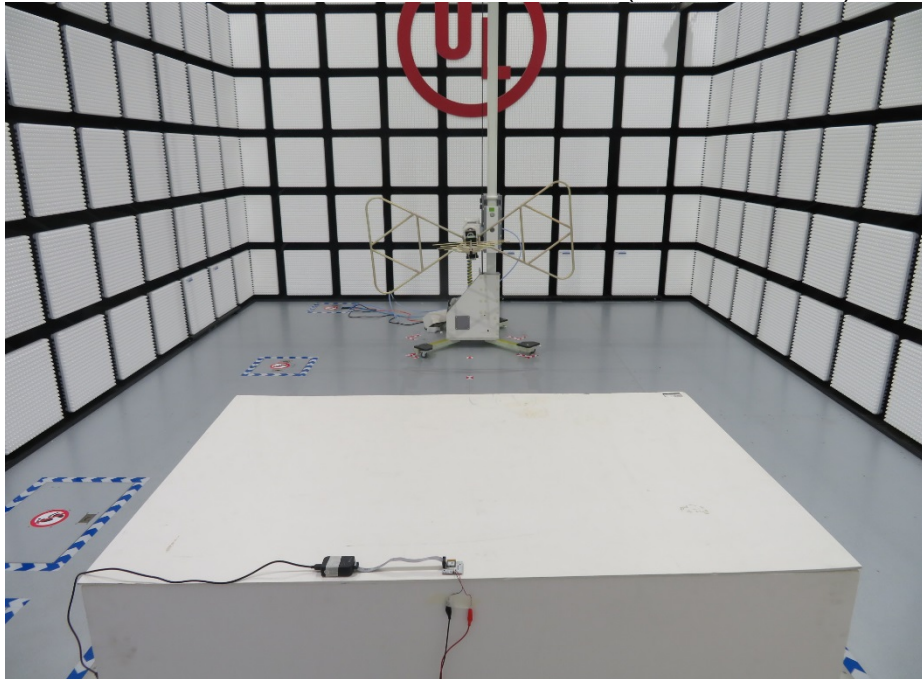
RADIATED RF MEASUREMENT SETUP (30MHz ~ 1 GHz)
