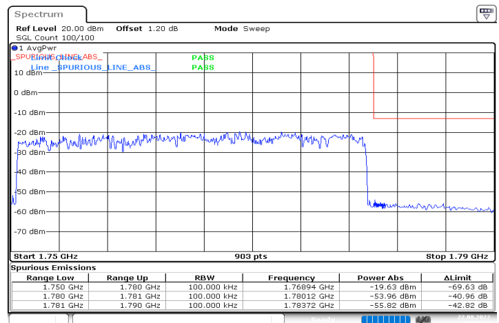
n66_30MHz_15kHz_1765MHz_DFT-s-OFDM QPSK_RB160@0
