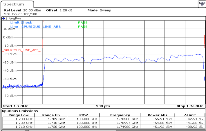
n66_40MHz_15kHz_1730MHz_DFT-s-OFDM QPSK_RB216@0
