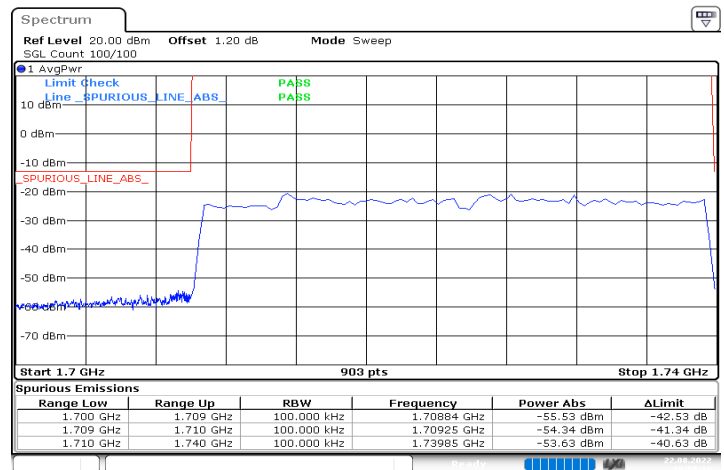
n66_30MHz_15kHz_1725MHz_DFT-s-OFDM QPSK_RB160@0
