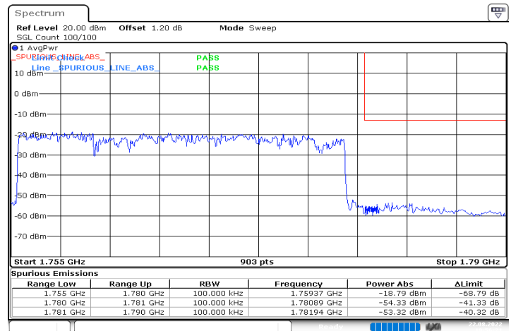
n66_25MHz_15kHz_1767.5MHz_DFT-s-OFDM QPSK_RB128@0
