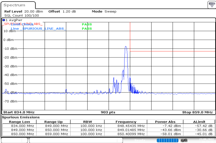
n5_15MHz_15kHz_841.5MHz_DFT-s-OFDM QPSK_RB1@78
