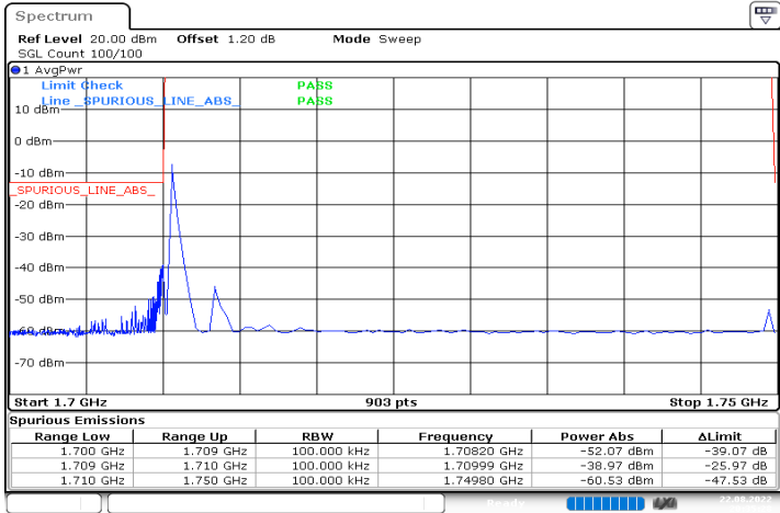
n66_40MHz_15kHz_1730MHz_DFT-s-OFDM QPSK_RB1@0
