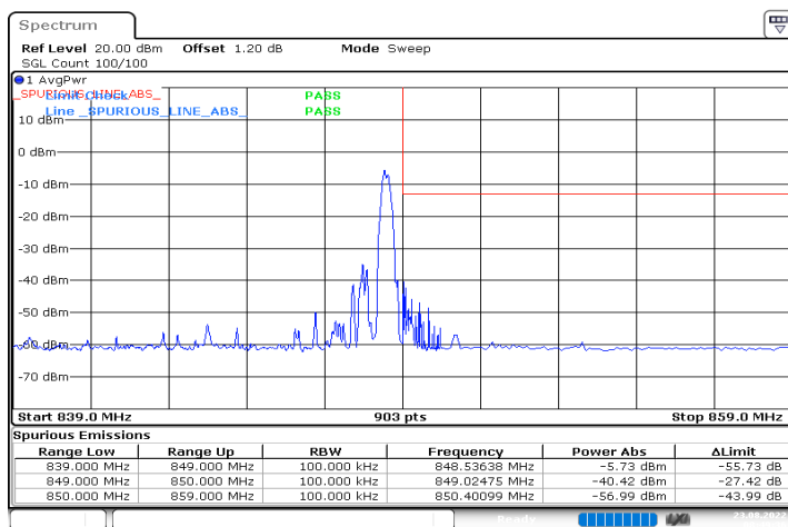
n5_10MHz_15kHz_844MHz_DFT-s-OFDM QPSK_RB1@51
