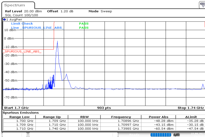
n66_30MHz_15kHz_1725MHz_DFT-s-OFDM QPSK_RB1@0
