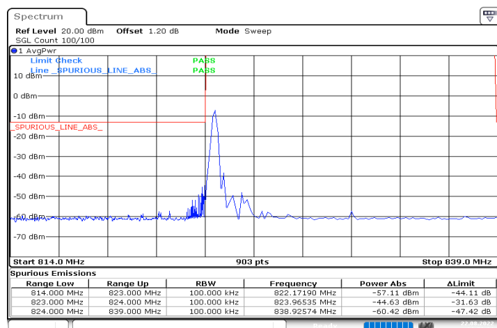
n5_15MHz_15kHz_831.5MHz_DFT-s-OFDM QPSK_RB1@0
