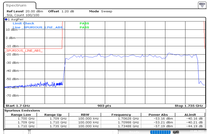
n66_25MHz_15kHz_1722.5MHz_DFT-s-OFDM QPSK_RB128@0
