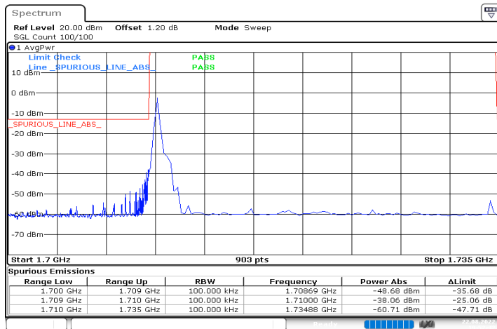
n66_25MHz_15kHz_1722.5MHz_DFT-s-OFDM QPSK_RB1@0
