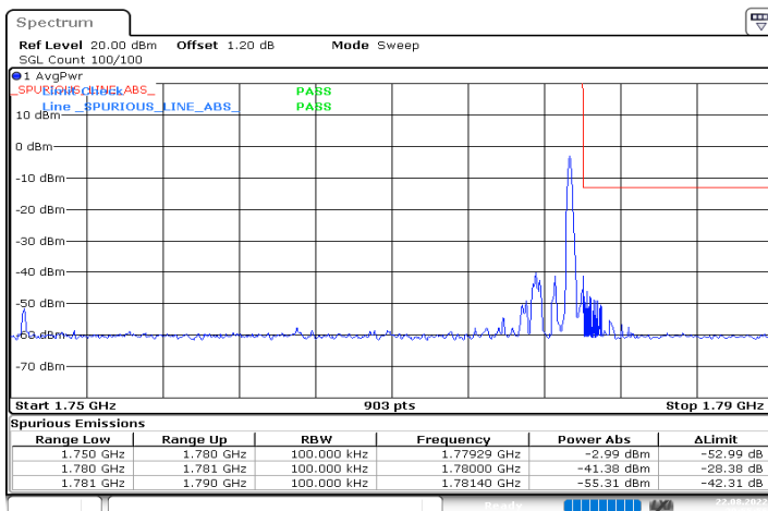
n66_30MHz_15kHz_1765MHz_DFT-s-OFDM QPSK_RB1@159
