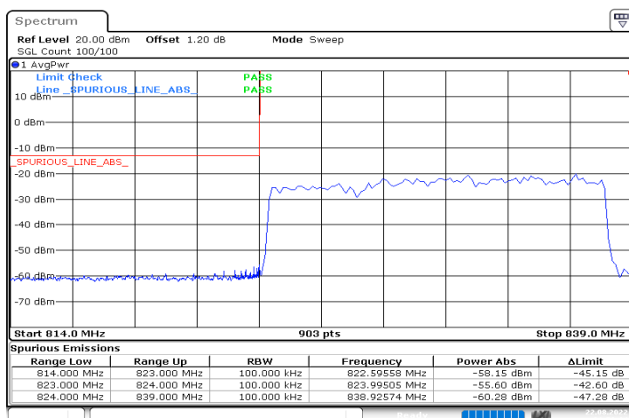
n5_15MHz_15kHz_831.5MHz_DFT-s-OFDM QPSK_RB75@0
