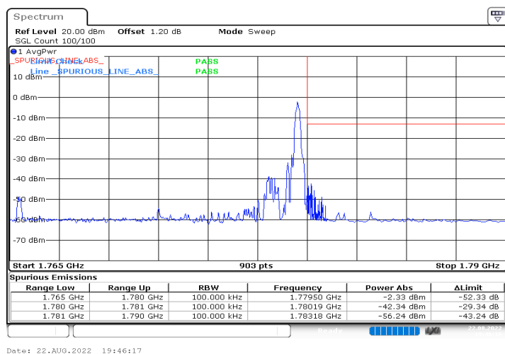
n66_15MHz_15kHz_1772.5MHz_DFT-s-OFDM QPSK_RB1@78
