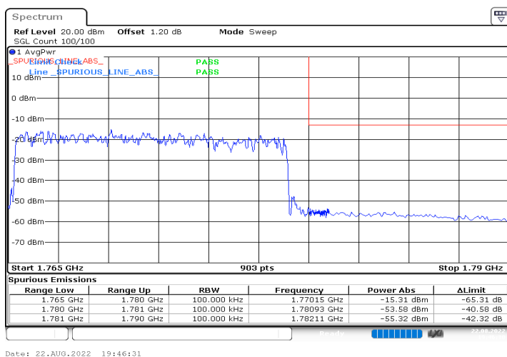
n66_15MHz_15kHz_1772.5MHz_DFT-s-OFDM QPSK_RB75@0
