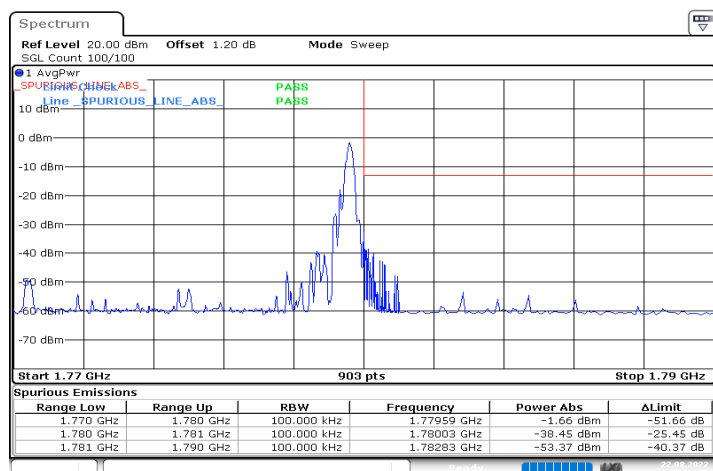
n66_10MHz_15kHz_1775MHz_DFT-s-OFDM QPSK_RB1@51
