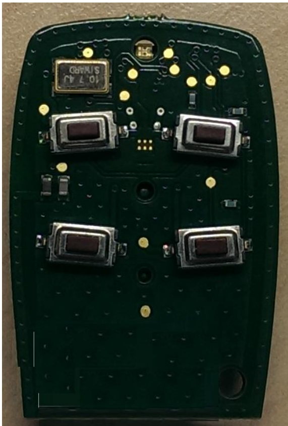
BOTTOM OF PCB
