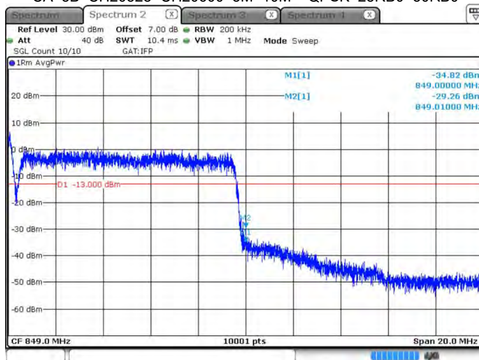
CA 5B CH20528+CH20600 5M+10M QPSK 25RB0+50RB0
