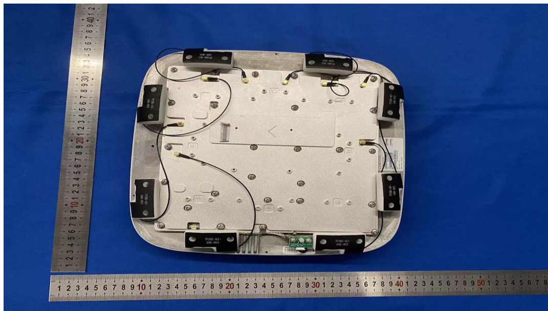
Internal Antenna
