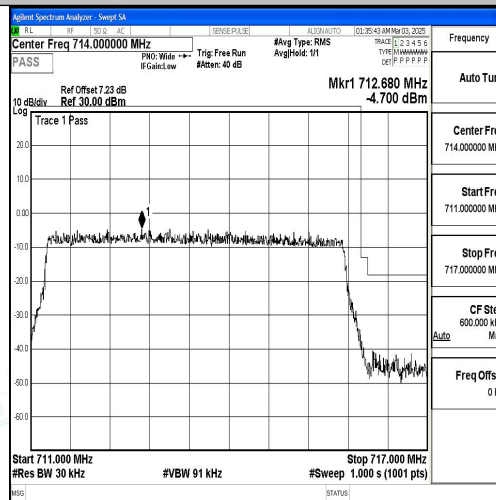
Band17_5MHz_16QAM_23825_25RB#0
