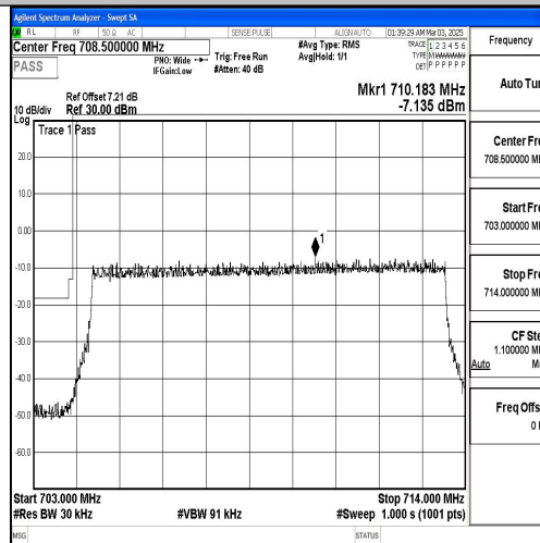
Band17_10MHz_QPSK_23780_50RB#0
