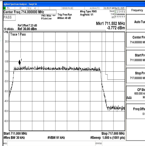
Band17_5MHz_QPSK_23825_25RB#0
