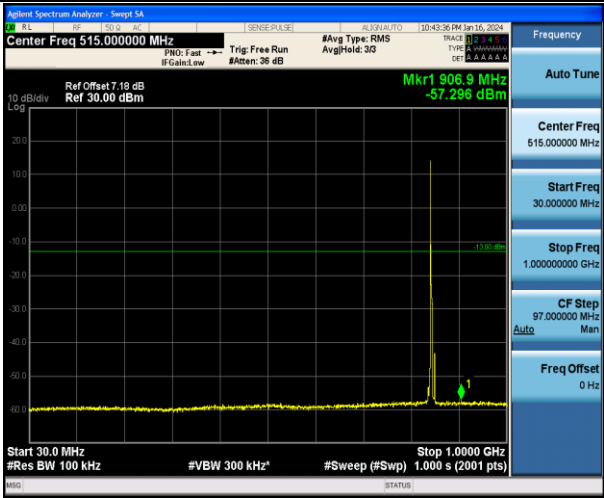
Band5_5MHz_16QAM_20625_1RB#0_30~1000_30~1000
