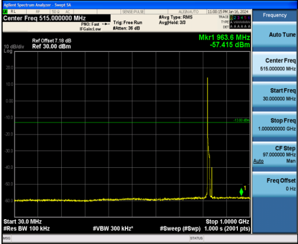
Band5_10MHz_16QAM_20450_1RB#0_30~1000_30~1000
