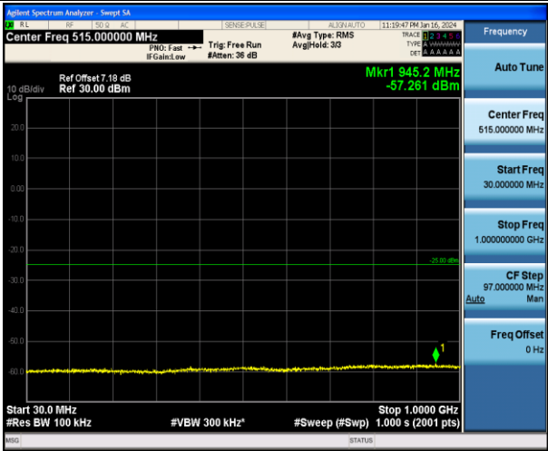
Band7_5MHz_16QAM_21100_1RB#0_30~1000_30~1000
