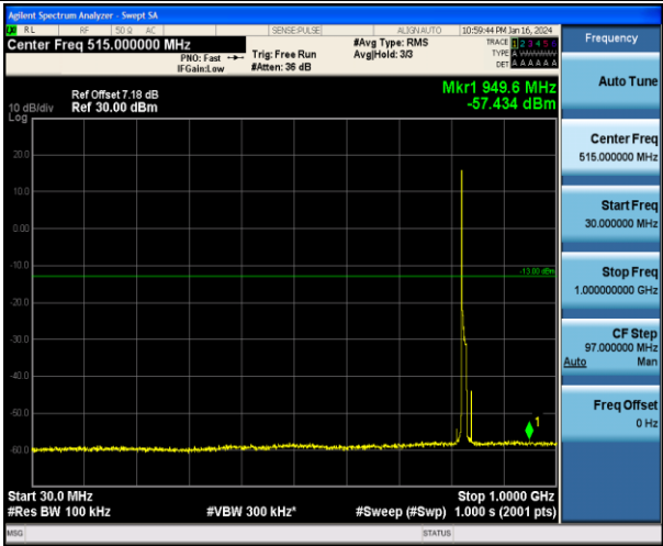
Band5_10MHz_QPSK_20450_1RB#0_30~1000_30~1000
