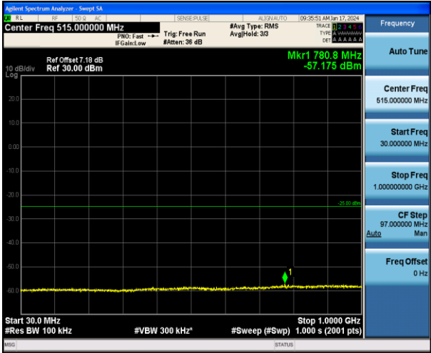
Band7_15MHz_QPSK_21375_1RB#0_30~1000_30~1000
