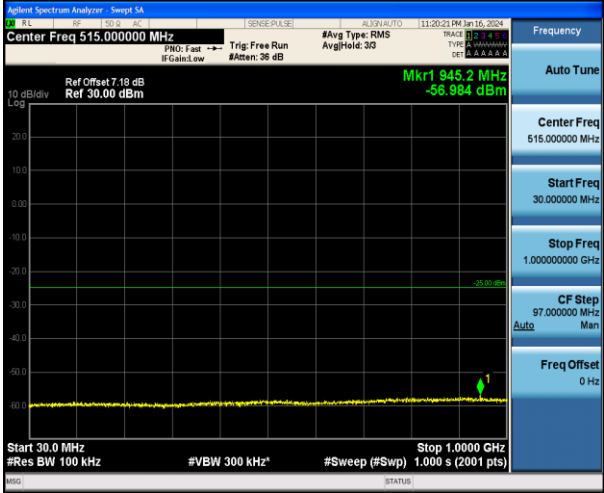
Band7_5MHz_QPSK_21425_1RB#0_30~1000_30~1000
