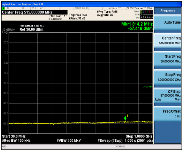
Band7_15MHz_16QAM_21100_1RB#0_30~1000_30~1000
