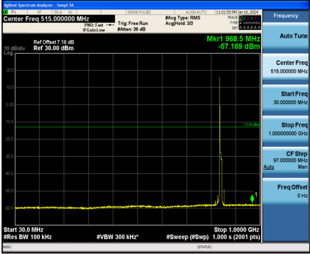
Band5_10MHz_QPSK_20600_1RB#0_30~1000_30~1000
