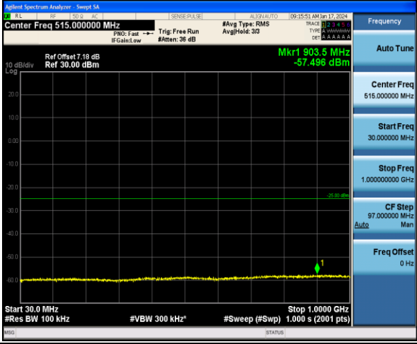
Band7_10MHz_16QAM_20800_1RB#0_30~1000_30~1000
