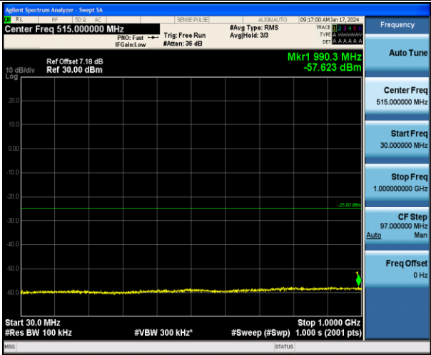
Band7_10MHz_16QAM_21100_1RB#0_30~1000_30~1000
