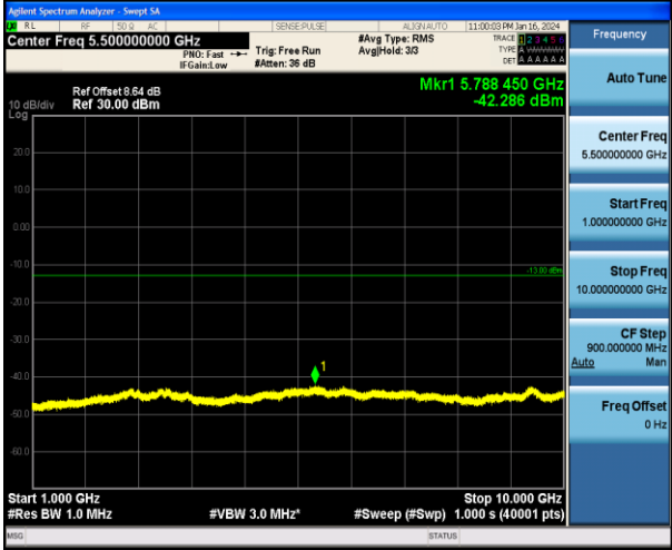
Band5_10MHz_QPSK_20450_1RB#0_1000~10000_1000~10000
