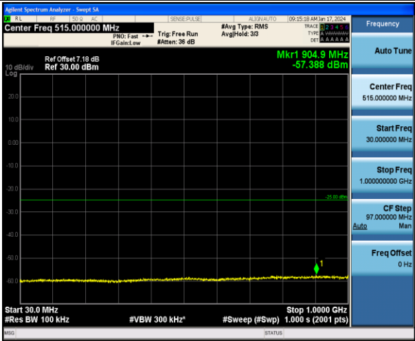
Band7_10MHz_QPSK_20800_1RB#0_30~1000_30~1000
