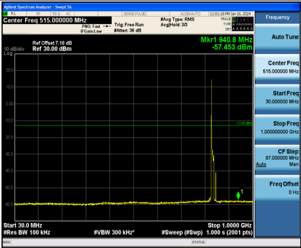
Band5_10MHz_16QAM_20525_1RB#0_30~1000_30~1000
