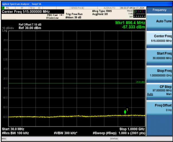
Band7_15MHz_QPSK_20825_1RB#0_30~1000_30~1000
