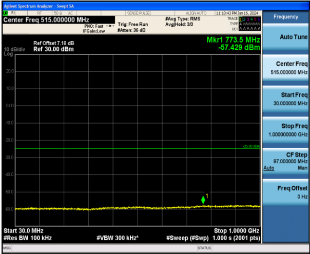
Band7_5MHz_16QAM_20775_1RB#0_30~1000_30~1000
