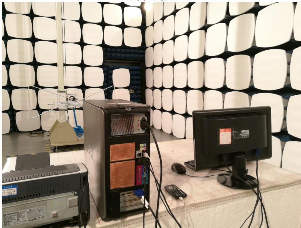
Radiated Emission(for PC mode) Below 1GHz
