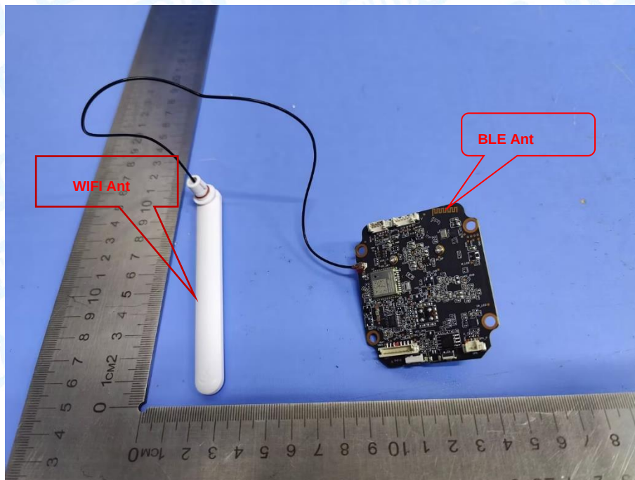
Photo 10 Antenna Appearance
