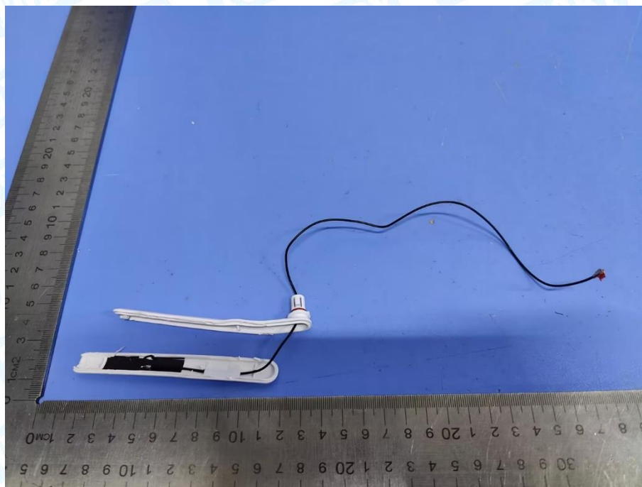
Photo 10 Antenna Appearance
