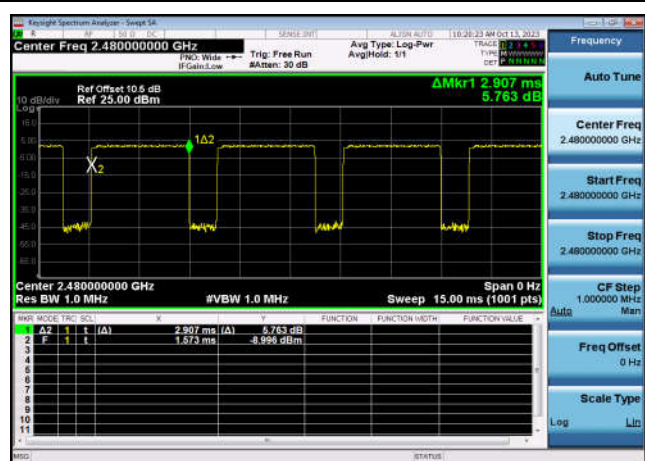
8DPSK,2480,3DH5,Transmission Time
