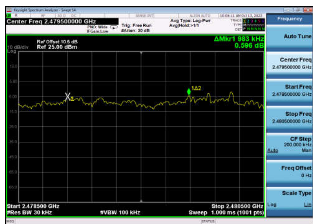
8DPSK,Hopping3DH5,2478.5~2480.5
