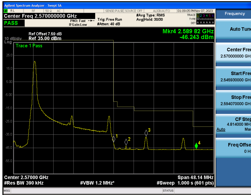
Band7-20MHz-16QAM-21350-1RB#99
