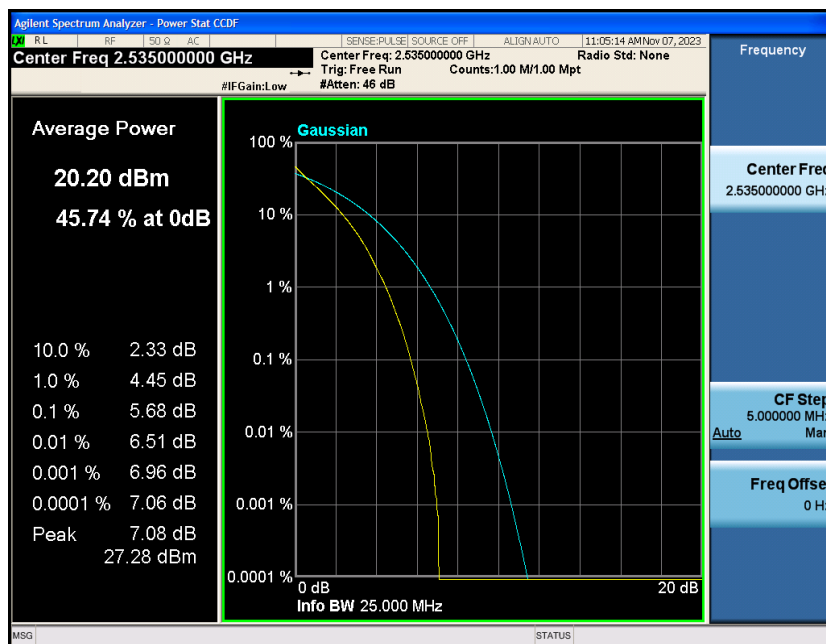
Band7-10MHz-QPSK-21400-1RB#0
