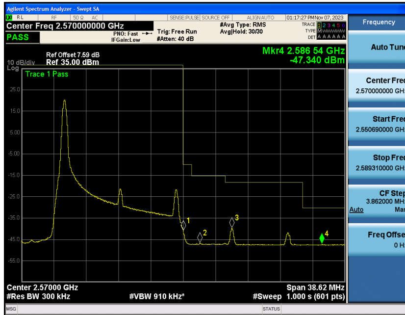
Band7-15MHz-16QAM-21375-1RB#74
