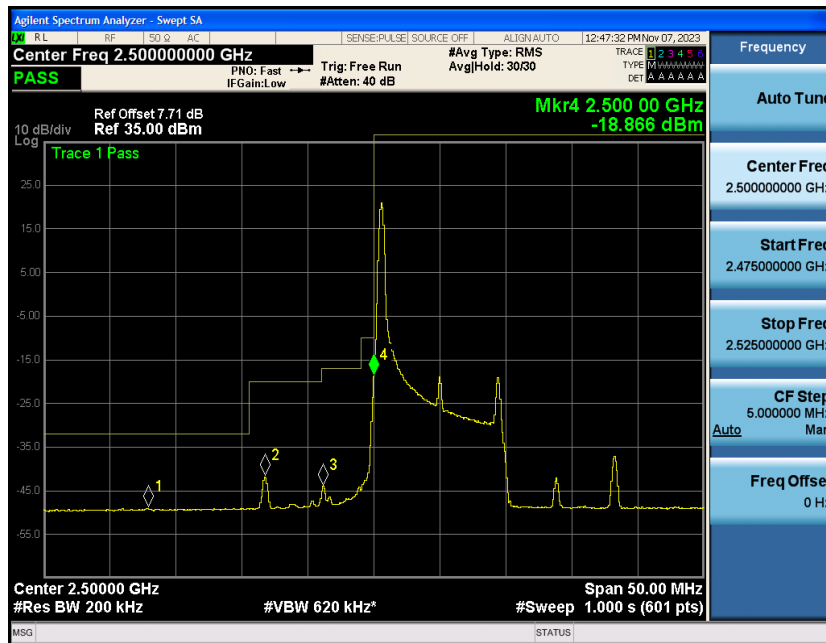
Band7-10MHz-QPSK-20800-1RB#49
