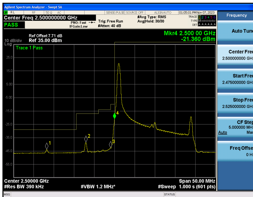
Band7-20MHz-16QAM-20850-1RB#99
