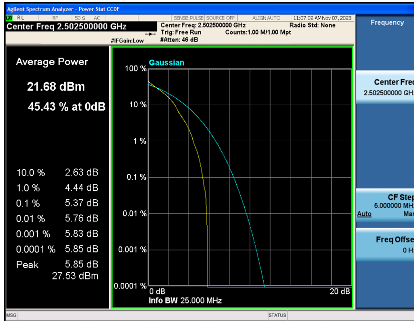
Band7-5MHz-QPSK-20775-25RB#0
