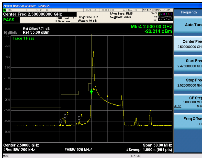
Band7-10MHz-16QAM-20800-1RB#49
