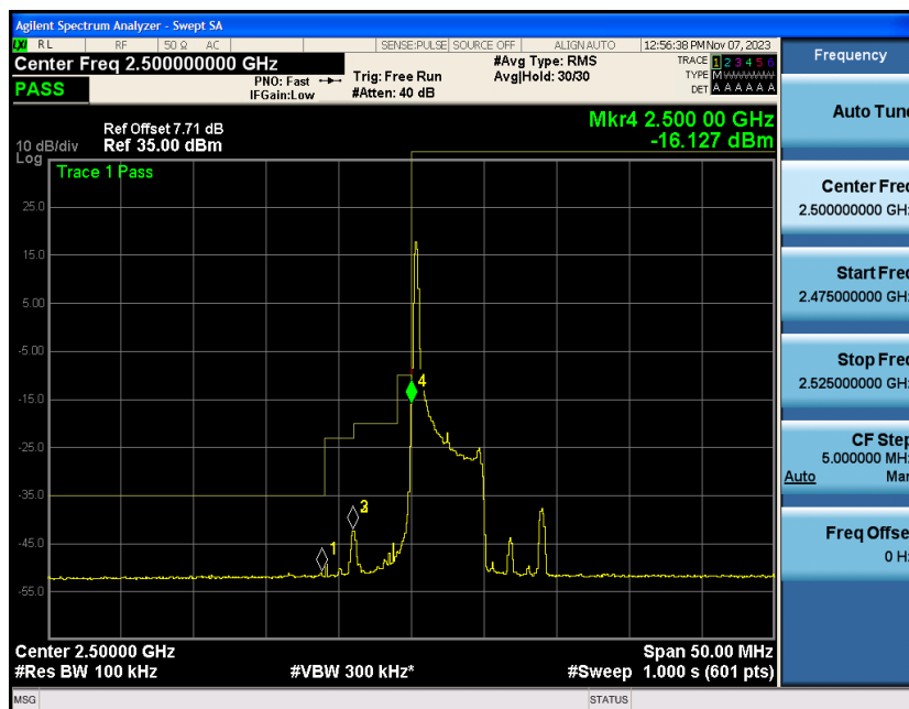
Band7-5MHz-16QAM-20775-1RB#24
