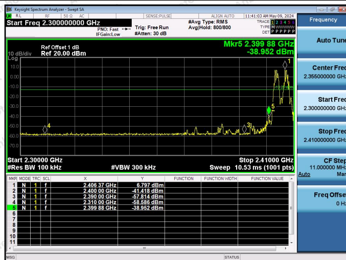
2.4G-Ant1-Hop_2403-PASS
