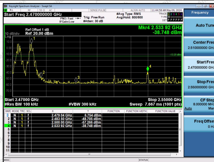
2.4G-Ant1-Hop_2479-PASS
