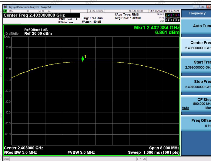
2.4G-Ant1-2403-PASS
