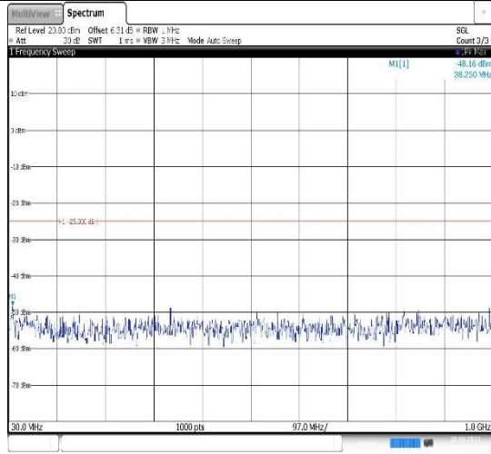
Band41-5MHz-16QAM-41565-1RB#0- Range1:30~1000MHz
