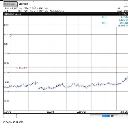
Band41-15MHz-QPSK-40620-1RB#0- Range2:1000~26500MHz
