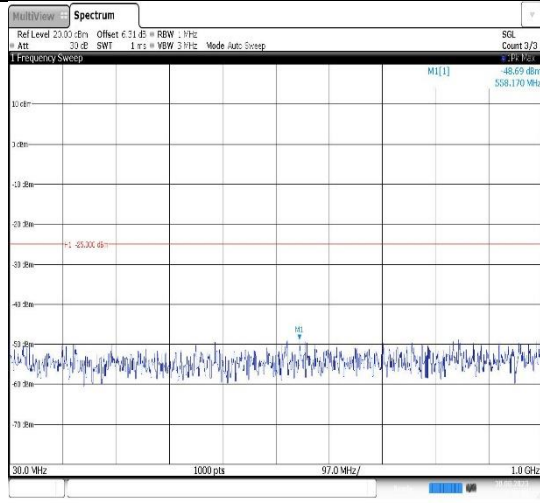
Band41-15MHz-QPSK-40620-1RB#0- Range1:30~1000MHz
