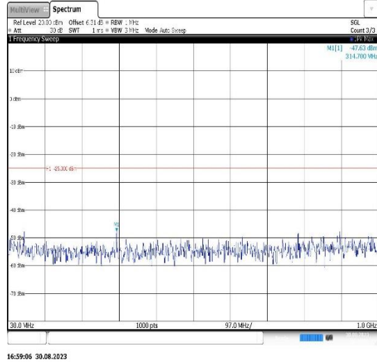
Band41-5MHz-QPSK-41565-1RB#0- Range1:30~1000MHz
