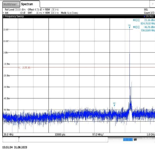
Band26(824-849)-15MHz-16QAM-26865-1RB#0-Range1:30~1000MHz
