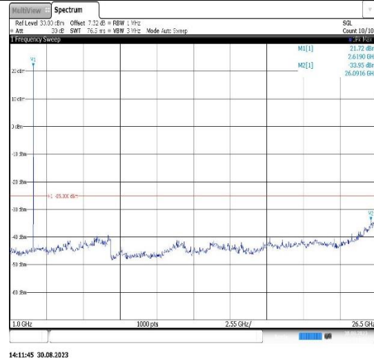
Band38-10MHz-16QAM-37800-1RB#0- Range2:1000~26500MHz
