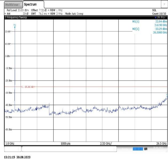
Band38-5MHz-16QAM-37775-1RB#0- Range2:1000~26500MHz
