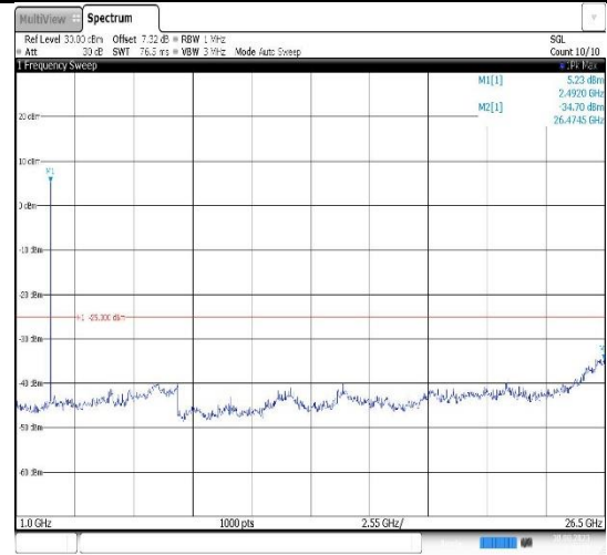
Band41-15MHz-16QAM-40620-1RB#0- Range2:1000~26500MHz
