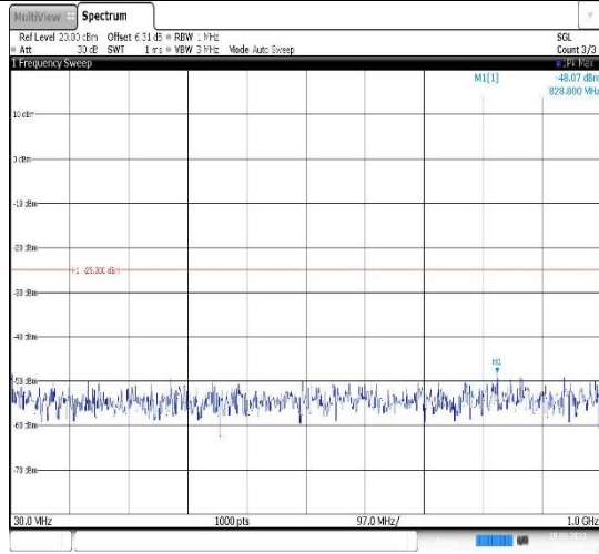
Band41-20MHz-QPSK-41490-1RB#0- Range1:30~1000MHz
