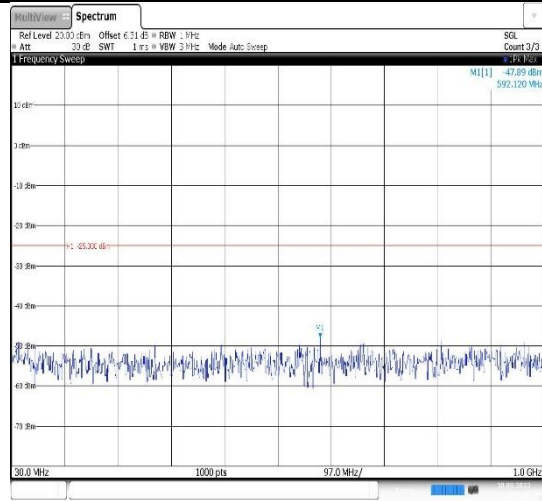
Band38-5MHz-16QAM-38000-1RB#0- Range1:30~1000MHz
