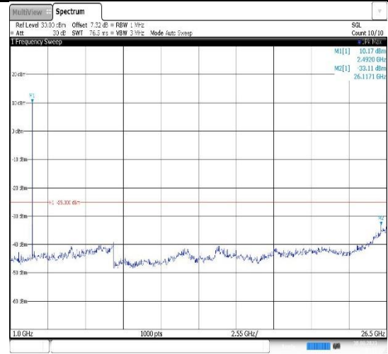
Band41-10MHz-16QAM-40620-1RB#0- Range2:1000~26500MHz
