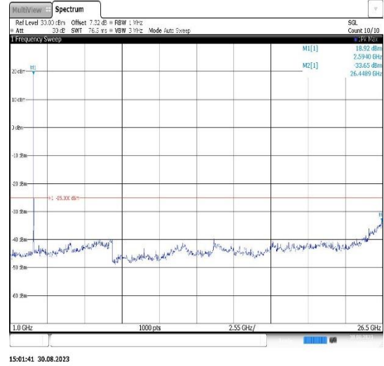
Band38-15MHz-QPSK-38175-1RB#0- Range2:1000~26500MHz
