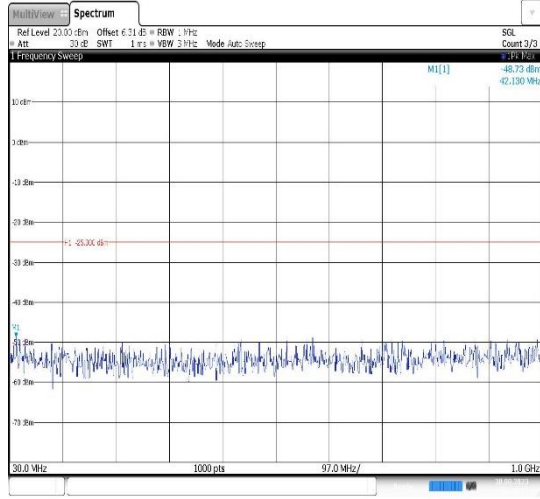
Band41-5MHz-16QAM-40620-1RB#0- Range1:30~1000MHz
