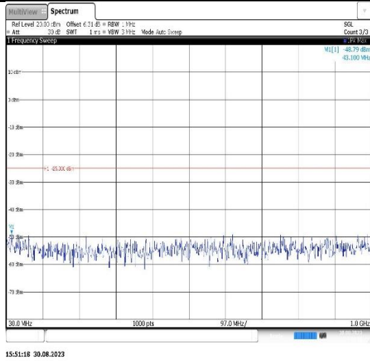
Band38-20MHz-QPSK-38000-1RB#0- Range1:30~1000MHz
