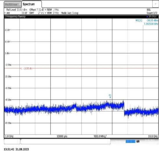
Band26(824-849)-15MHz-16QAM-26865-1RB#0-Range2:1000~10000MHz
