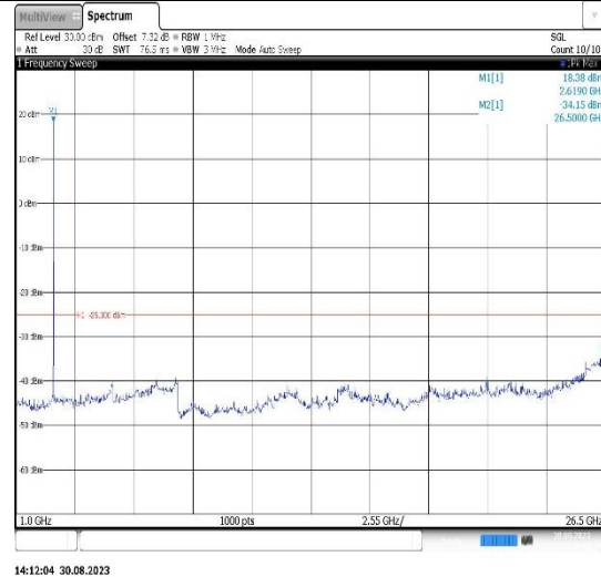
Band38-15MHz-QPSK-37825-1RB#0- Range2:1000~26500MHz
