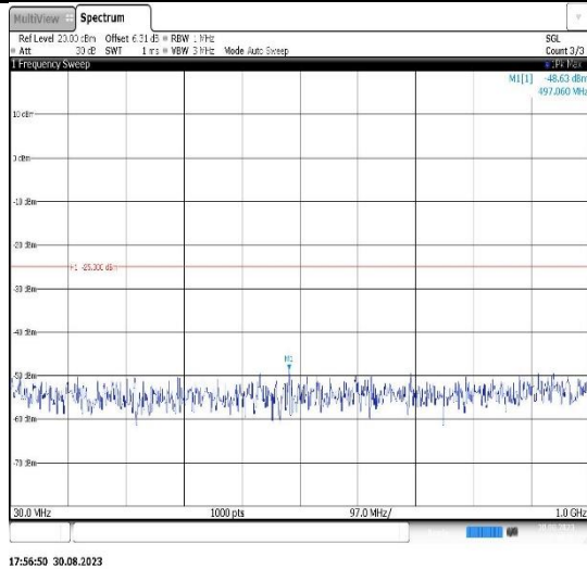
Band41-15MHz-QPSK-40620-1RB#0- Range1:30~1000MHz
