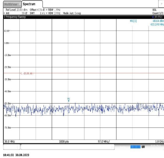
Band41-20MHz-16QAM-41490-1RB#0- Range1:30~1000MHz
