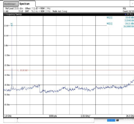
Band41-15MHz-QPSK-40620-1RB#0- Range2:1000~26500MHz
