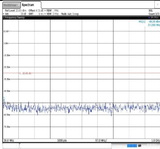
Band41-10MHz-16QAM-40620-1RB#0- Range1:30~1000MHz
