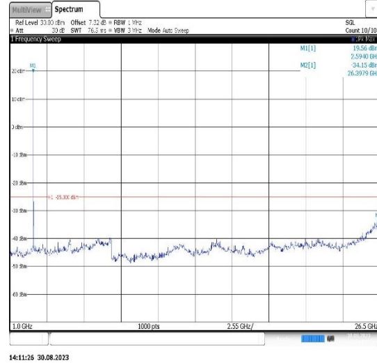
Band38-10MHz-16QAM-38200-1RB#0- Range2:1000~26500MHz
