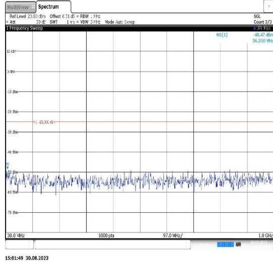
Band38-15MHz-16QAM-38175-1RB#0- Range1:30~1000MHz
