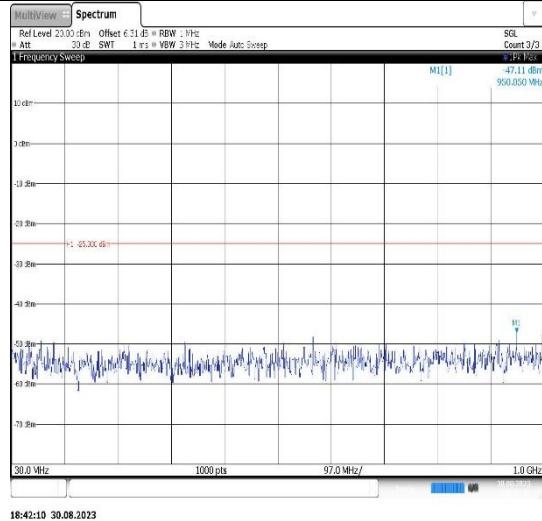
Band66-1.4MHz-QPSK-131979-1RB#0- Range1:30~1000MHz
