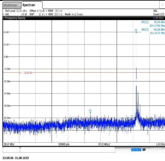
Band26(824-849)-15MHz-16QAM-26915-1RB#0- Range1:30~1000MHz
