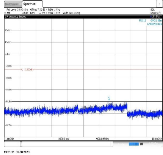
Band26(824-849)-15MHz-16QAM-26965-1RB#0- Range2:1000~10000MHz
