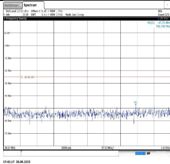
Band41-10MHz-QPSK-40620-1RB#0- Range1:30~1000MHz
