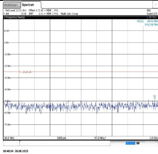
Band41-20MHz-16QAM-40620-1RB#0- Range1:30~1000MHz
