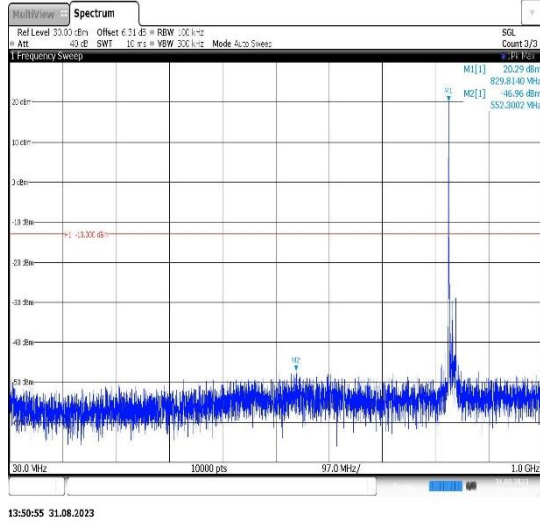
Band26(824-849)-15MHz-QPSK-26965-1RB#0-Range1:30~1000MHz
