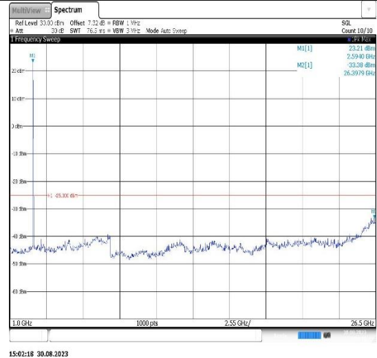
Band38-15MHz-16QAM-37825-1RB#0- Range2:1000~26500MHz
