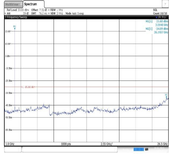
Band38-5MHz-16QAM-38225-1RB#0- Range2:1000~26500MHz
