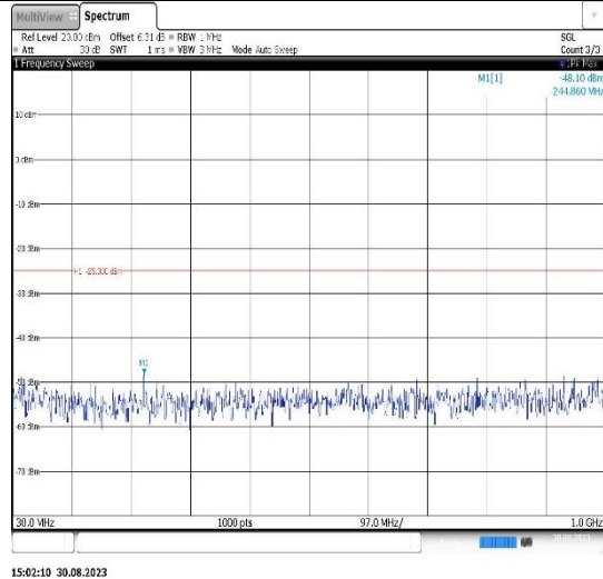
Band38-15MHz-16QAM-37825-1RB#0- Range1:30~1000MHz
