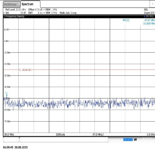
Band41-5MHz-16QAM-39675-1RB#0- Range1:30~1000MHz
