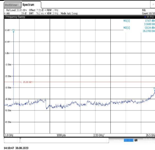
Band38-10MHz-16QAM-38000-1RB#0- Range2:1000~26500MHz
