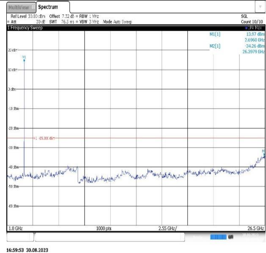
Band41-5MHz-16QAM-39675-1RB#0- Range2:1000~26500MHz
