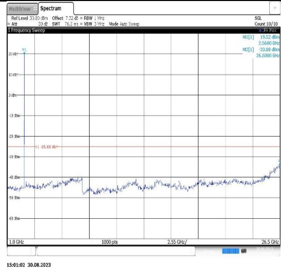
Band38-15MHz-QPSK-38000-1RB#0- Range2:1000~26500MHz
