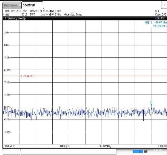
Band38-20MHz-16QAM-38000-1RB#0- Range1:30~1000MHz
