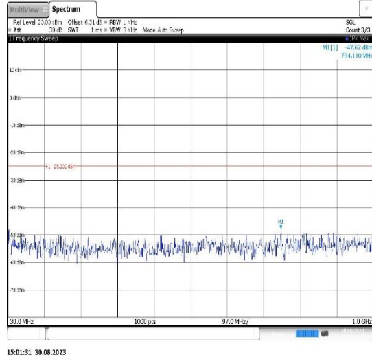
Band38-15MHz-QPSK-38175-1RB#0- Range1:30~1000MHz
