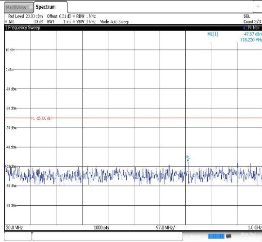
Band41-10MHz-16QAM-41540-1RB#0- Range1:30~1000MHz
