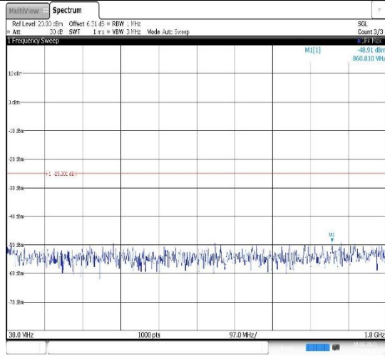
Band38-20MHz-16QAM-38150-1RB#0- Range1:30~1000MHz
