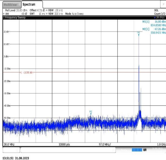
.Band38-5MHz-QPSK-37775-1RB#0- Range1:30~1000MHz
