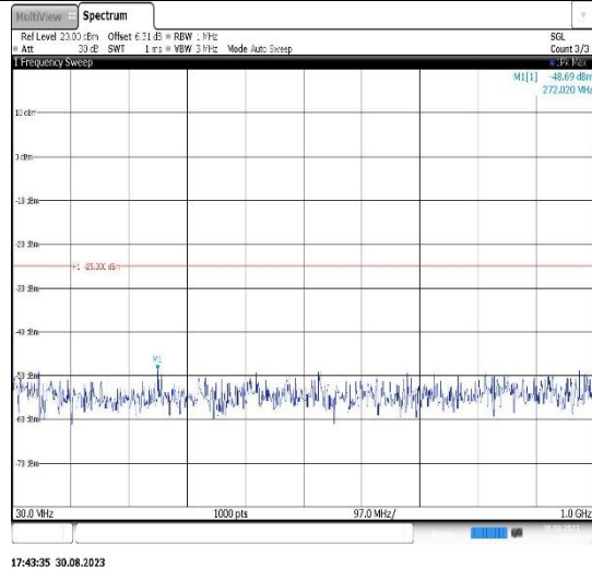
Band41-10MHz-16QAM-39700-1RB#0- Range1:30~1000MHz
