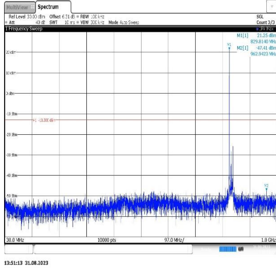
Band26(824-849)-15MHz-16QAM-26965-1RB#0- Range1:30~1000MHz
