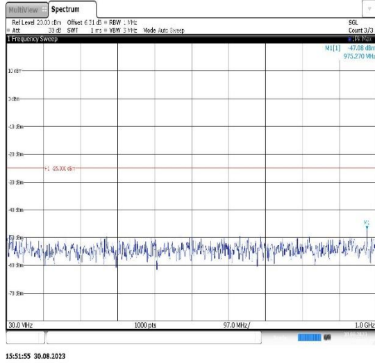
Band38-20MHz-QPSK-38150-1RB#0- Range1:30~1000MHz
