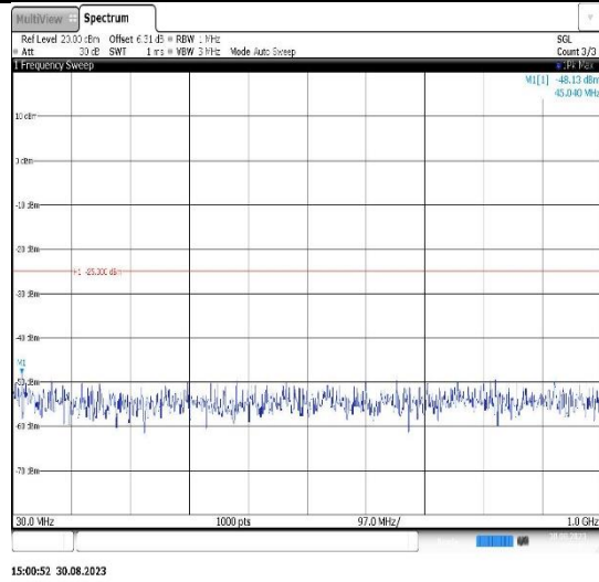
Band38-15MHz-QPSK-38000-1RB#0- Range1:30~1000MHz
