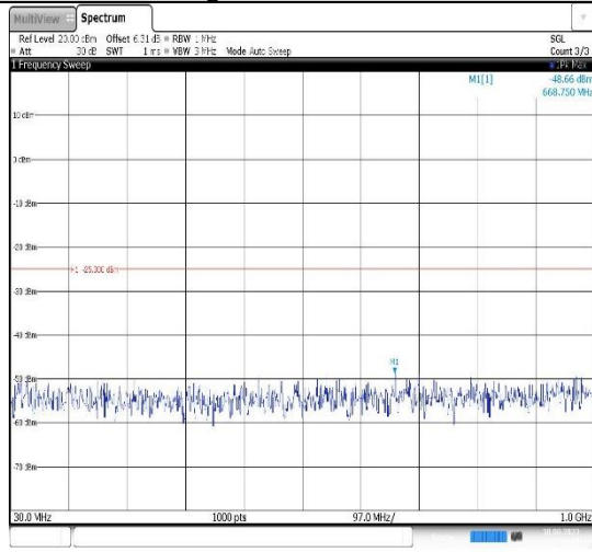
Band41-15MHz-QPSK-41515-1RB#0- Range1:30~1000MHz
