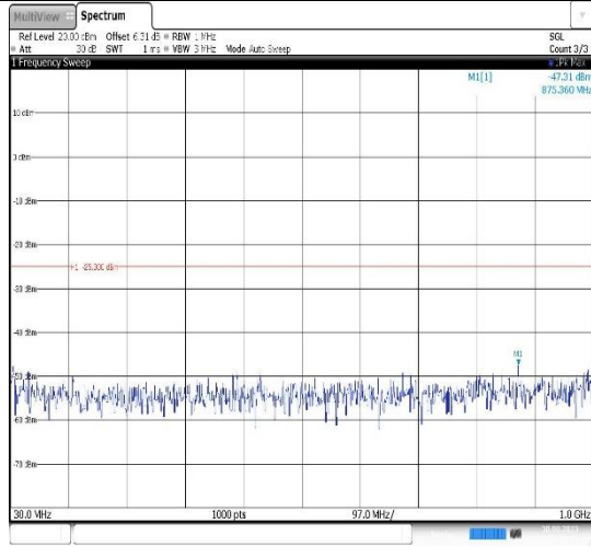
Band41-15MHz-16QAM-41515-1RB#0- Range1:30~1000MHz
