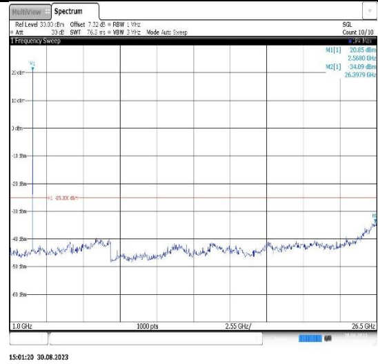
Band38-15MHz-16QAM-38000-1RB#0- Range2:1000~26500MHz
