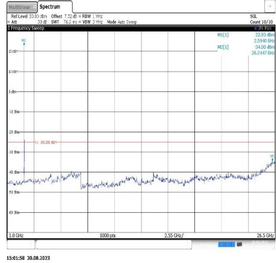
Band38-15MHz-16QAM-38175-1RB#0- Range2:1000~26500MHz
