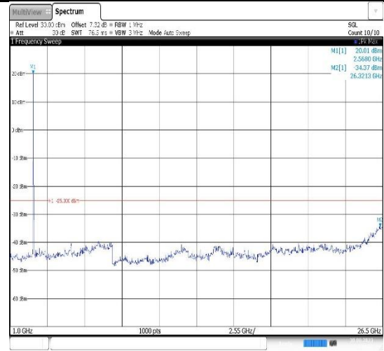
Band38-20MHz-16QAM-38000-1RB#0- Range2:1000~26500MHz
