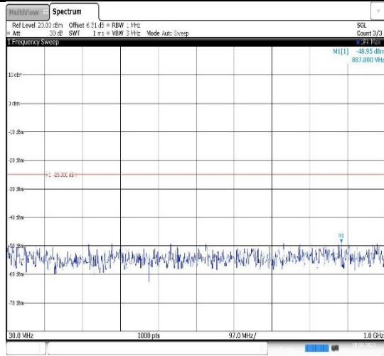
Band41-20MHz-QPSK-40620-1RB#0- Range1:30~1000MHz
