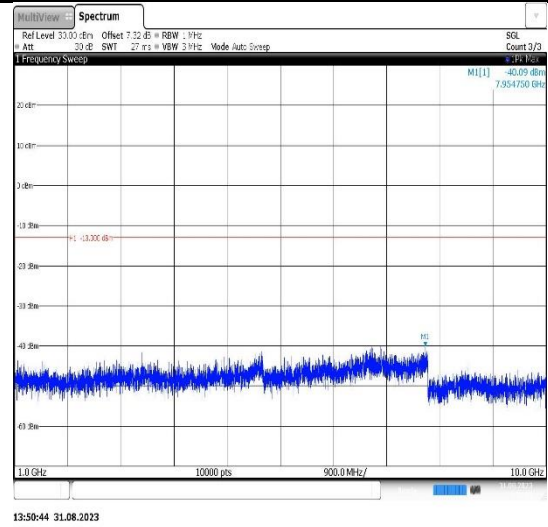
Band26(824-849)-15MHz-16QAM-26915-1RB#0- Range2:1000~10000MHz
