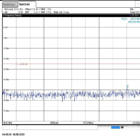
Band38-10MHz-QPSK-38000-1RB#0- Range1:30~1000MHz
