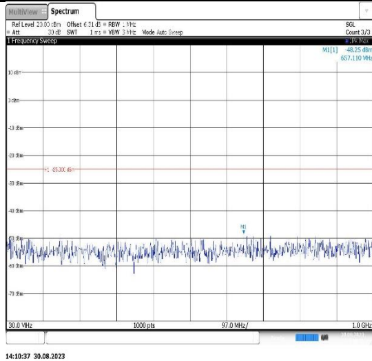
Band38-10MHz-16QAM-38000-1RB#0- Range1:30~1000MHz
