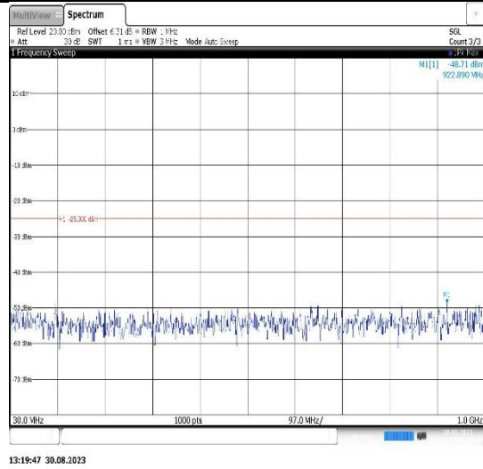
Band38-5MHz-QPSK-38000-1RB#0- Range1:30~1000MHz
