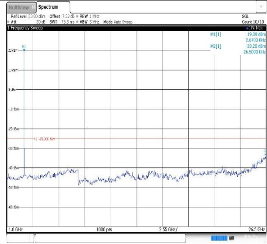
Band41-10MHz-16QAM-41540-1RB#0- Range2:1000~26500MHz
