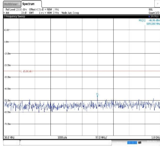
Band38-5MHz-16QAM-38225-1RB#0- Range1:30~1000MHz
