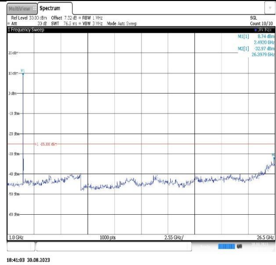
Band41-20MHz-16QAM-40620-1RB#0- Range2:1000~26500MHz
