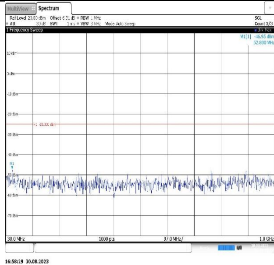
Band41-5MHz-QPSK-40620-1RB#0- Range1:30~1000MHz
