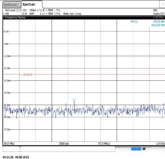
Band38-10MHz-16QAM-37800-1RB#0- Range1:30~1000MHz
