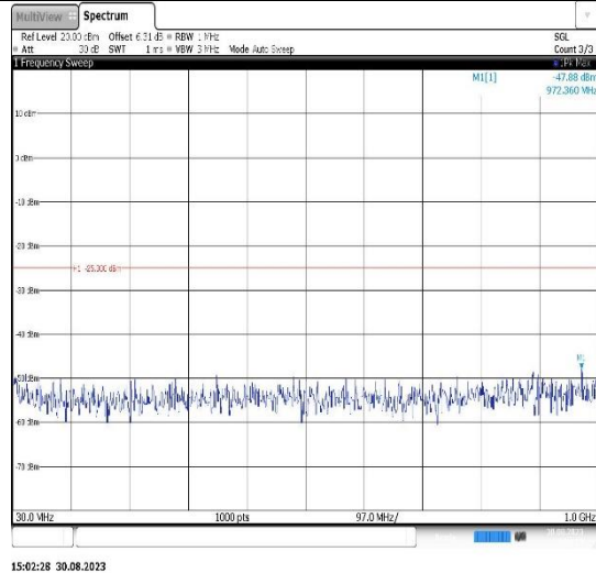
Band38-20MHz-QPSK-37850-1RB#0- Range1:30~1000MHz
