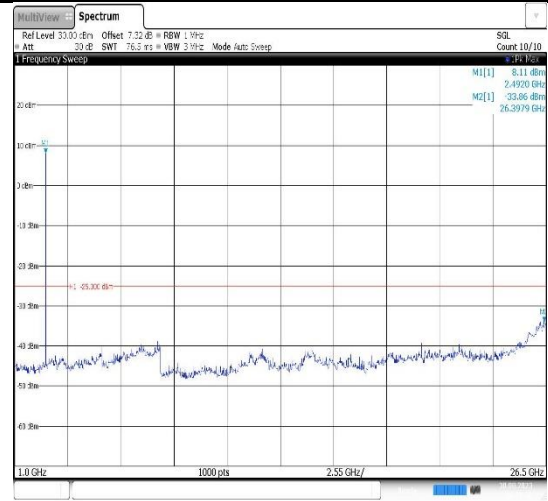
Band41-5MHz-16QAM-40620-1RB#0- Range2:1000~26500MHz
