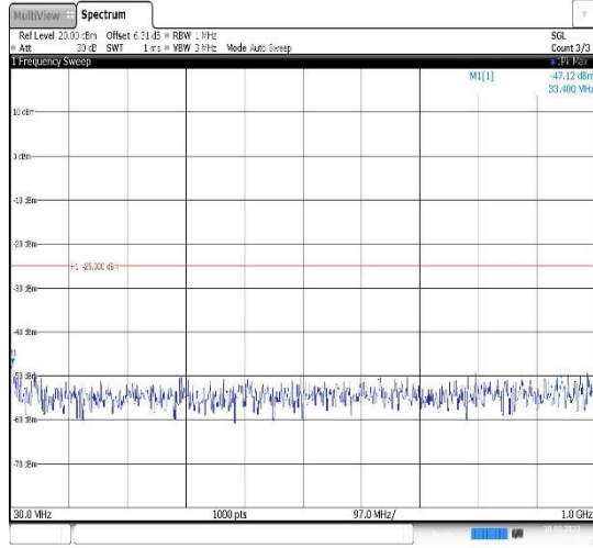
Band41-15MHz-16QAM-40620-1RB#0- Range1:30~1000MHz
