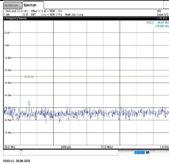
Band38-15MHz-16QAM-38000-1RB#0- Range1:30~1000MHz
