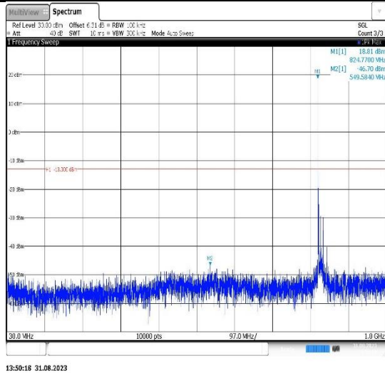
Band26(824-849)-15MHz-QPSK-26915-1RB#0-Range1:30~1000MHz
