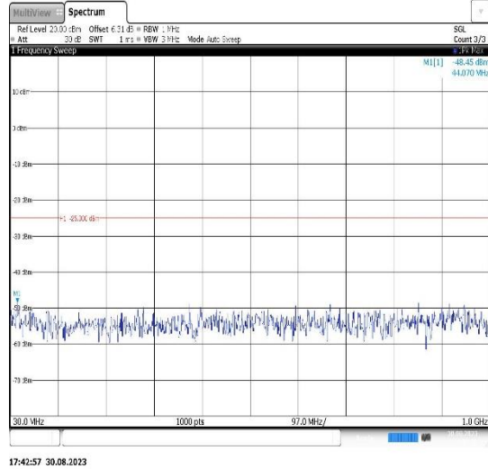
Band41-10MHz-QPSK-41540-1RB#0- Range1:30~1000MHz
