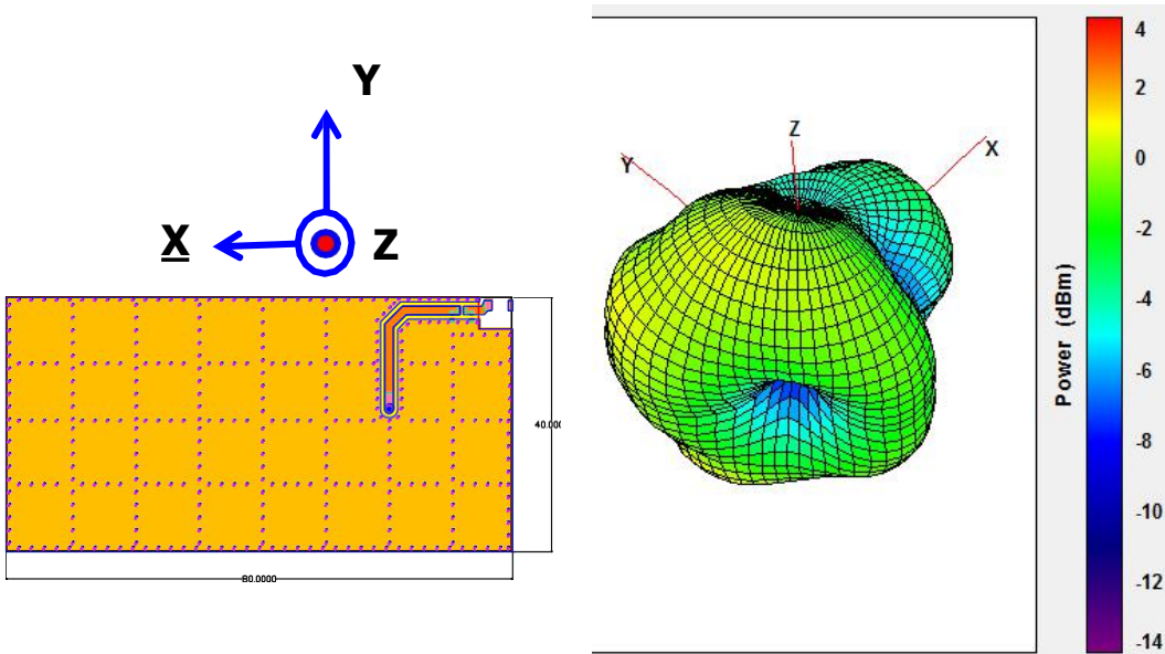
Radiation Pattern
