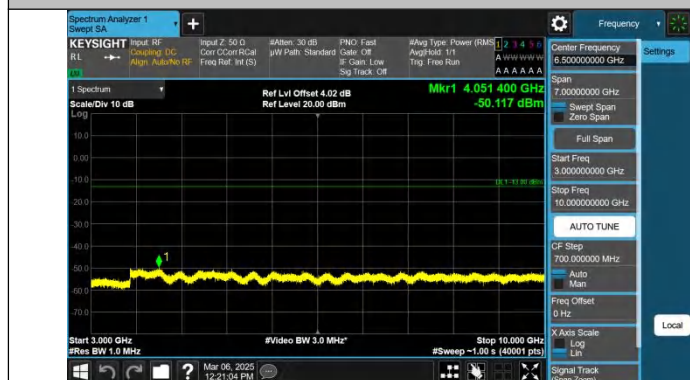
Band12-5MHz-QPSK-23155-1RB#0-3000~10000-PASS
