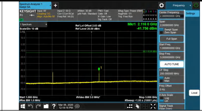
Band12-5MHz-QPSK-23095-1RB#0-1000~3000-PASS
