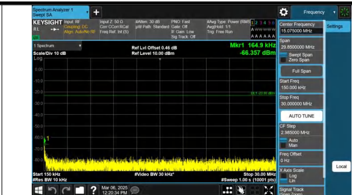
Band12-5MHz-QPSK-23155-1RB#0-0.15~30-PASS
