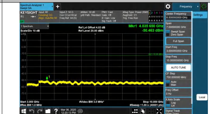
Band12-5MHz-QPSK-23095-1RB#24-3000~10000-PASS
