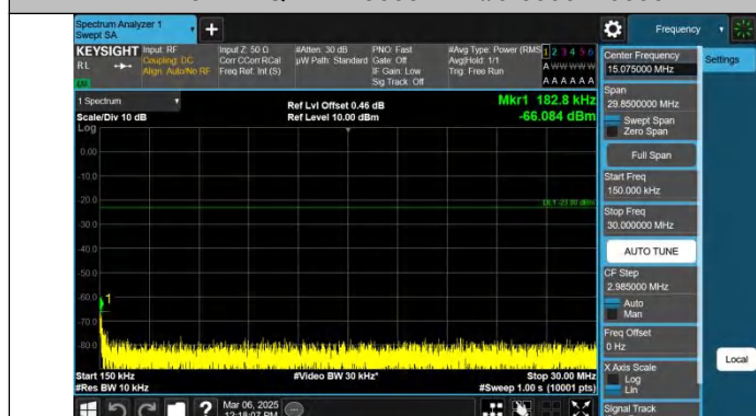
Band12-5MHz-QPSK-23035-1RB#24-0.15~30-PASS
