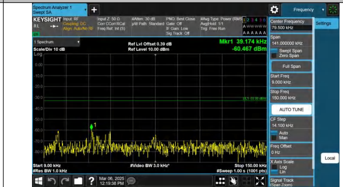
Band12-5MHz-QPSK-23095-1RB#24-0.009~0.15-PASS
