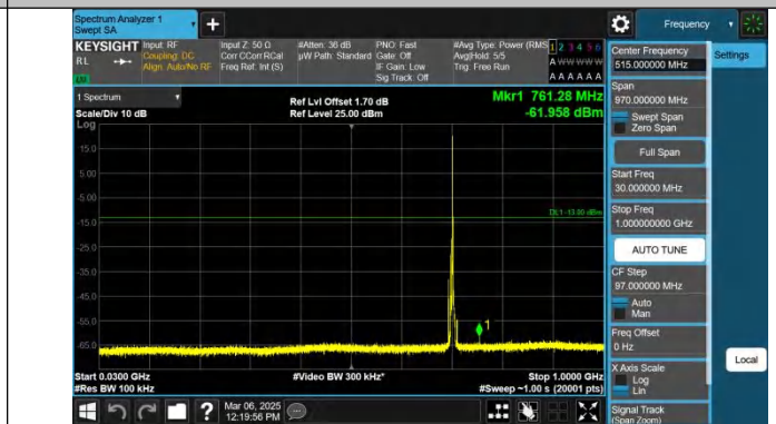
Band12-5MHz-QPSK-23095-1RB#24-30~1000-PASS
