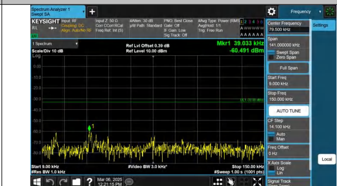
Band12-5MHz-QPSK-23155-1RB#24-0.009~0.15-PASS
