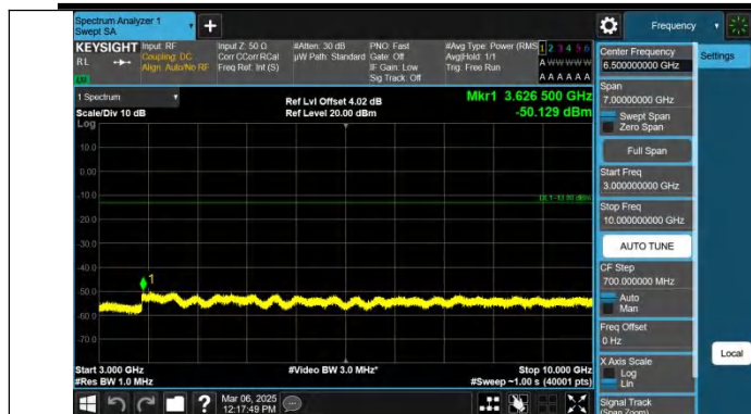
Band12-5MHz-QPSK-23035-1RB#0-3000~10000-PASS
