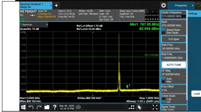
Band12-5MHz-QPSK-23095-1RB#0-30~1000-PASS
