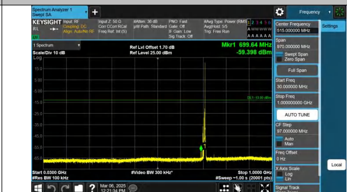
Band12-5MHz-QPSK-23155-1RB#24-30~1000-PASS
