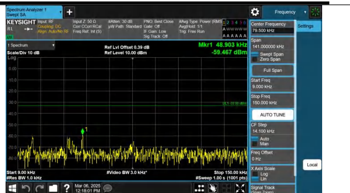
Band12-5MHz-QPSK-23035-1RB#24-0.009~0.15-PASS
