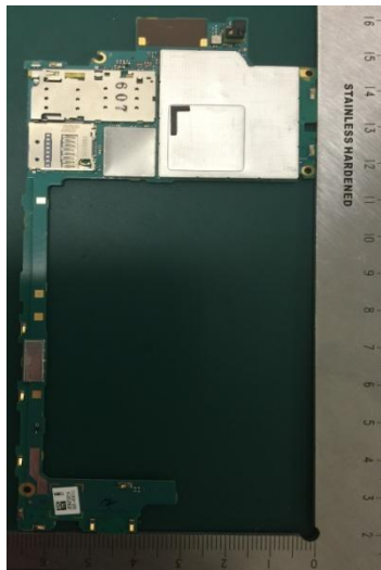
Internal PWB with Shield cases (Rear-side) Internal PWB without Shield cases (Rear-side)
