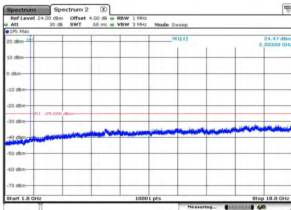
B7_CH20775_5M_1RB12_QPSK_Above 1G
