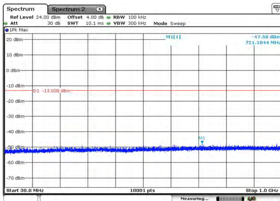
B66_CH131979_1.4M_1RB2_QPSK_Below 1G
