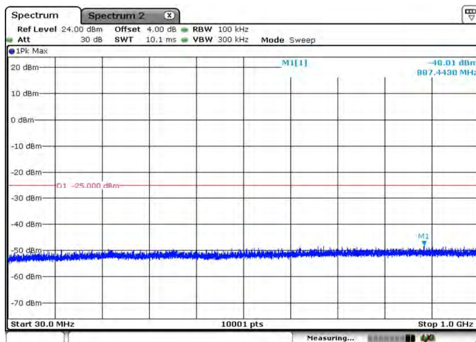
B7_CH20775_5M_1RB12_QPSK_Below 1G
