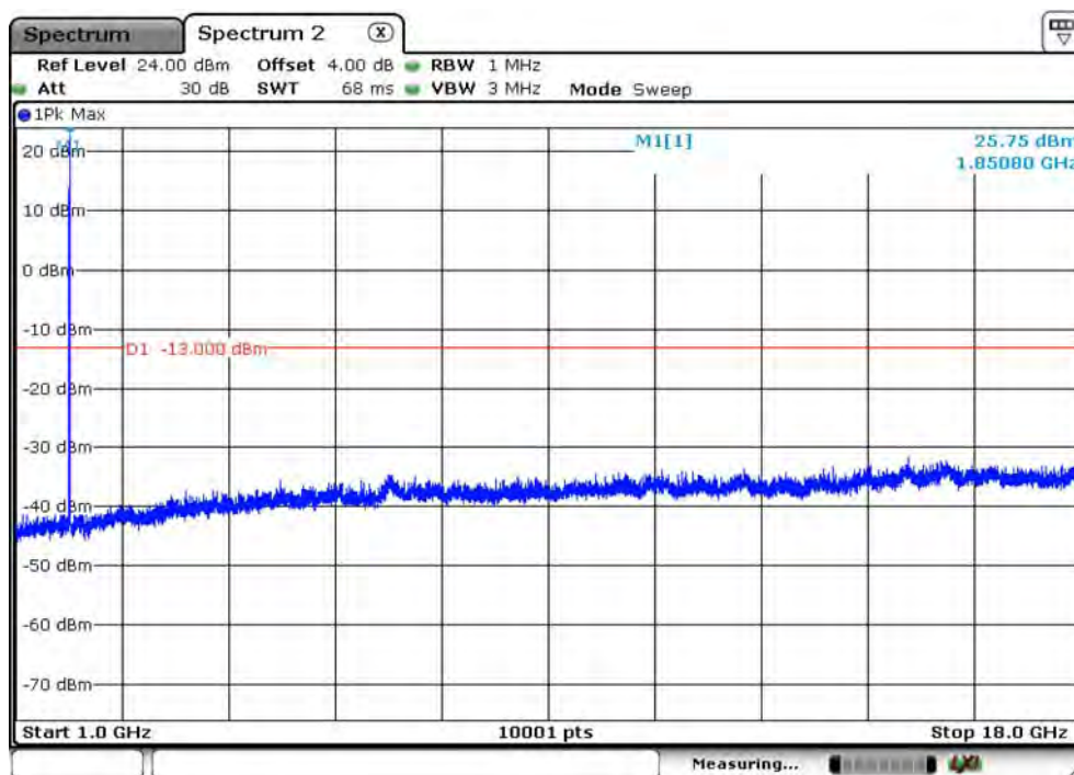
B25_CH26047_1.4M_1RB2__QPSK_Above 1G
