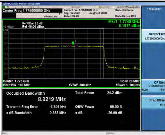
Band66-10MHz-QPSK-132622-50RB#0
