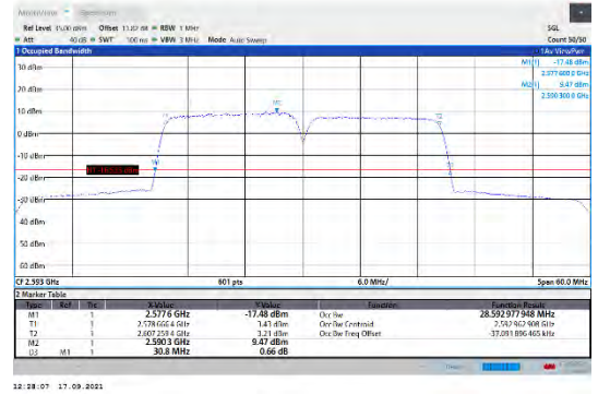
CA_41C-15MHz-15MHz-16QAM-16QAM-40545-40695-75RB#0-75RB#0
