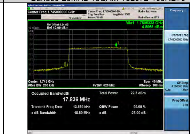
Band66-20MHz-16QAM-132322-100RB#0
