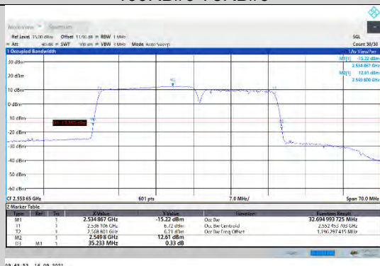
CA_7C-20MHz-15MHz-QPSK-QPSK-21201-21372-100RB#0-75RB#0
