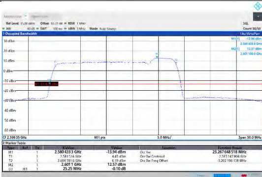
CA_41C-20MHz-5MHz-QPSK-QPSK-40595-40712-100RB#0-25RB#0
