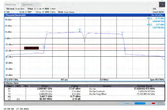
CA_41C-20MHz-20MHz-QPSK-QPSK-41292-41490-100RB#0-100RB#0
