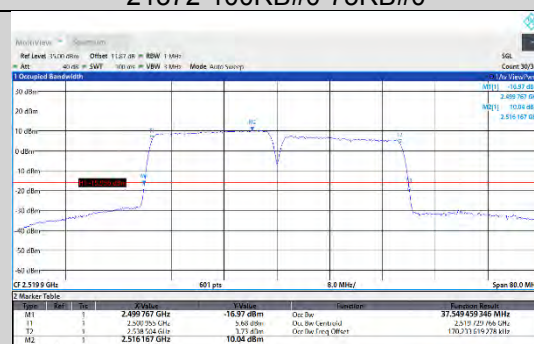
CA_7C-20MHz-15MHz-16QAM-16QAM-21201-21372-100RB#0-75RB#0
