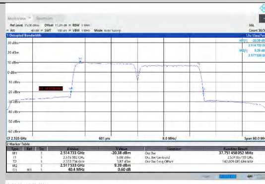
CA_7C-20MHz-20MHz-QPSK-QPSK-21001-21199-100RB#0-100RB#0
