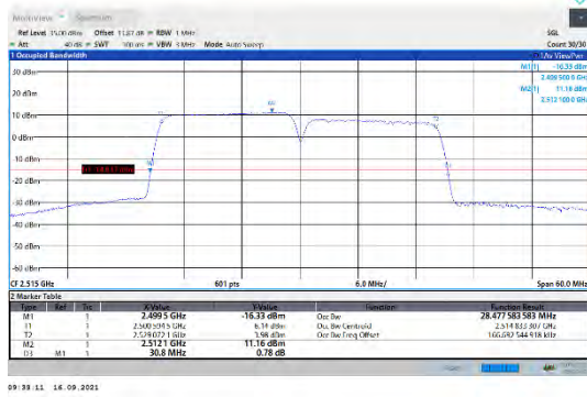
CA_7C-15MHz-15MHz-QPSK-QPSK-20825-20975-75RB#0-75RB#0
