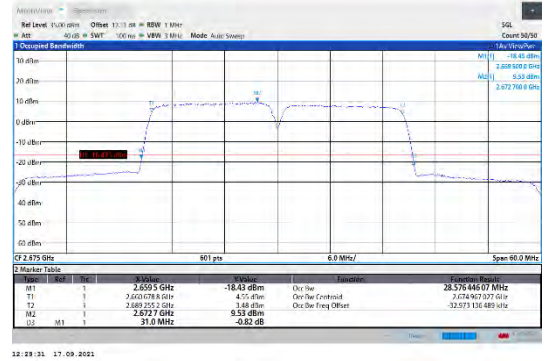
CA_41C-15MHz-15MHz-16QAM-16QAM-41365-41515-75RB#0-75RB#0
