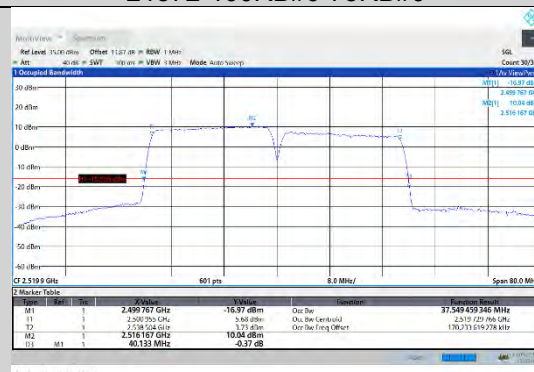
CA_7C-20MHz-20MHz-QPSK-QPSK-20850-21048-100RB#0-100RB#0
