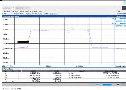
CA_41C-20MHz-10MHz-16QAM-16QAM-39750-39894-100RB#0-50RB#0
