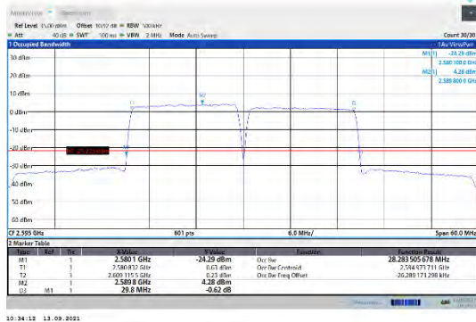
CA_38C-15MHz-15MHz-16QAM-16QAM-37925-38075-75#0-75#0
