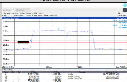
CA_7C-20MHz-15MHz-QPSK-QPSK-21201-21372-100RB#0-75RB#0
