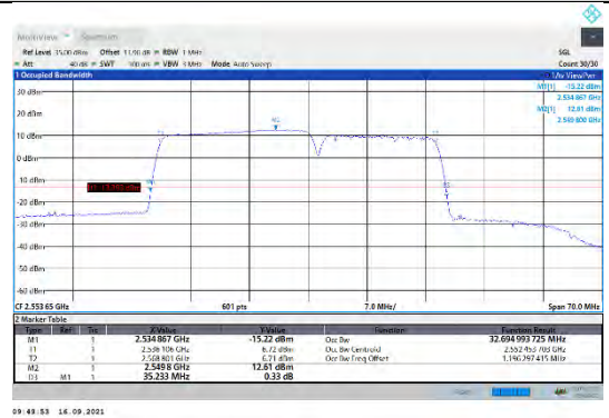
CA_7C-20MHz-15MHz-QPSK-QPSK-21201-21372-100RB#0-75RB#0
