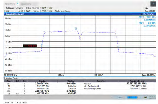
CA_38C-20MHz-20MHz-QPSK-QPSK-37850-38048-100RB#0-100RB#0
