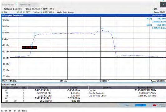
CA_41C-20MHz-5MHz-QPSK-QPSK-39750-39867-100RB#0-25RB#0
