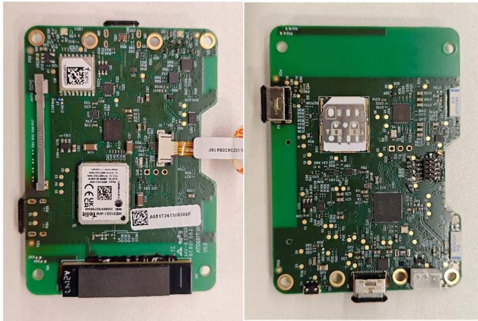
Figure 5: PCBA board
