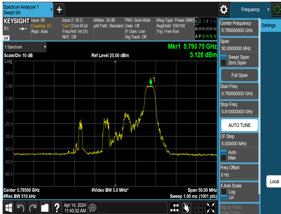
Plot 7-138. Power Spectral Density Plot MIMO ANT2 (20MHz BW 802.11be – 26 Tones (UNII Band 3) – Ch. 157)
