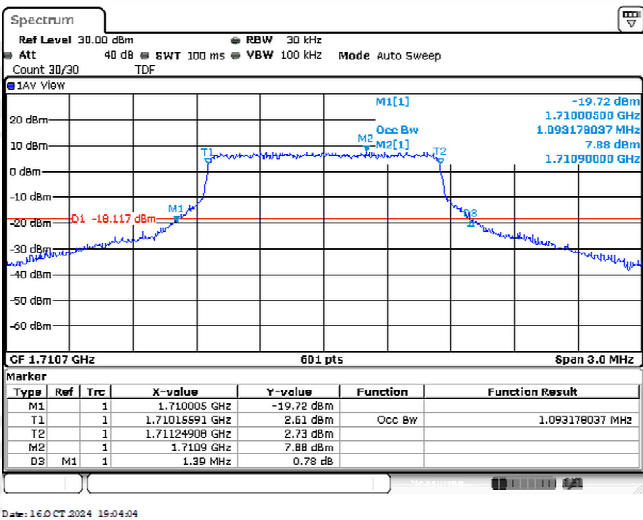
Band4-1.4MHz-16QAM-19957-6RB#0-1.093
