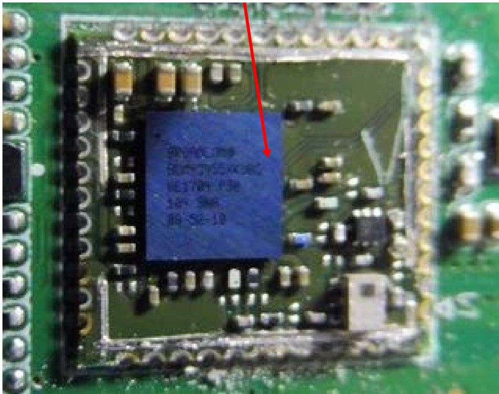
Wi-Fi and BT Module (Chip)
