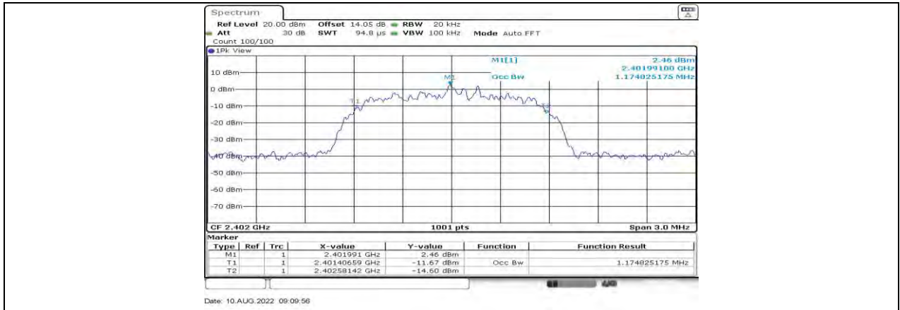
2DH5_Ant1_2402
