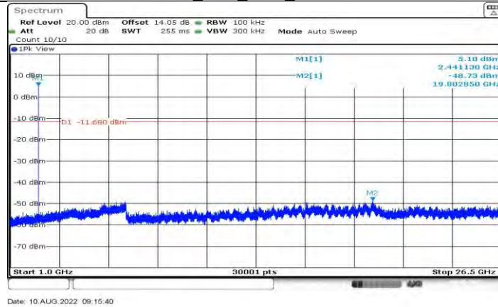
2DH5_Ant1_2441_1000~26500
