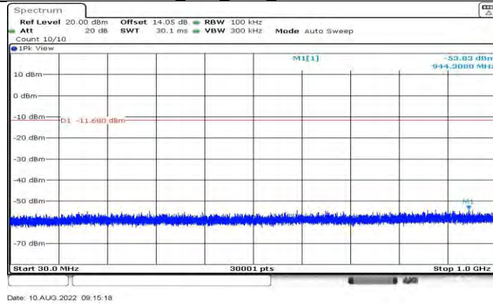
2DH5_Ant1_2441_30~1000
