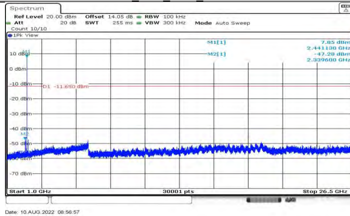
DH5_Ant1_2441_1000~26500
