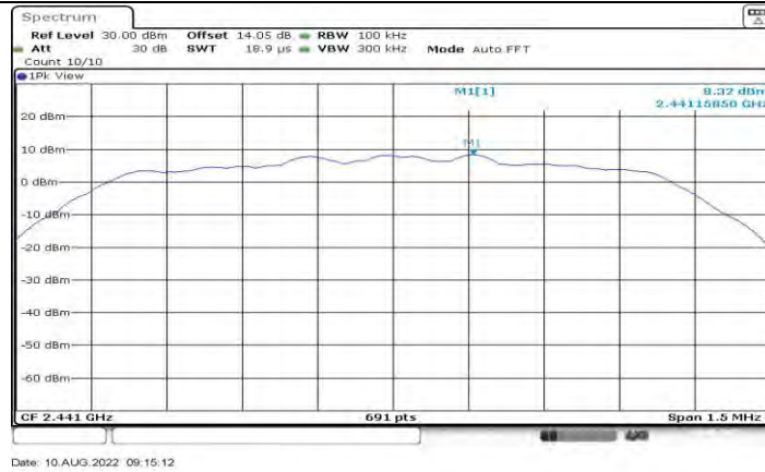
2DH5_Ant1_2441_0~Reference
