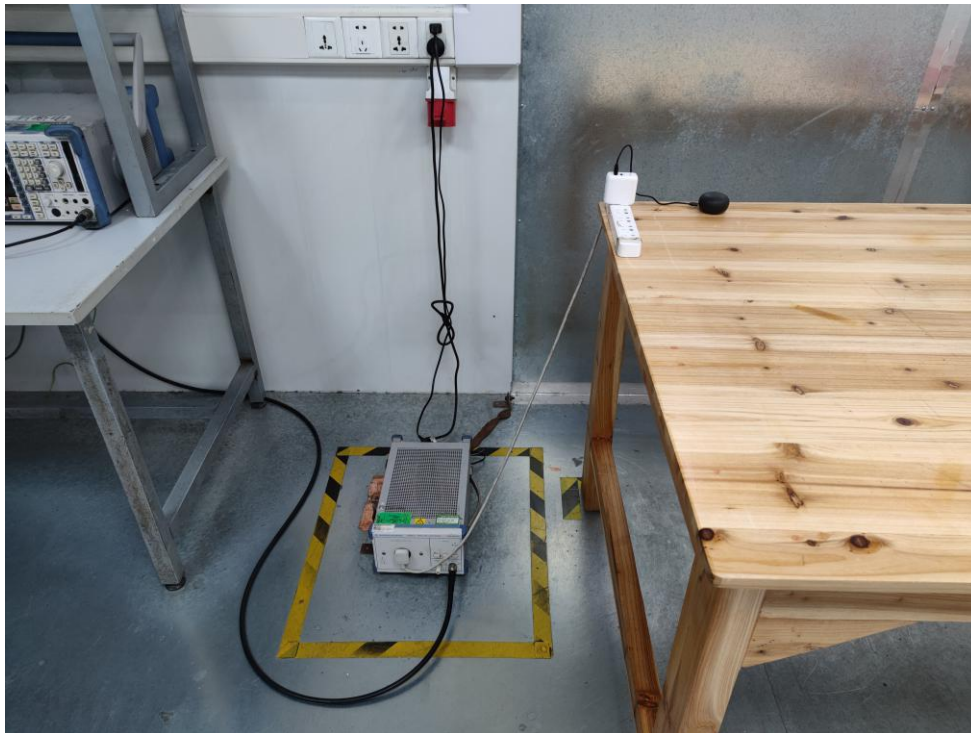
FCC ID: 2AIIIF-09347PG Photo of Power Line Conducted Emission Test
