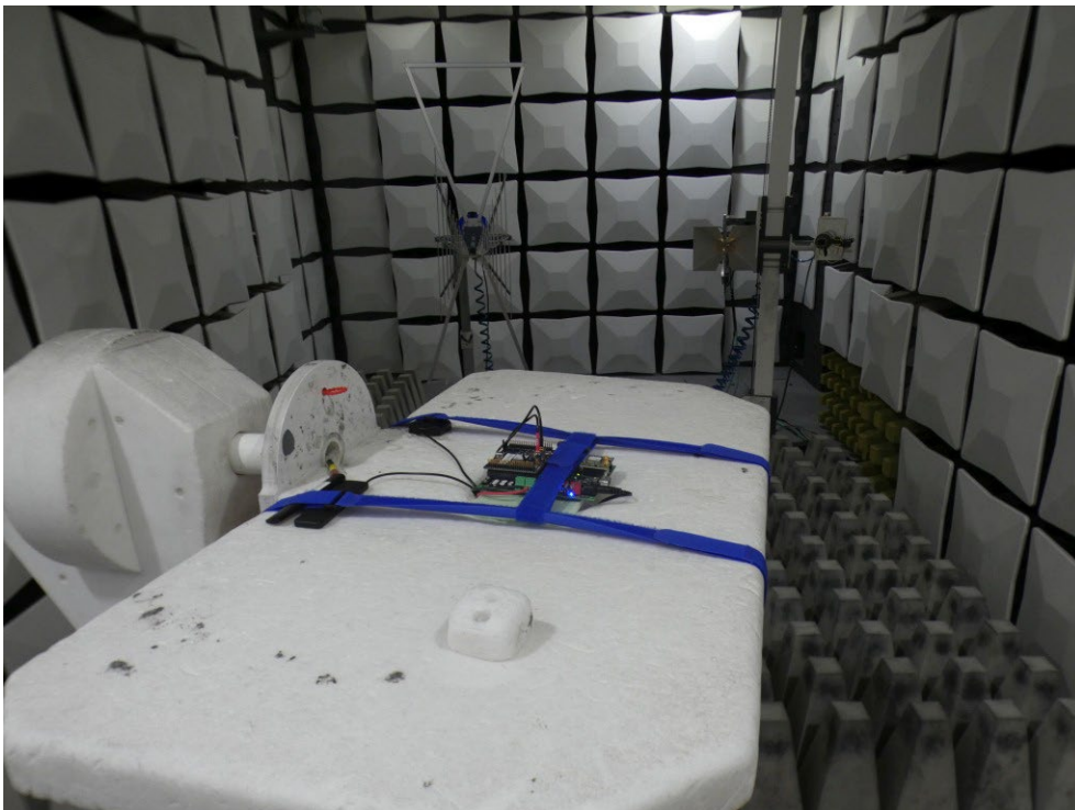
Photo 3: Antenna setup for radiated measurements above 1GHz
