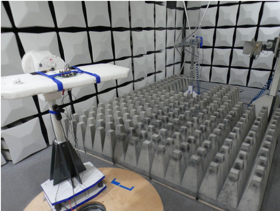
Photo 1: Test setup for radiated measurements above 1GHz
