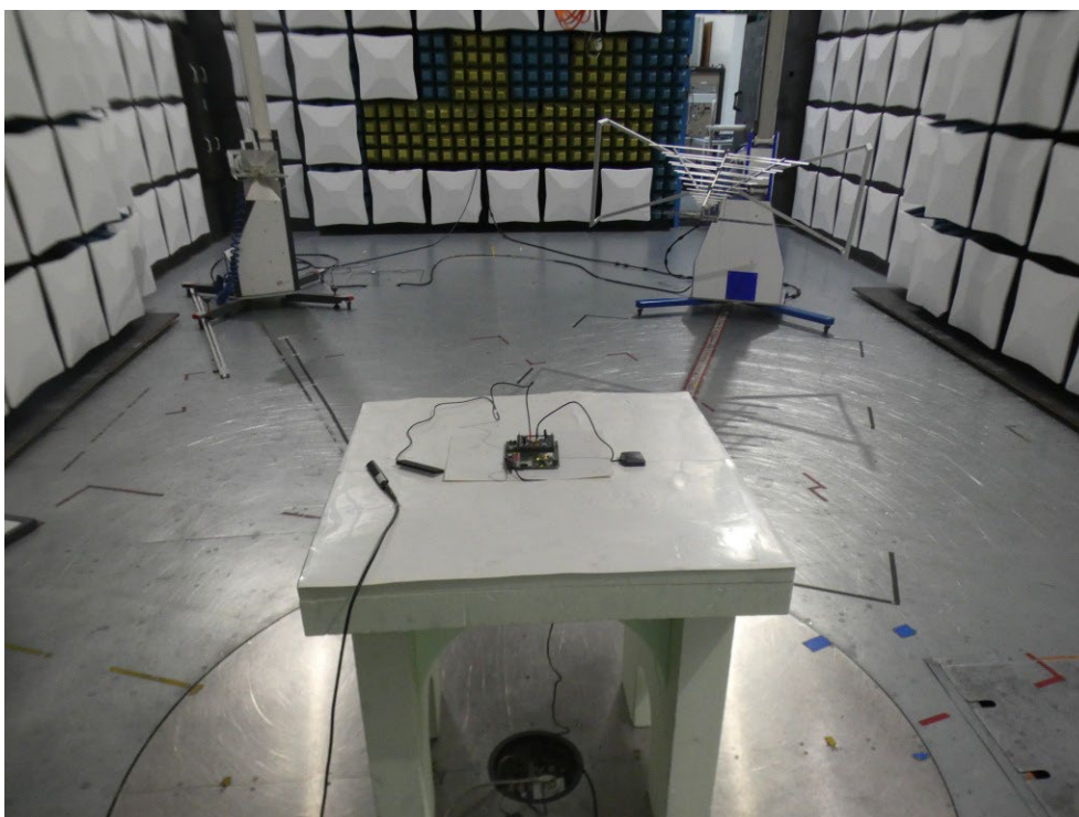
Photo 6: Antenna setup for radiated measurements below 1GHz
