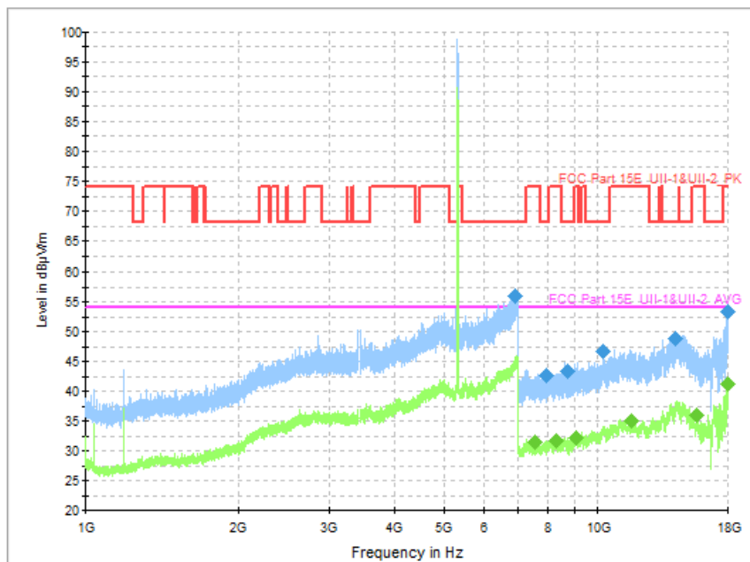
Fig. 70 Transmitter Spurious Emission (802.11a, CH64 5320MHz)
