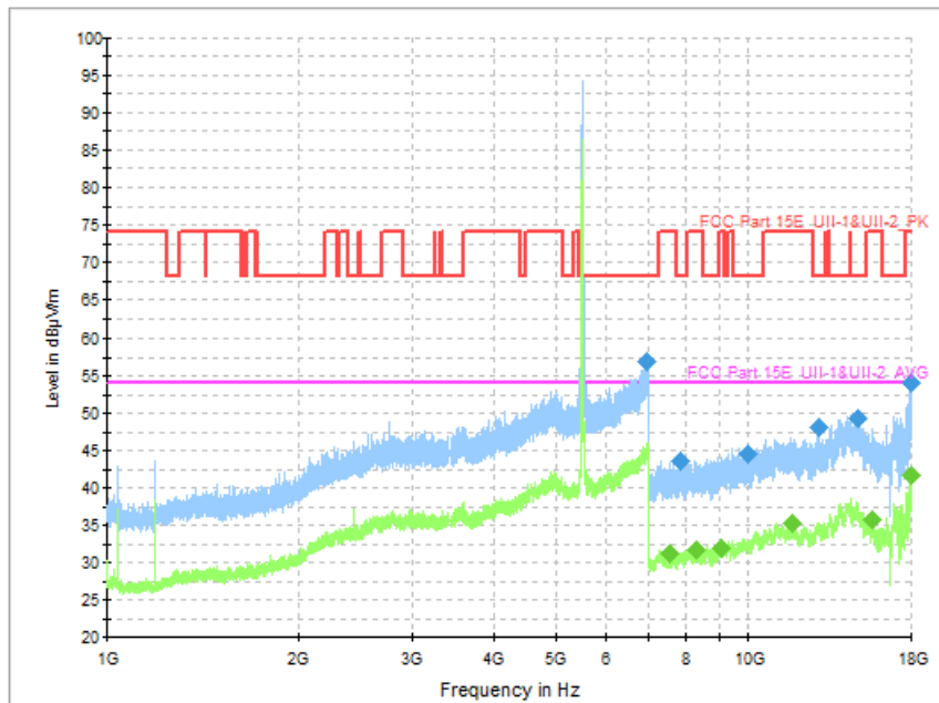
Fig. 81 Transmitter Spurious Emission (802.11n-HT40, CH102 5510MHz)
