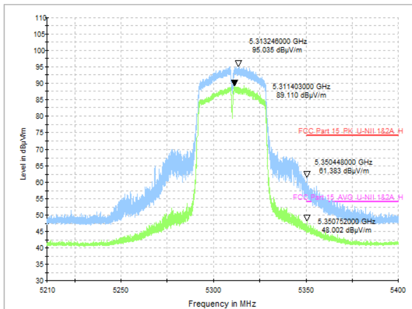
Fig. 56 Band Edges (802.11n-HT40, CH62 5310MHz)
