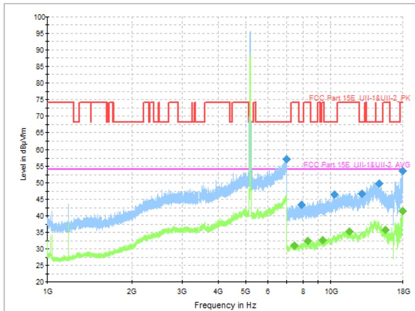
Fig. 77 Transmitter Spurious Emission (802.11n-HT40, CH38 5190MHz)
