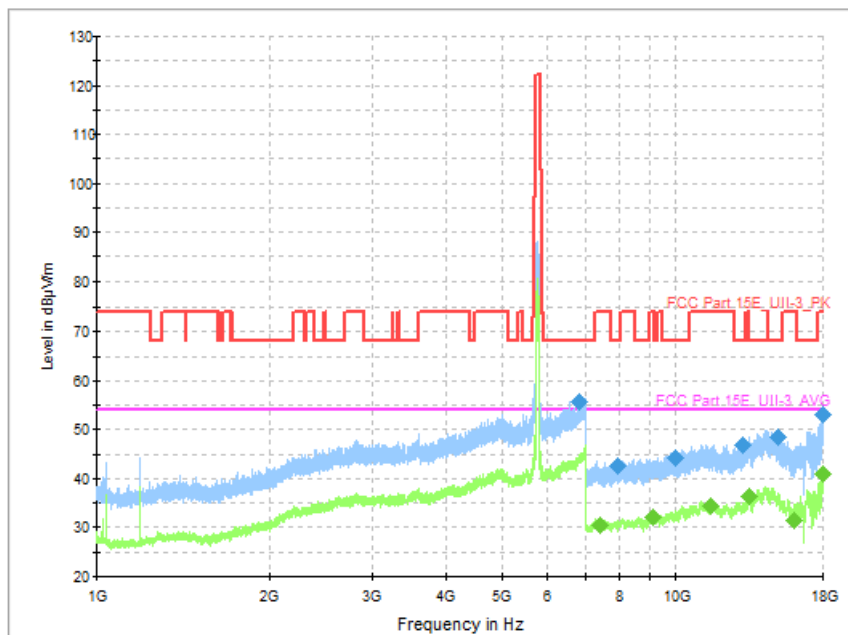
Fig. 88 Transmitter Spurious Emission (802. 11ac-VHT80, CH155 5775MHz)
