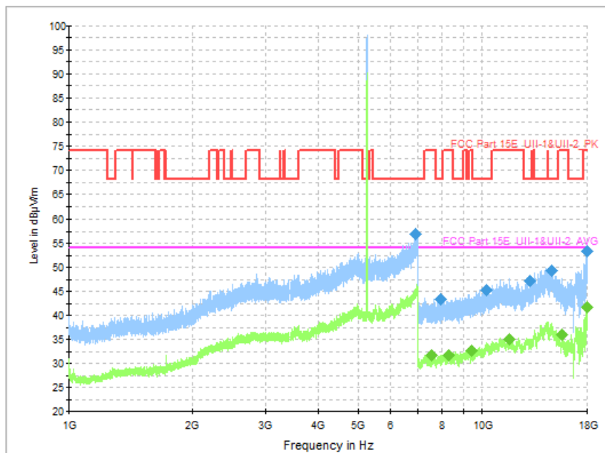
Fig. 68 Transmitter Spurious Emission (802.11a, CH52 5260MHz)
