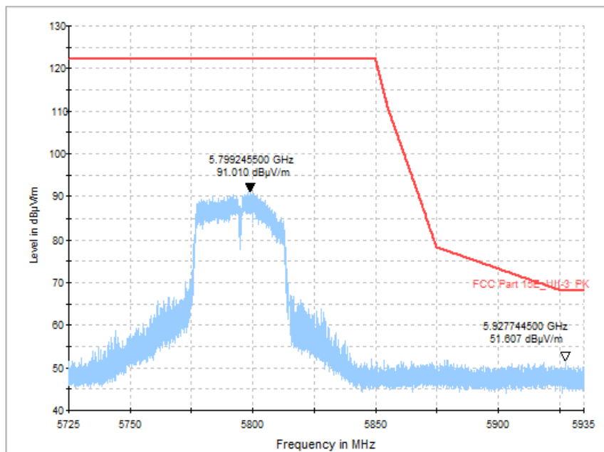
Fig. 60 Band Edges (802.11n-HT40, CH159 5795MHz)
