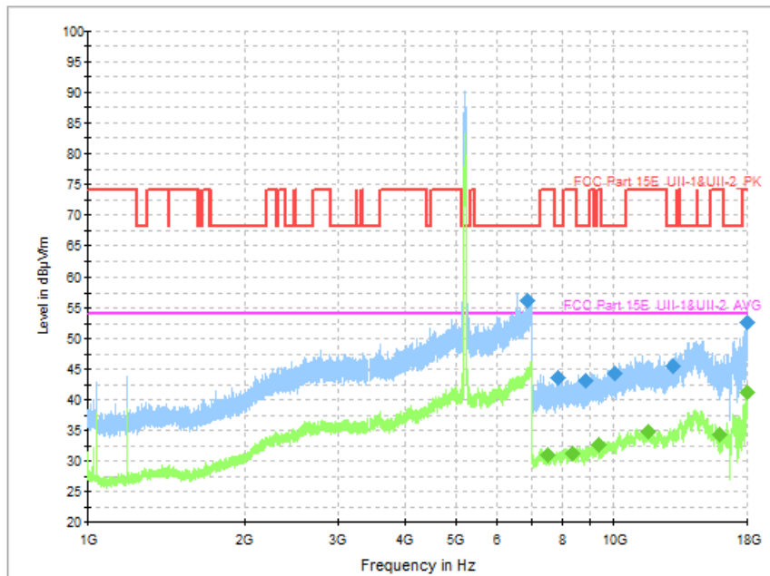
Fig. 85 Transmitter Spurious Emission (802. 11ac-VHT80, CH42 5210MHz)
