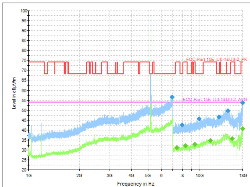
Fig. 66 Transmitter Spurious Emission (802.11a, CH40 5200MHz)
