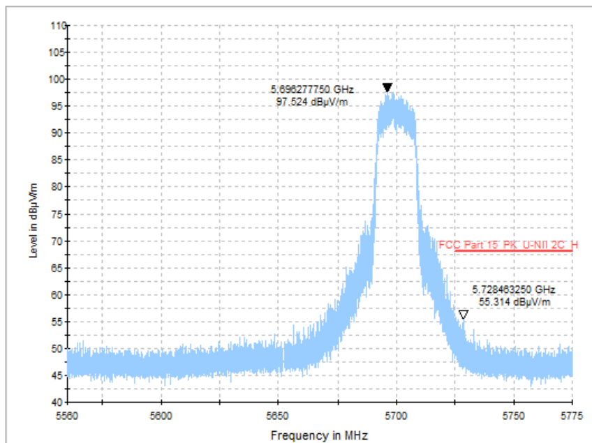
Fig. 52 Band Edges (802.11a, CH140 5700MHz)
