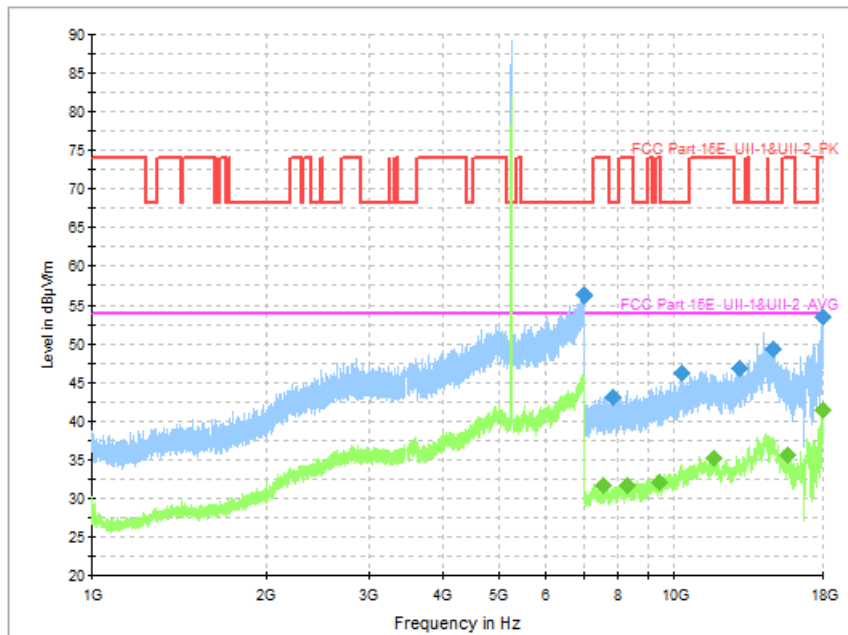
Fig. 67 Transmitter Spurious Emission (802.11a, CH48 5240MHz)
