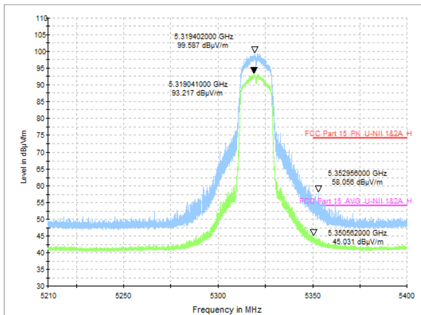
Fig. 50 Band Edges (802.11a, CH64 5320MHz)
