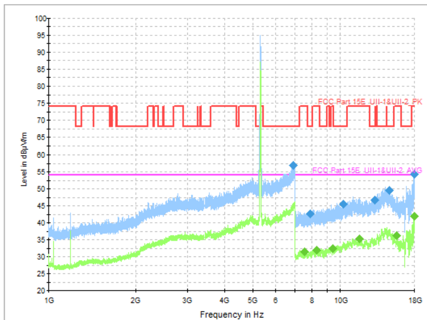
Fig. 80 Transmitter Spurious Emission (802.11n-HT40, CH62 5310MHz)
