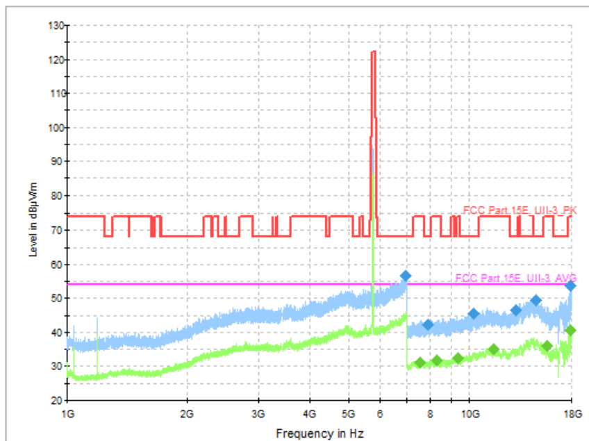
Fig. 74 Transmitter Spurious Emission (802. 11a, CH149 5745MHz)
