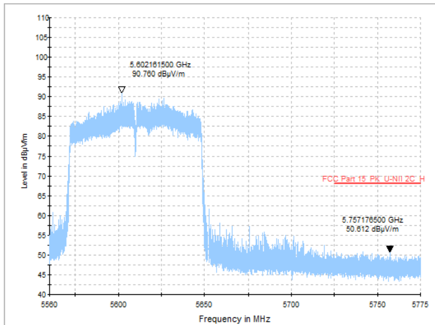
Fig. 63 Band Edges (802.11ac-VHT80, CH122 5610MHz)
