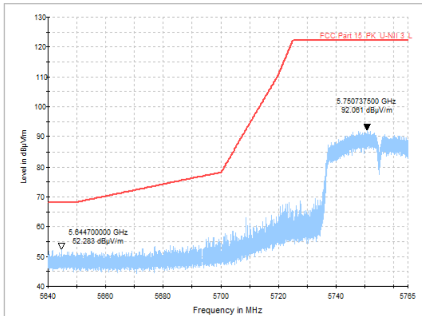
Fig. 59 Band Edges (802.11n-HT40, CH151 5755MHz)
