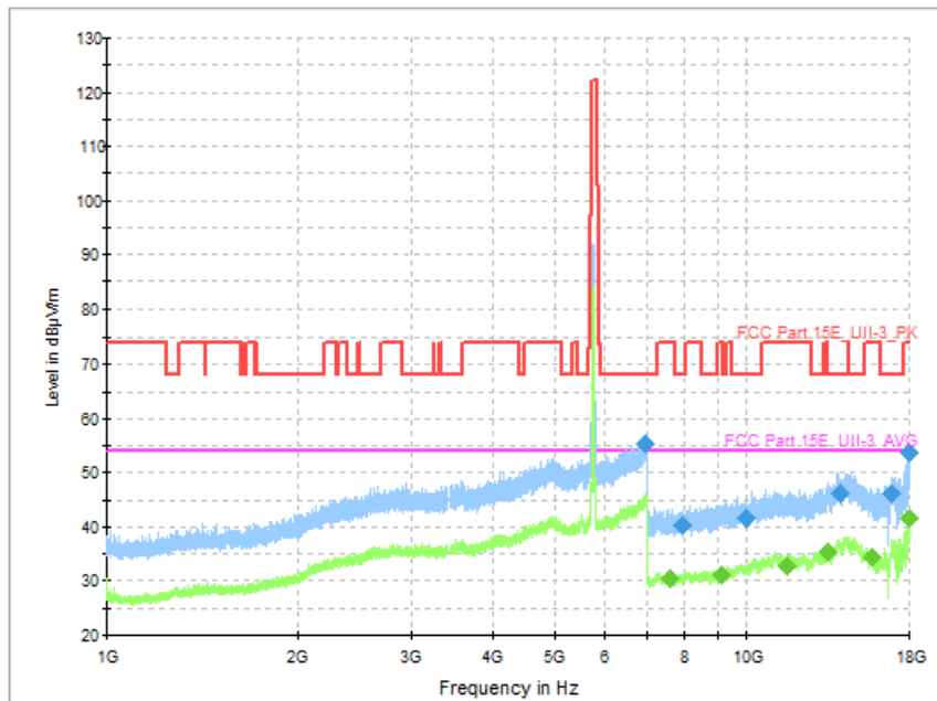
Fig. 83 Transmitter Spurious Emission (802. 11ac-VHT40, CH151 5755MHz)
