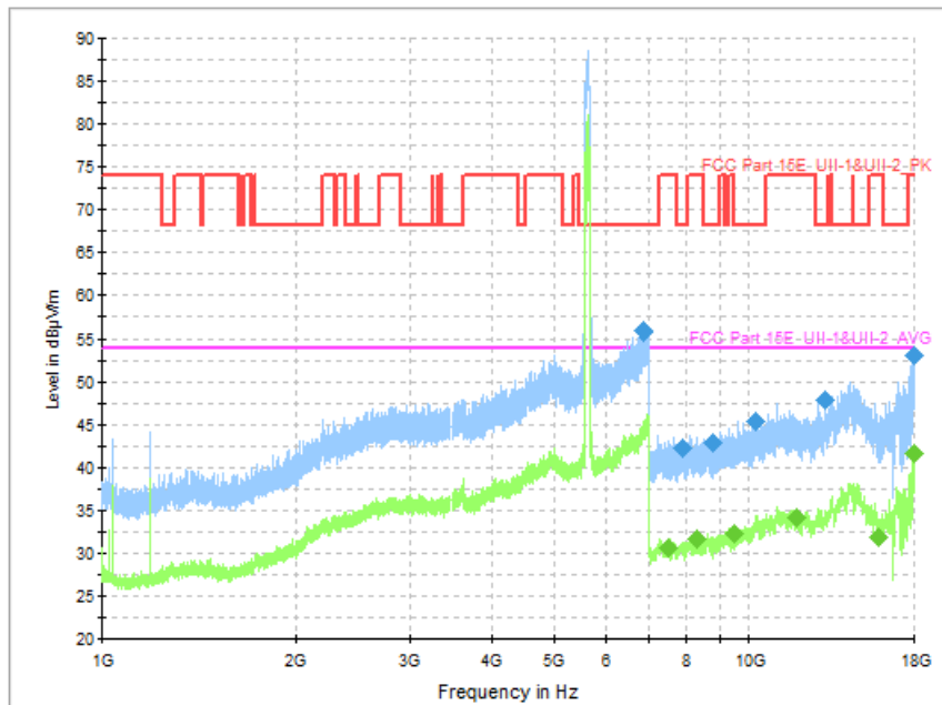
Fig. 87 Transmitter Spurious Emission (802. 11ac-VHT80, CH122 5610MHz)
