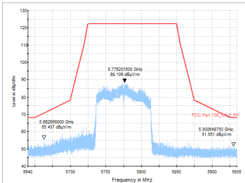
Fig. 64 Band Edges (802.11ac-VHT80, CH155 5775MHz)
