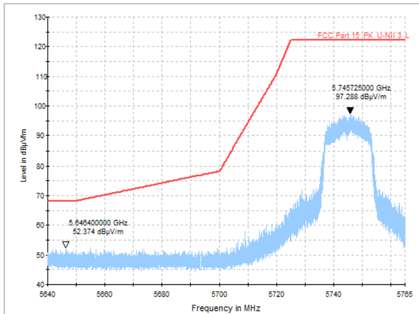
Fig. 53 Band Edges (802.11a, CH149 5745MHz)
