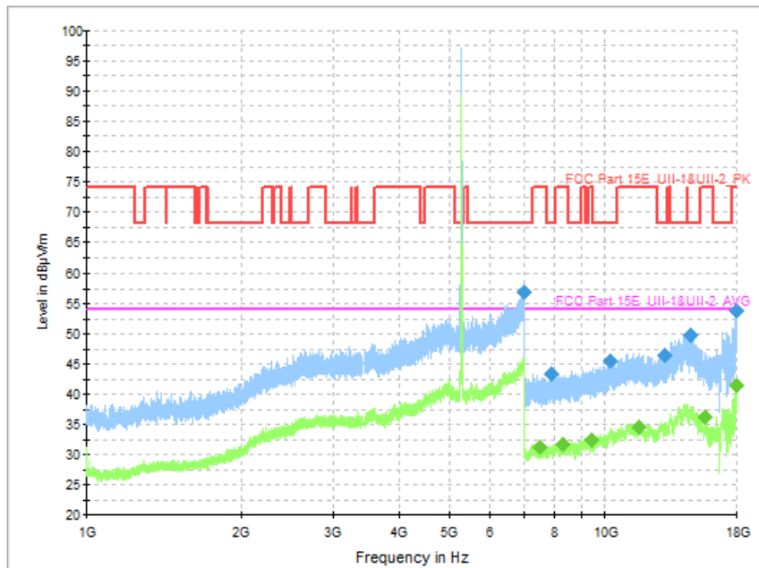
Fig. 69 Transmitter Spurious Emission (802.11a, CH56 5280MHz)
