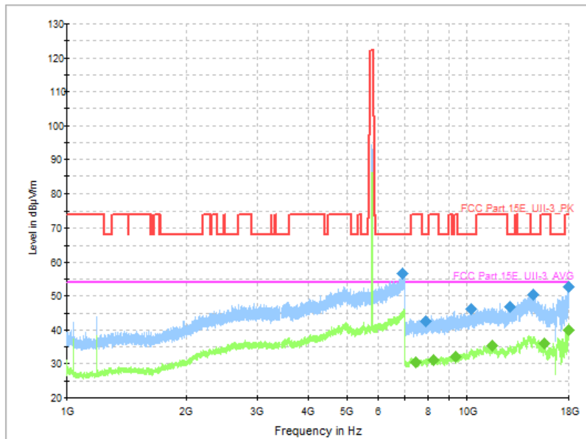
Fig. 75 Transmitter Spurious Emission (802. 11a, CH157 5785MHz)
