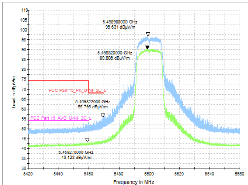
Fig. 51 Band Edges (802.11a, CH100 5500MHz)
