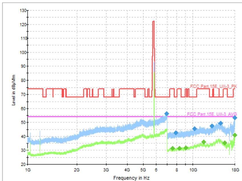
Fig. 76 Transmitter Spurious Emission (802. 11a, CH165 5825MHz)
