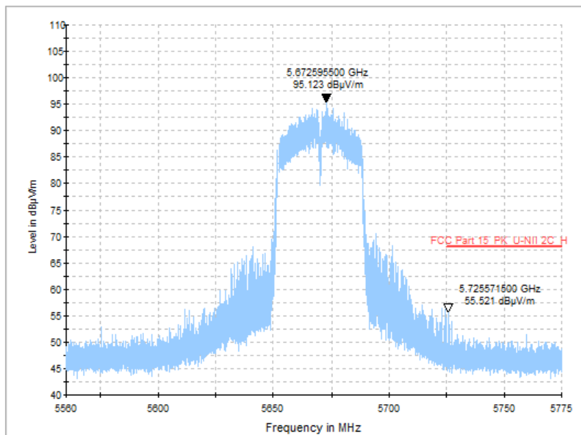
Fig. 58 Band Edges (802.11n-HT40, CH134 5670MHz)
