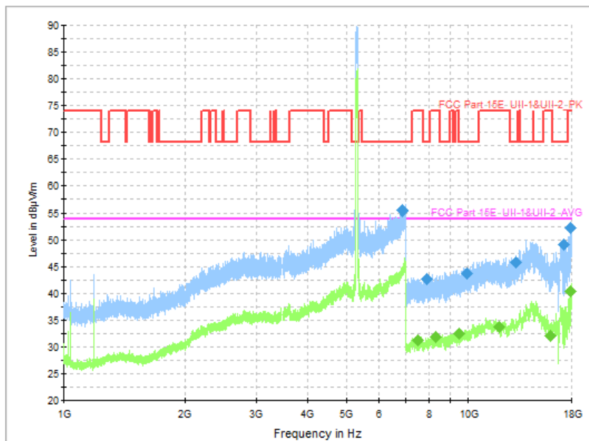
Fig. 86 Transmitter Spurious Emission (802. 11ac-VHT80, CH58 5290MHz)
