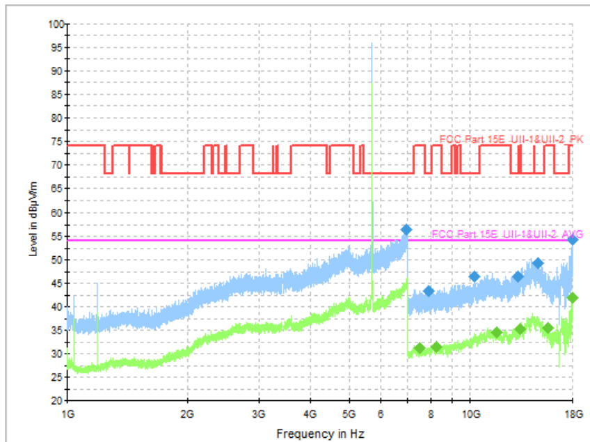
Fig. 73 Transmitter Spurious Emission (802.11a, CH140 5700MHz)
