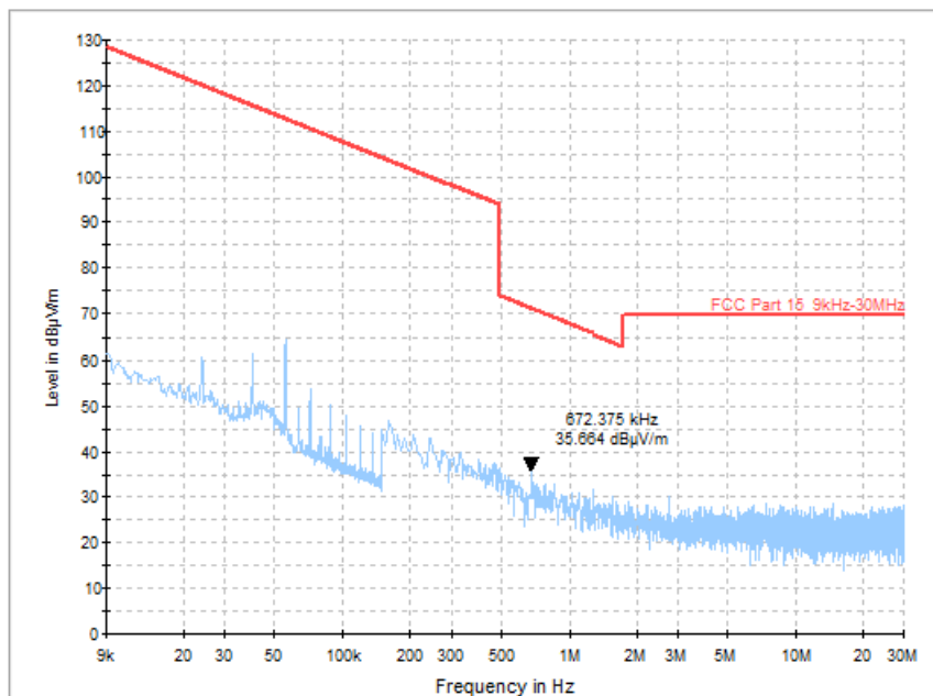
Fig. 92 Radiated Spurious Emission (All Channel, 9kHz ~ 30MHz)
