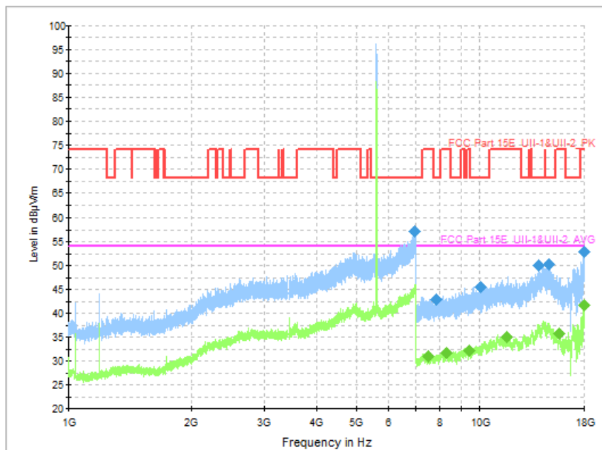
Fig. 72 Transmitter Spurious Emission (802.11a, CH116 5580MHz)
