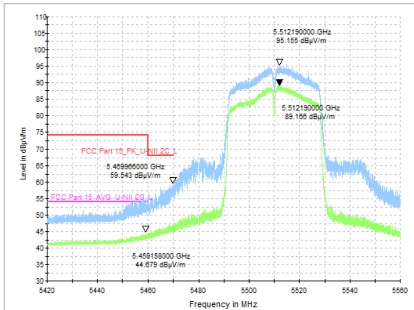
Fig. 57 Band Edges (802.11n-HT40, CH102 5510MHz)
