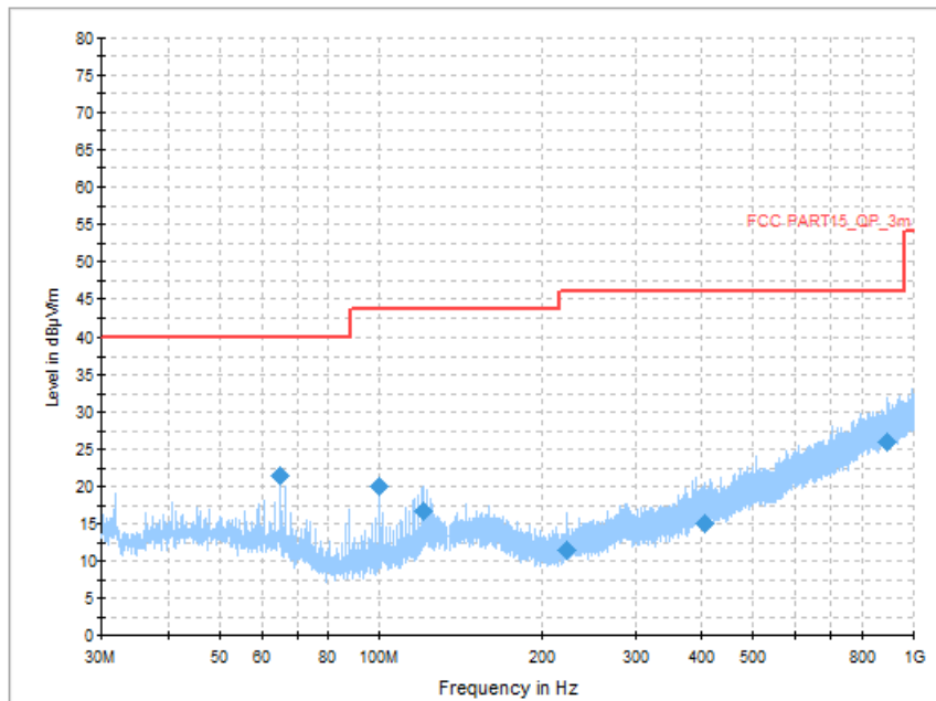
Fig. 89 Transmitter Spurious Emission (All channel, 30MHz~1GHz)
