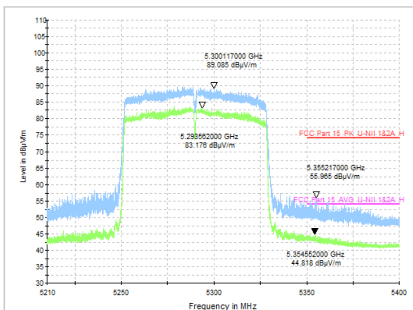
Fig. 62 Band Edges (802.11ac-VHT80, CH58 5290MHz)
