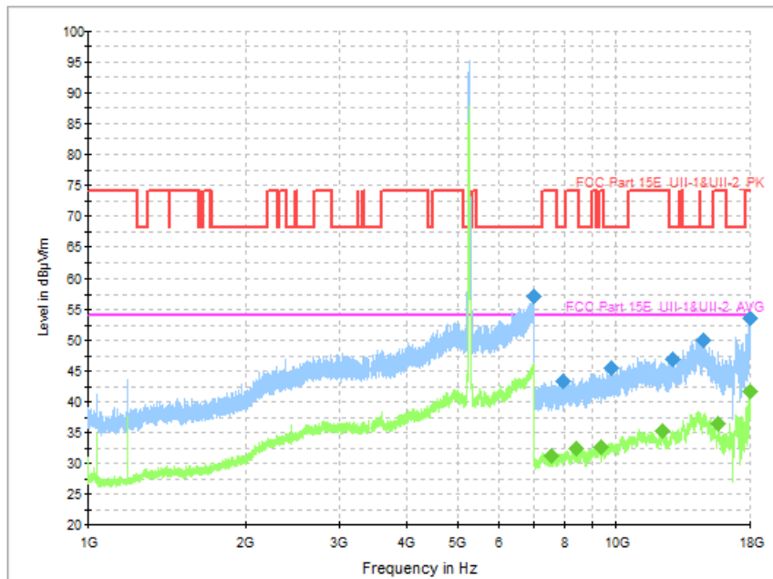
Fig. 79 Transmitter Spurious Emission (802.11n-HT40, CH54 5270MHz)
