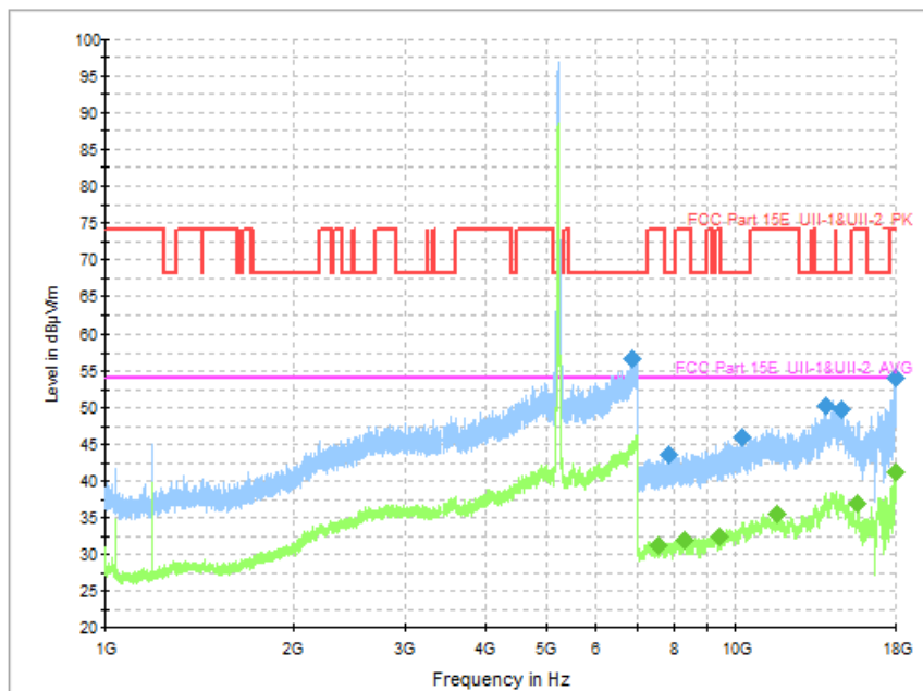
Fig. 78 Transmitter Spurious Emission (802.11n-HT40, CH46 5230MHz)
