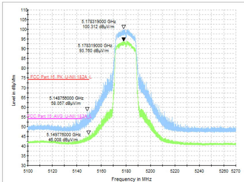
Fig. 49 Band Edges (802.11a, CH36 5180MHz)
