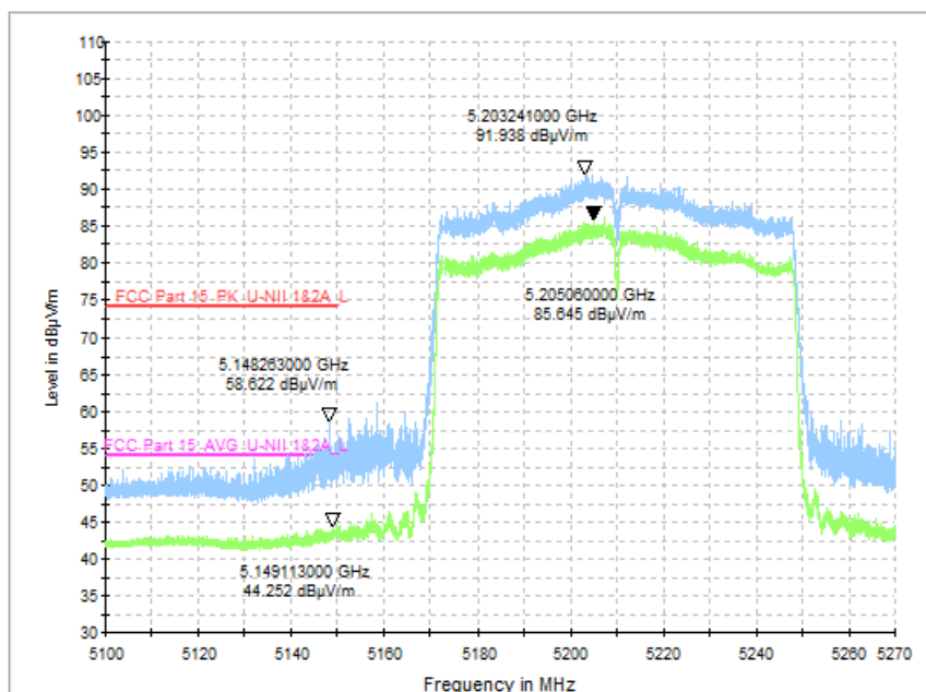
Fig. 61 Band Edges (802.11ac-VHT80, CH42 5210MHz)
