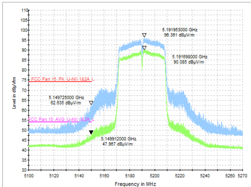
Fig. 55 Band Edges (802.11n-HT40, CH38 5190MHz)
