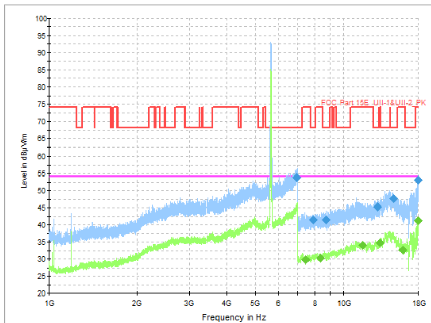
Fig. 82 Transmitter Spurious Emission (802.11n-HT40, CH134 5670MHz)
