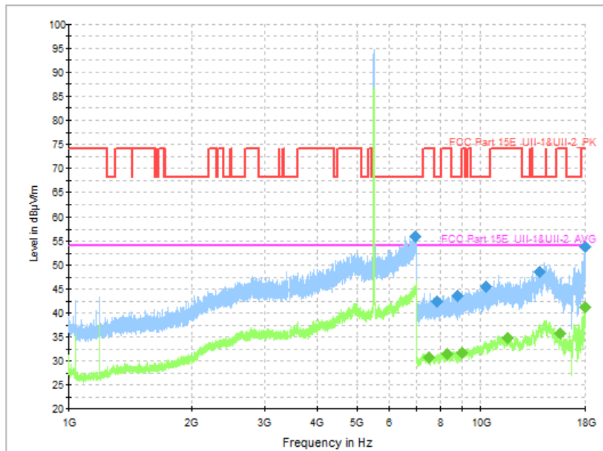
Fig. 71 Transmitter Spurious Emission (802.11a, CH100 5500MHz)
