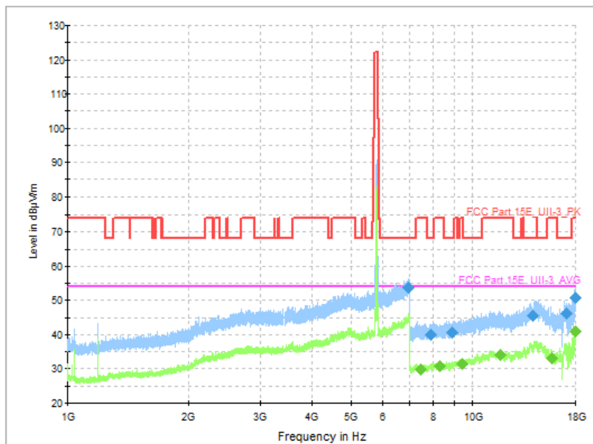
Fig. 84 Transmitter Spurious Emission (802. 11ac-VHT40, CH159 5795MHz)
