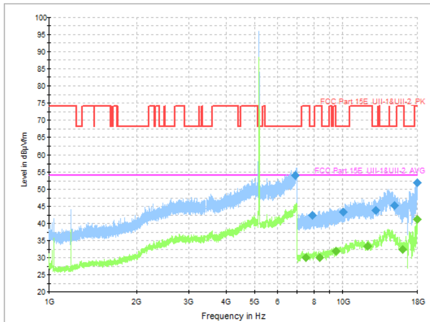
Fig. 65 Transmitter Spurious Emission (802.11a, CH36 5180MHz)
