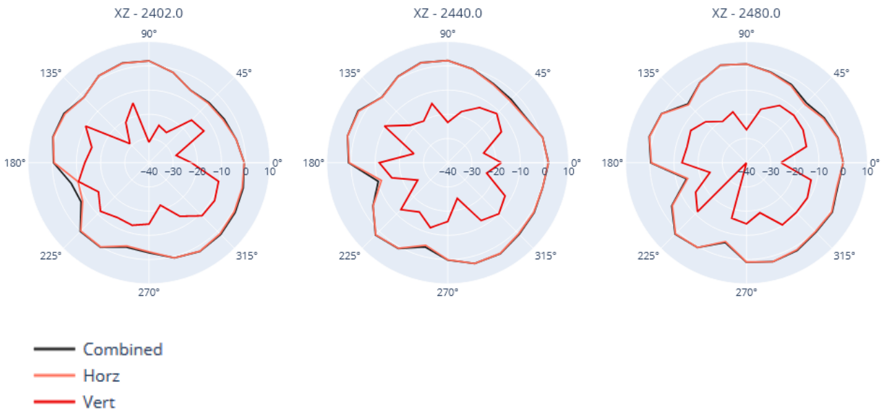
Figure 2 - Gain X-Z
