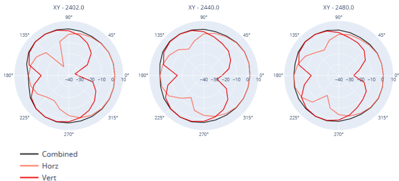
Figure 1 – Gain X-Y
