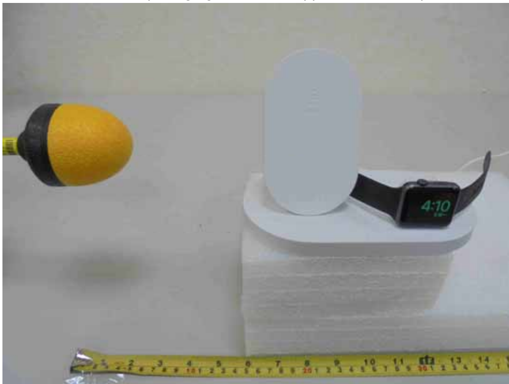
E-Field (Charging Mode with Apple Watch - Left)
