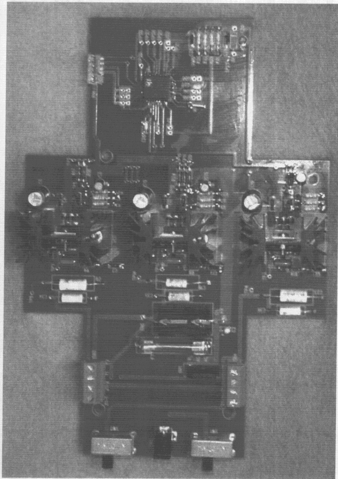
Photo 7. EUT, Main Board, Component Side
