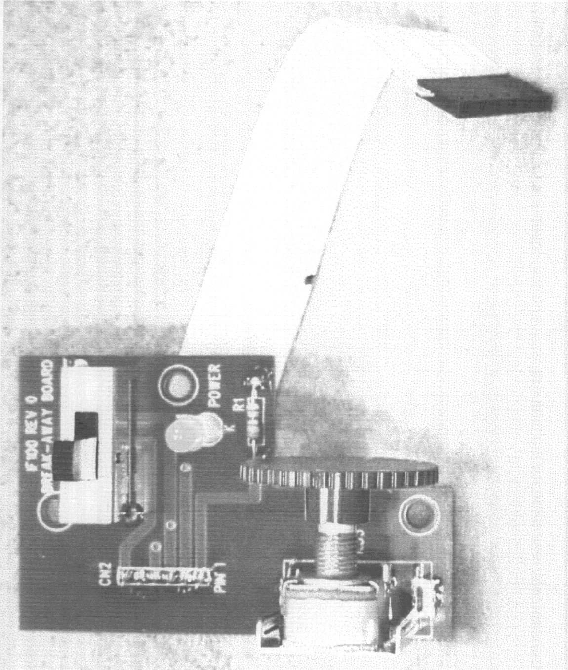
Photo 3. Break Away Board, Component Side
