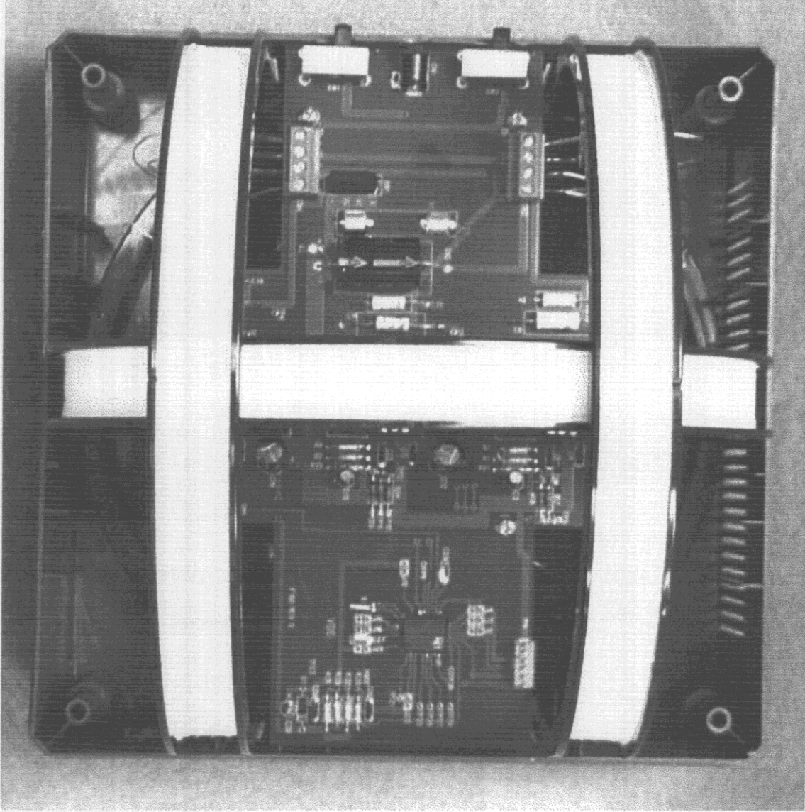
Photo 6. EUT, Front View, Rear Cover
