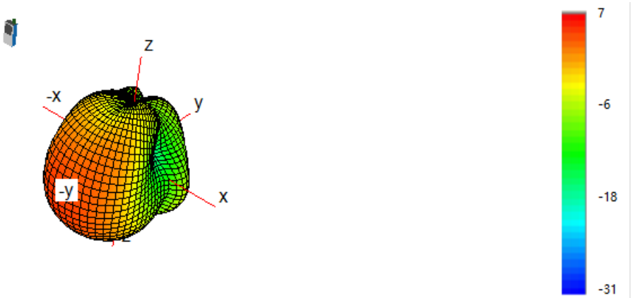
3D Antenna pattern
