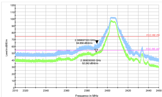
802.11ax HE40-Channel 3 Peak &amp; Average
