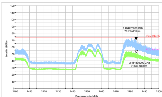
802.11g-Channel 9 Peak &amp; Average
