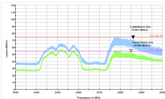
802.11n HT20-Channel 9 Peak &amp; Average
