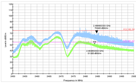
802.11g-Channel 11 Peak &amp; Average
