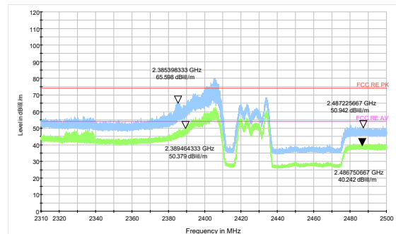
802.11g-Channel 4 Peak &amp; Average
