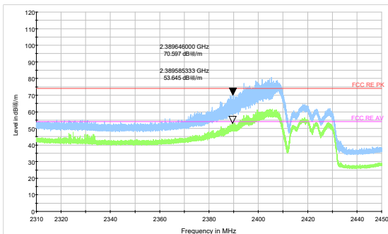
802.11n HT20-Channel 3 Peak &amp; Average
