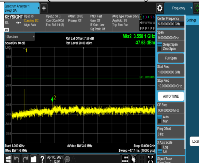
Band66-1.4MHz-QPSK-132665-1RB#0-Range2:1000~10000MHz
