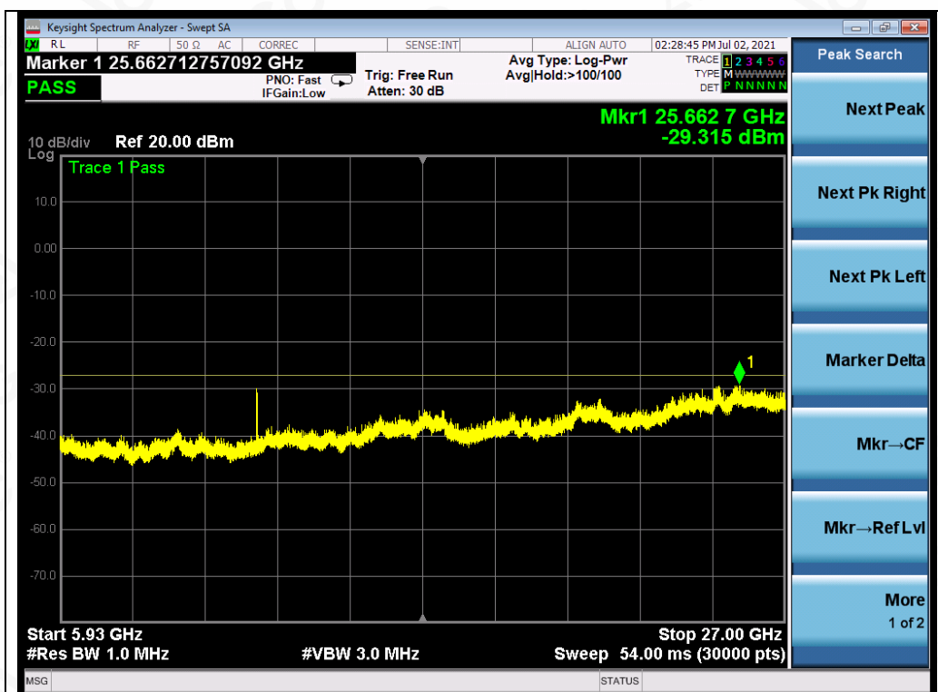
Test_Graph_802.11n20_ANT1_5825_MCS0_Frequency Band4
