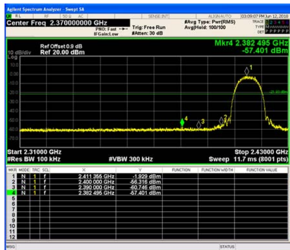
Left bandedge
