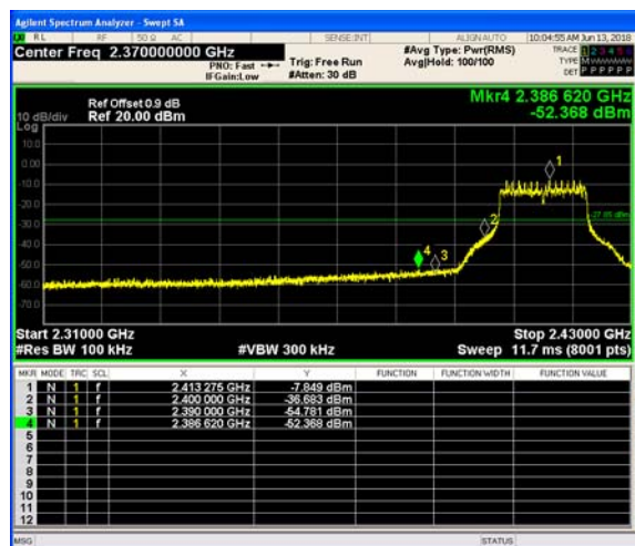
Left bandedge
