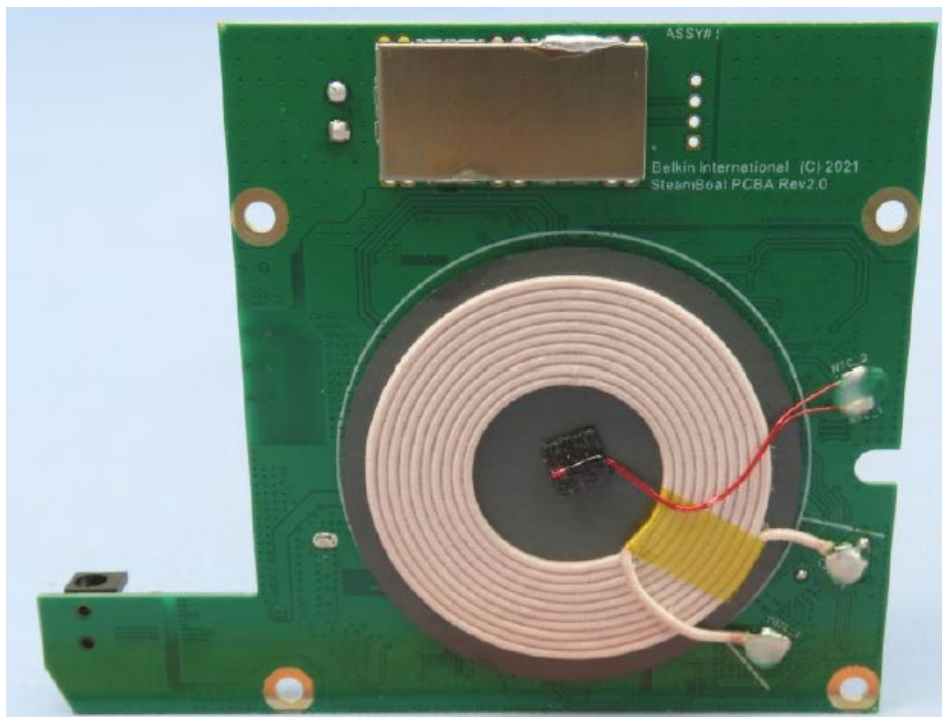
Center Coil Antenna for AirPods (110.5 kHz to 148.5 kHz) – Bottom View
