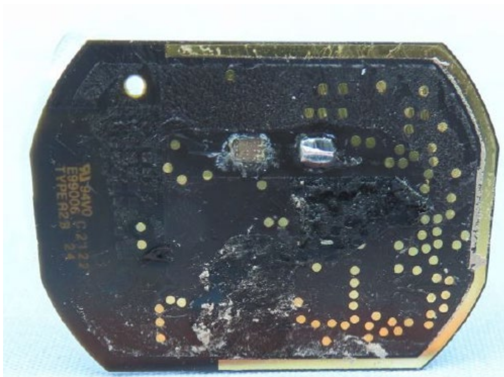
C222 PCB (MagSafe iPhones – 360 kHz) – Bottom View
