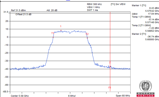
802.11a_Chain 3 / CH116
