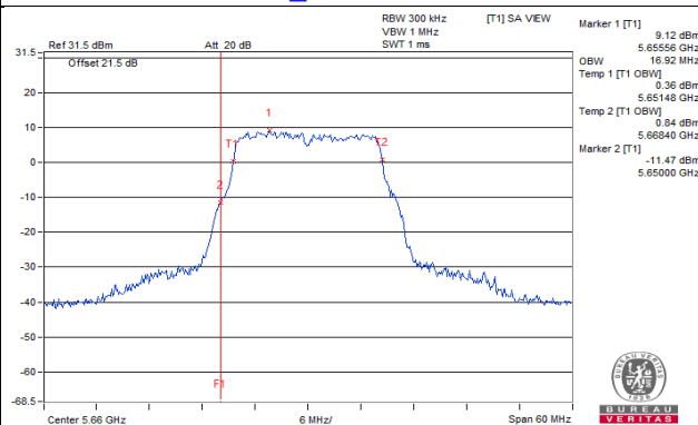
802.11a_Chain 3 / CH132
