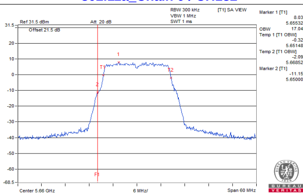
802.11a_Chain 2 / CH132
