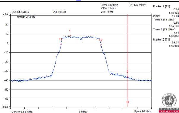
802.11a_Chain 2 / CH116
