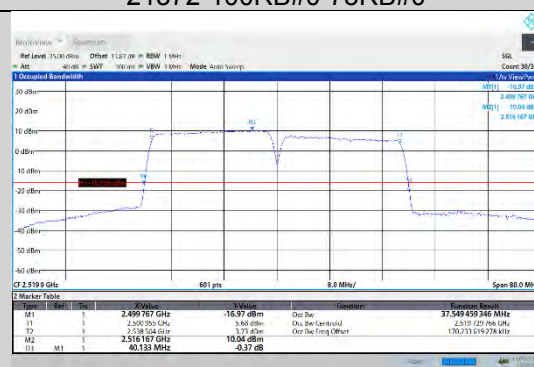
CA_7C-20MHz-20MHz-QPSK-QPSK-20850-21048-100RB#0-100RB#0
