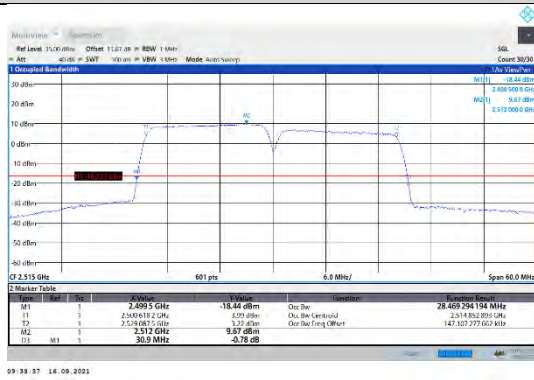
CA_7C-15MHz-15MHz-16QAM-16QAM-20825-20975-75RB#0-75RB#0
