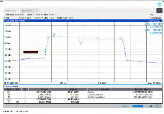
CA_7C-15MHz-20MHz-QPSK-QPSK-21003-21174-75RB#0-100RB#0
