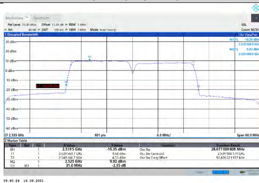
CA_7C-15MHz-15MHz-QPSK-QPSK-21025-21175-75RB#0-75RB#0
