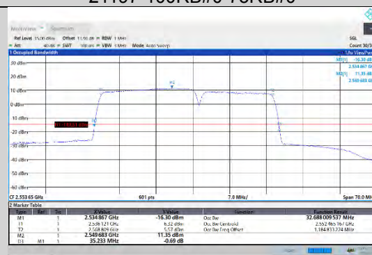
CA_7C-20MHz-15MHz-16QAM-16QAM-21201-21372-100RB#0-75RB#0
