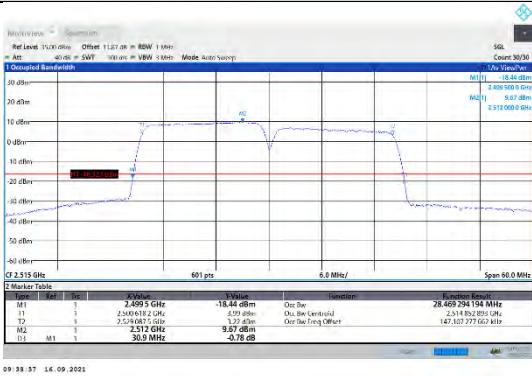
CA_7C-15MHz-15MHz-16QAM-16QAM-20825-20975-75RB#0-75RB#0
