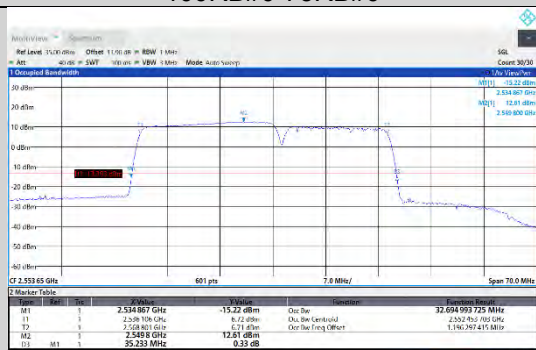
CA_7C-20MHz-15MHz-QPSK-QPSK-21026-21197-100RB#0-75RB#0
