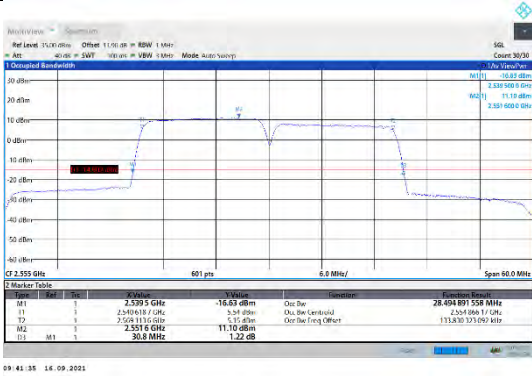
CA_7C-15MHz-15MHz-QPSK-QPSK-21225-21375-75RB#0-75RB#0
