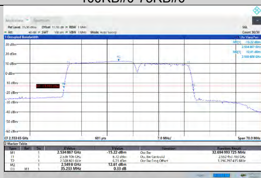
CA_7C-20MHz-15MHz-QPSK-QPSK-21201-21372-100RB#0-75RB#0
