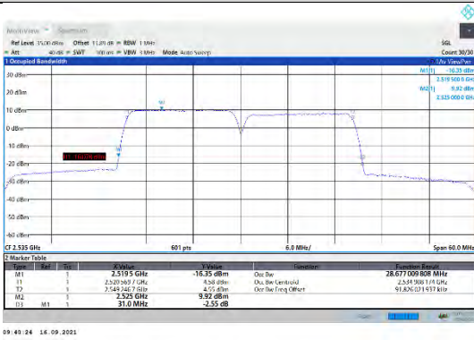
CA_7C-15MHz-15MHz-QPSK-QPSK-21025-21175-75RB#0-75RB#0
