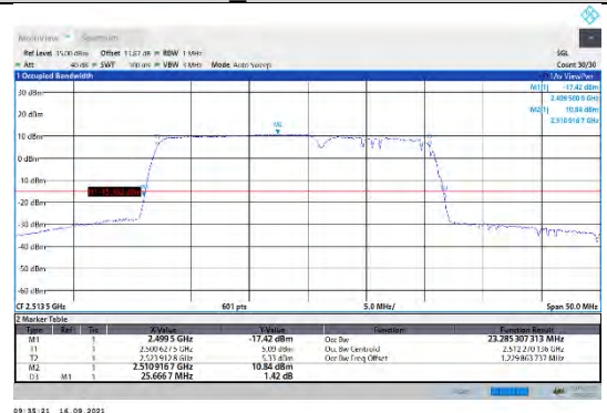
CA_7C-15MHz-10MHz-16QAM-16QAM-20825-20945-75RB#0-50RB#0
