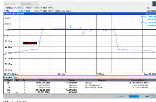
CA_7C-20MHz-15MHz-QPSK-QPSK-20850-21021-100RB#0-75RB#0
