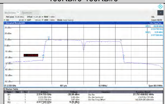
CA_7C-20MHz-20MHz-QPSK-QPSK-20850-21048-100RB#0-100RB#0
