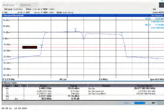
CA_7C-15MHz-15MHz-QPSK-QPSK-20825-20975-75RB#0-75RB#0
