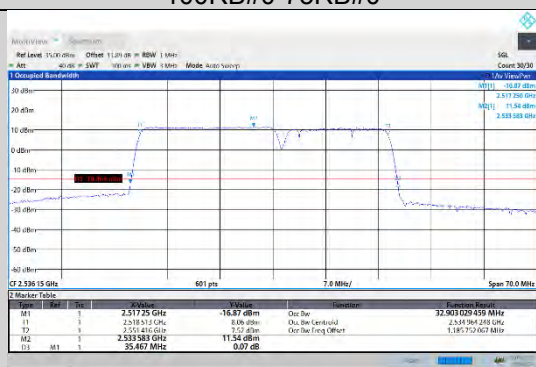
CA_7C-20MHz-15MHz-QPSK-QPSK-21026-21197-100RB#0-75RB#0
