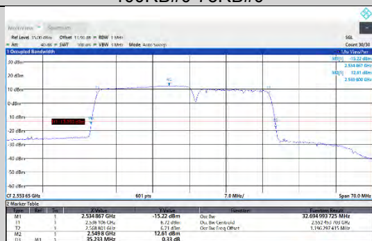
CA_7C-20MHz-15MHz-QPSK-QPSK-21026-21197-100RB#0-75RB#0
