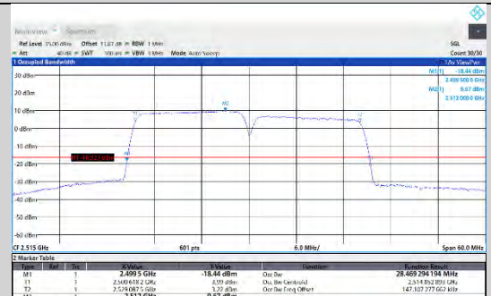
CA_7C-15MHz-15MHz-QPSK-QPSK-21225-21375-75RB#0-75RB#0
