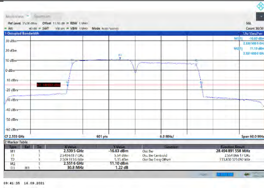
CA_7C-15MHz-15MHz-QPSK-QPSK-21225-21375-75RB#0-75RB#0
