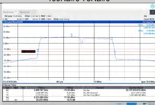
CA_7C-20MHz-15MHz-16QAM-16QAM-20850-21021-100RB#0-75RB#0
