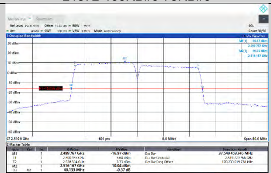
CA_7C-20MHz-15MHz-16QAM-16QAM-21201-21372-100RB#0-75RB#0
