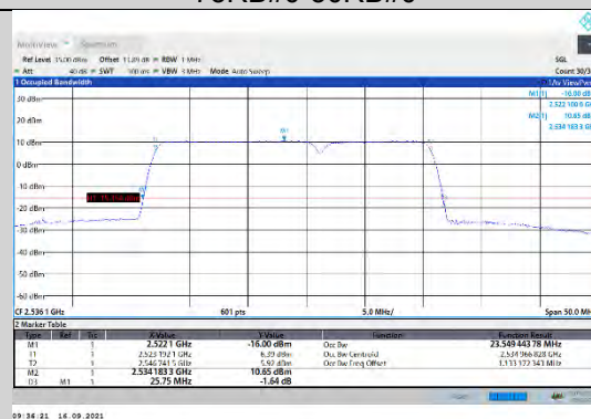
CA_7C-15MHz-10MHz-QPSK-QPSK-21051-21171-75RB#0-50RB#0
