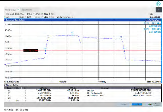
CA_7C-15MHz-20MHz-QPSK-QPSK-20828-20999-75RB#0-100RB#0
