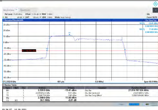
CA_7C-10MHz-20MHz-16QAM-16QAM-21206-21350-50RB#0-100RB#0
