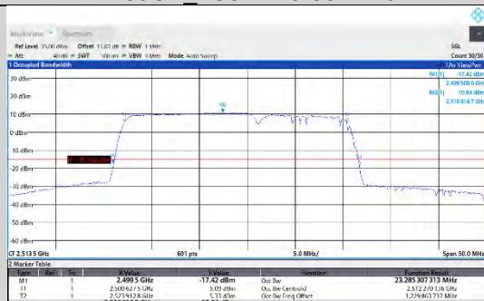
CA_7C-15MHz-10MHz-QPSK-QPSK-21277-2139CA_7C5RB#0-50RB#0
