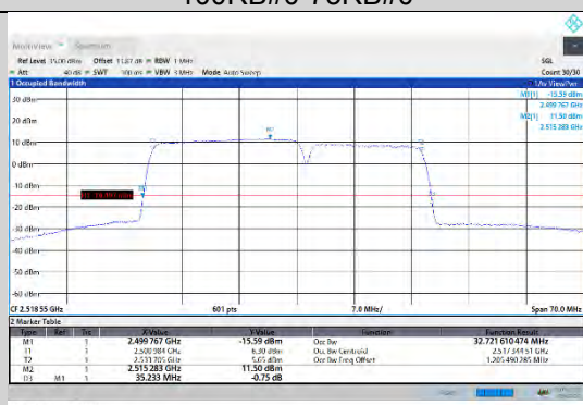
CA_7C-20MHz-15MHz-16QAM-16QAM-20850-21021-100RB#0-75RB#0
