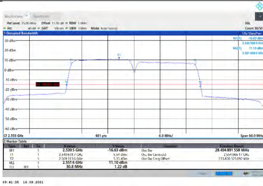
CA_7C-15MHz-15MHz-QPSK-QPSK-21225-21375-75RB#0-75RB#0
