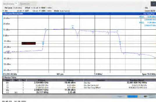
CA_7C-15MHz-20MHz-QPSK-QPSK-21179-21350-75RB#0-100RB#0
