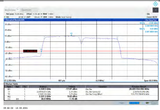
CA_7C-15MHz-15MHz-16QAM-16QAM-21225-21375-75RB#0-75RB#0
