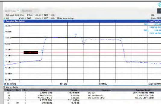
CA_7C-15MHz-15MHz-QPSK-QPSK-20825-20975-75RB#0-75RB#0
