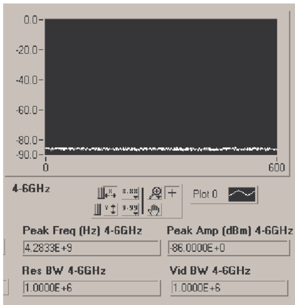
Figure 11 : Conducted Spurious Emissions - 1 Carrier, Channel 775 (4 GHz - 6 GHz)
