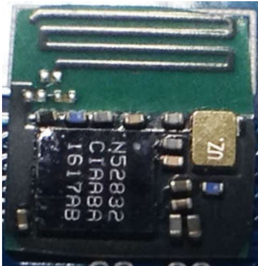
Figure 3: Internal Photo – Resin Removed
