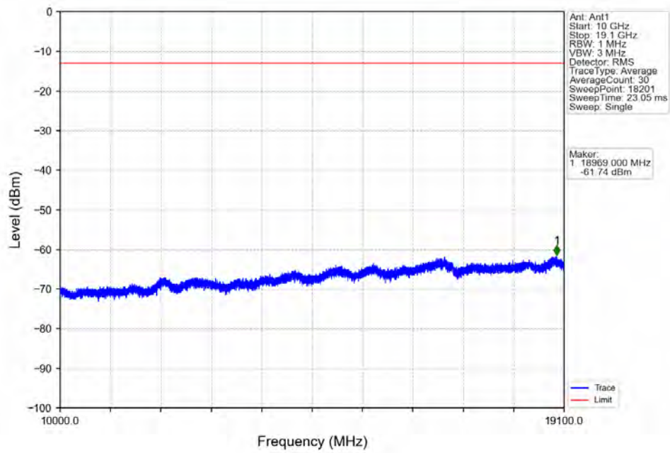
Band2_1.4MHz_16QAM_LCH_1850.7MHz_RB_1_0_NTNV
