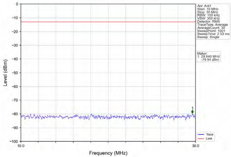
Band2_1.4MHz_16QAM_LCH_1850.7MHz_RB_1_0_NTNV
