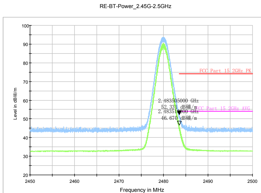
Fig.77. Radiated emission (Power): \pi/4 DQPSK, high channel
