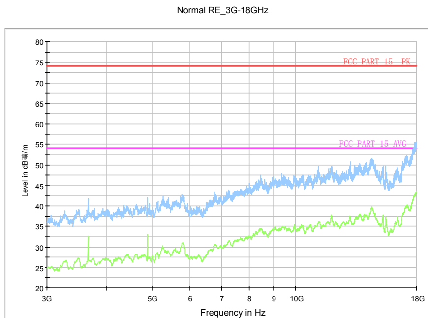
Fig.83. Radiated emission: 8DPSK, Channel 39, 3 GHz - 18 GHz
