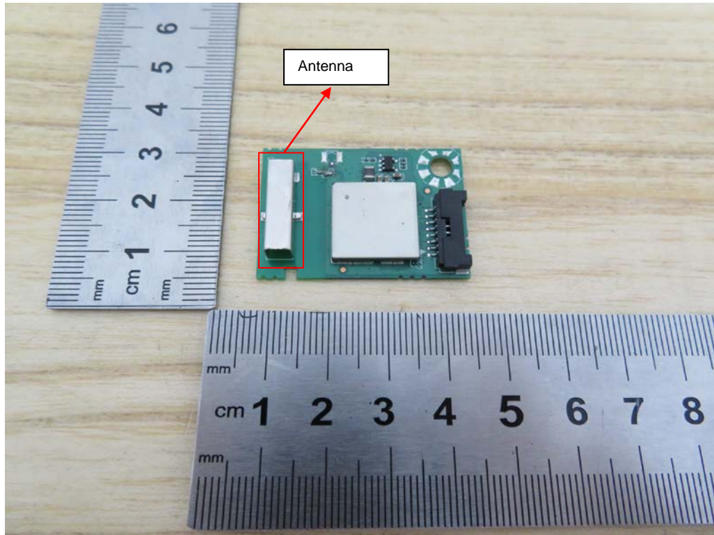
Detail View of EUT-1
