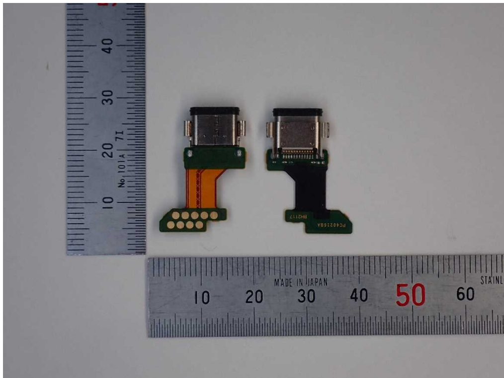
USB FPC
