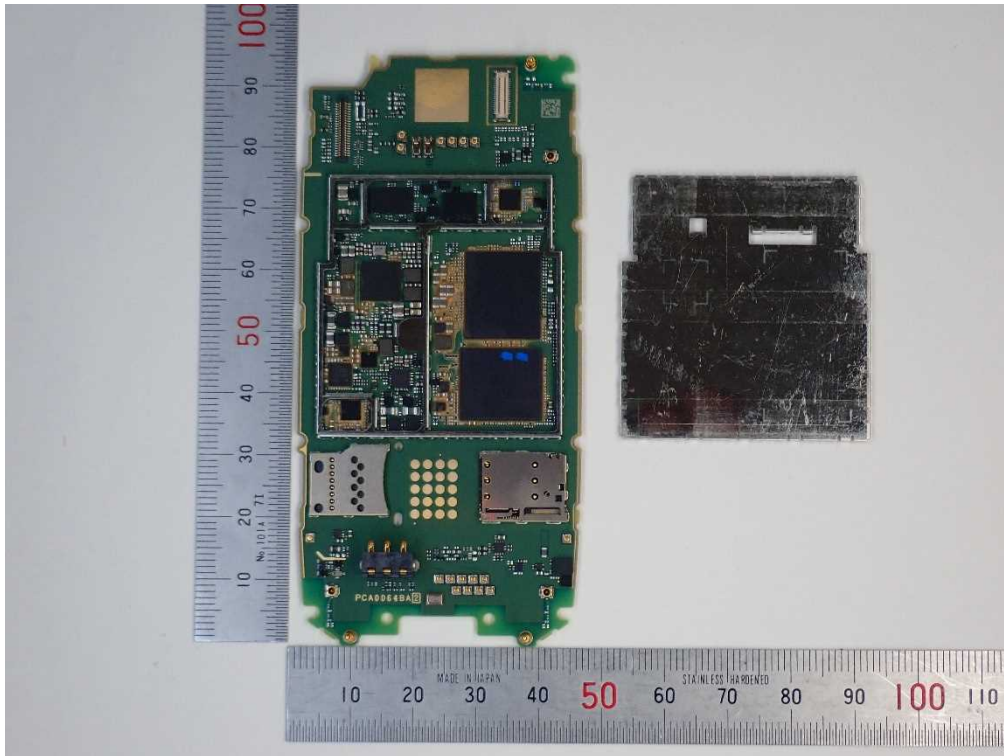
Main PCB rear (shield plate open)
