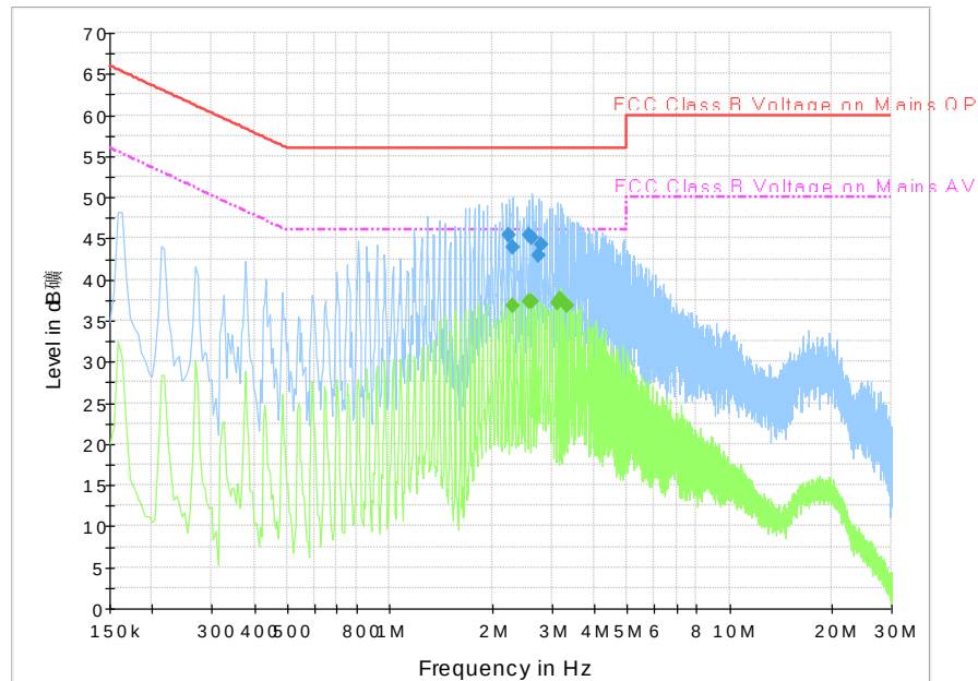
Fig.A.8.2 AC Powerline Conducted Emission-Iidle
