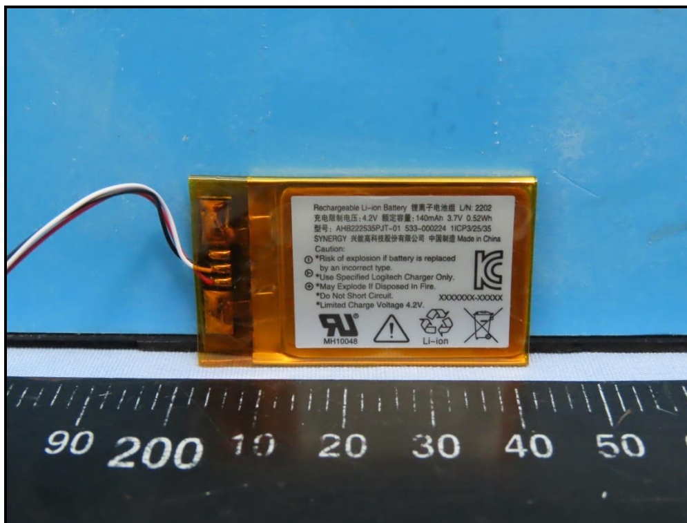
Battery 1 (Brand: SYNERGY, Model: AHB222535PJT-01 or 533-000224)
