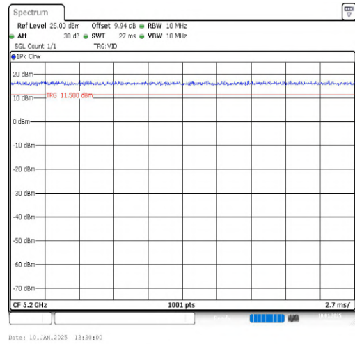
NTNV-11N20SISO-Ant1-5200
