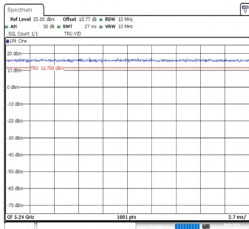
NTNV-11AC20SISO-Ant1-5240
