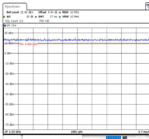
NTNV-11N40SISO-Ant1-5230
