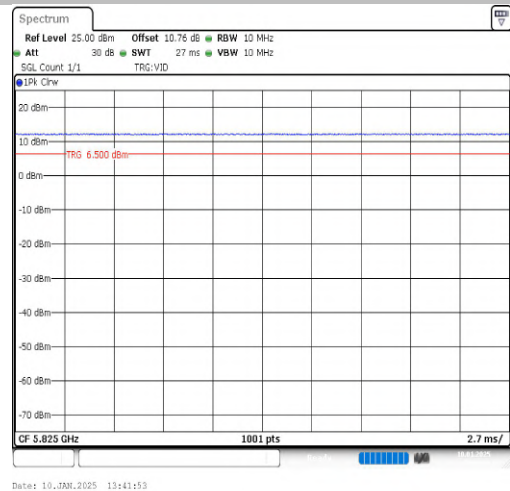
NTNV-11N20SISO-Ant1-5825
