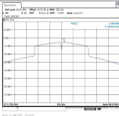
11N40SISO-Ant1-5795-PASS
