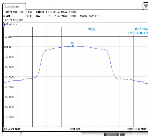
11AC20SISO-Ant1-5240-PASS
