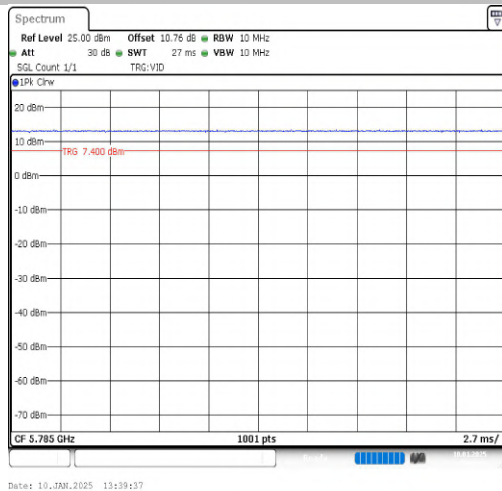
NTNV-11N20SISO-Ant1-5785
