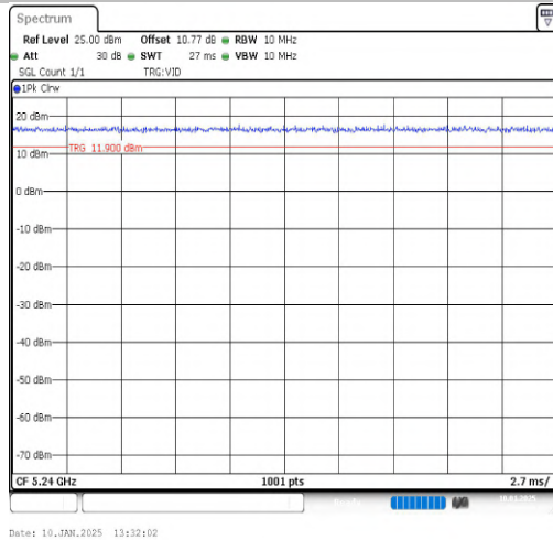
NTNV-11N20SISO-Ant1-5240
