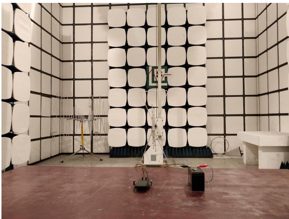
Radiated Emission below 1GHz- charge mode
