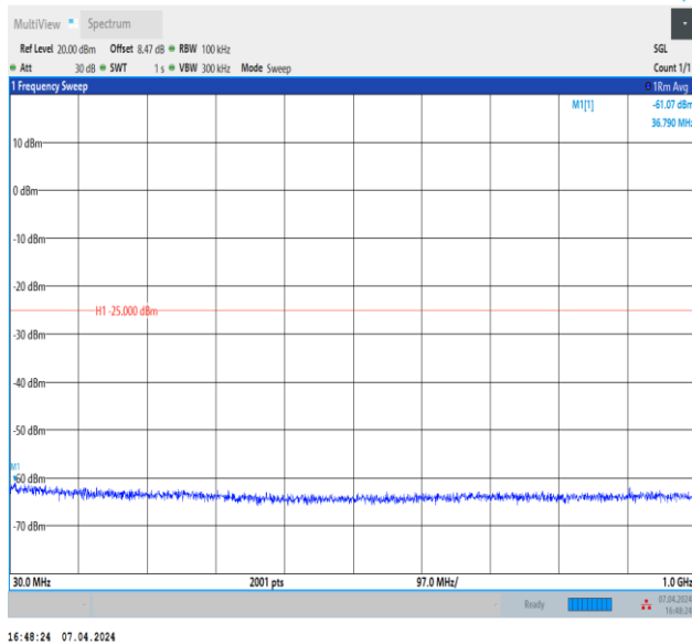
Band7_15MHz_QPSK_20825_1RB#0_30~1000_30~1000
