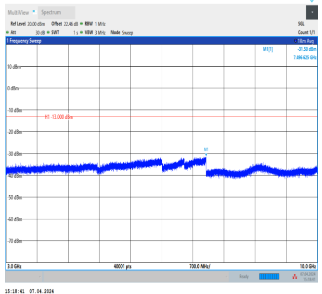
Band5_3MHz_QPSK_20415_1RB#0_3000~10000_3000~10000
