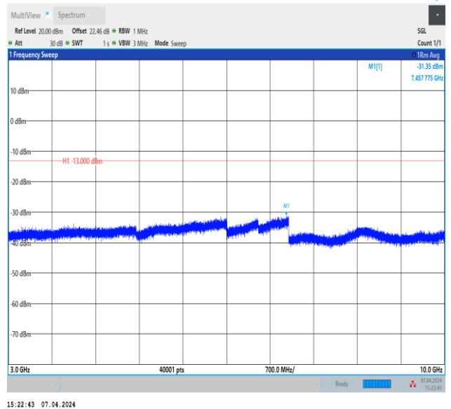
Band5_10MHz_QPSK_20450_1RB#0_3000~10000_3000~10000
