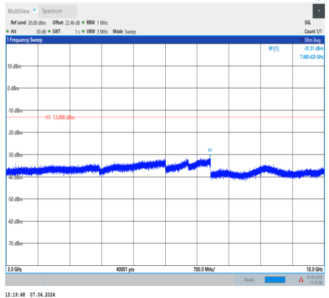
Band5_3MHz_QPSK_20635_1RB#0_3000~10000_3000~10 000
