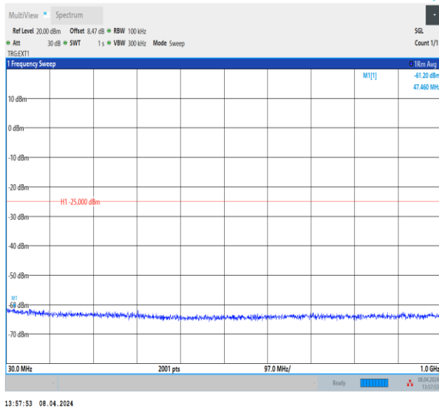
Band38_10MHz_QPSK_38000_1RB#0_30~1000_30~1000
