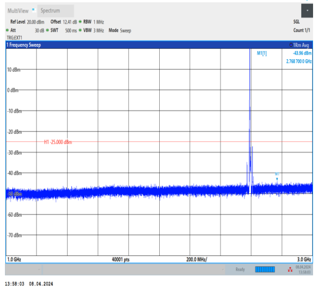
Band38_10MHz_QPSK_38000_1RB#0_1000~3000_1000~3000
