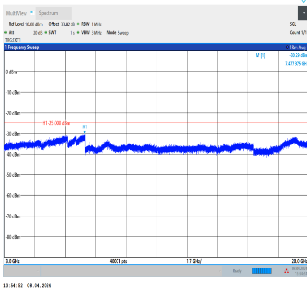
Band38_5MHz_QPSK_37775_1RB#0_3000~20000_3000~20000 0000
