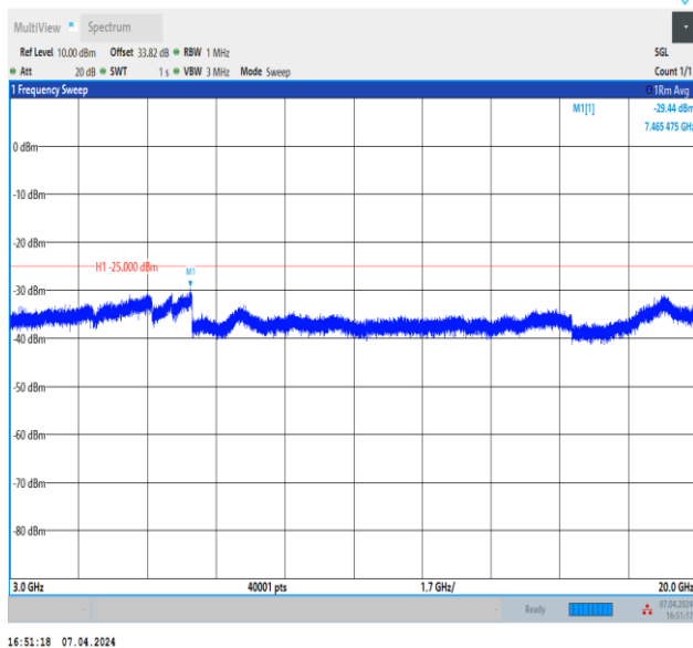
Band7_20MHz_QPSK_20850_1RB#0_3000~20000_3000~20000
