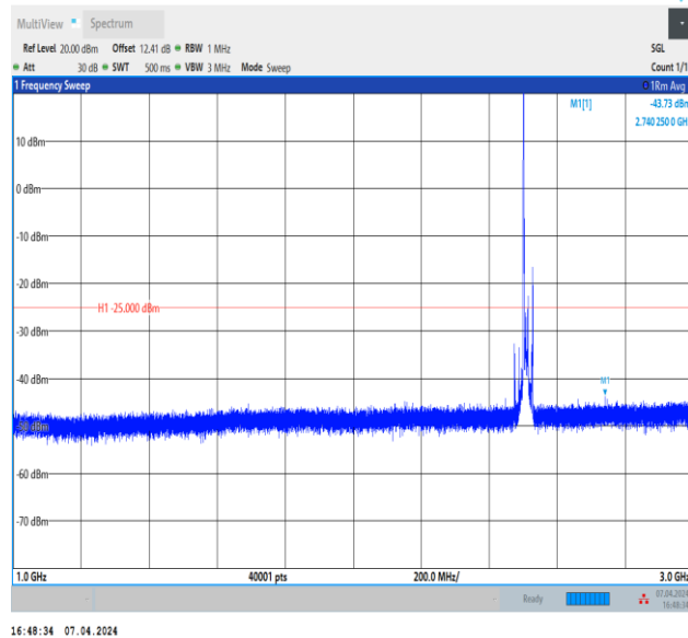
Band7_15MHz_QPSK_20825_1RB#0_1000~3000_1000~3000
