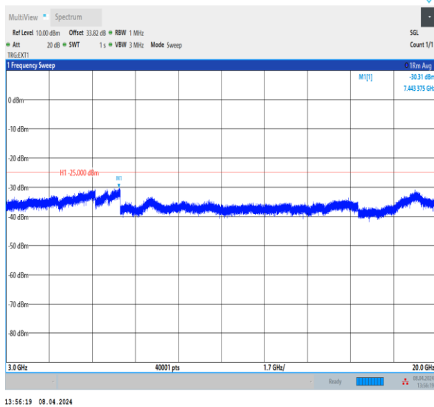
Band38_5MHz_QPSK_38225_1RB#0_3000~20000_3000~20000 0000
