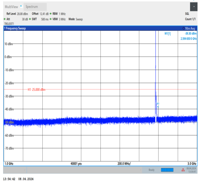
Band38_5MHz_QPSK_37775_1RB#0_1000~3000_1000~3000 00
