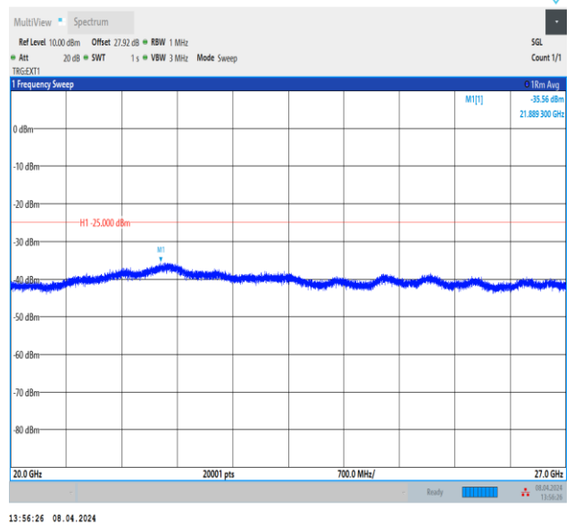
Band38_5MHz_QPSK_38225_1RB#0_20000~27000_20000~27000
