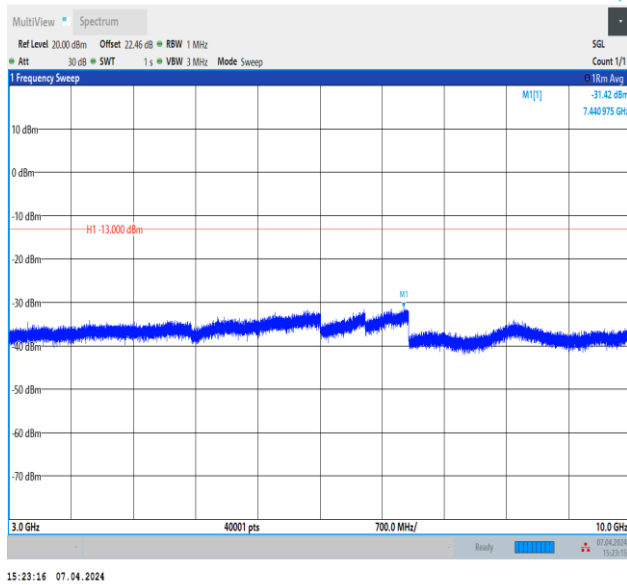
Band5_10MHz_QPSK_20525_1RB#0_3000~10000_3000~10000
