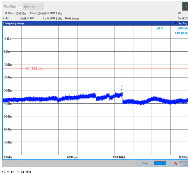
Band5_5MHz_QPSK_20425_1RB#0_3000~10000_3000~10000
