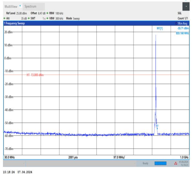
Band5_3MHz_QPSK_20415_1RB#0_30~1000_30~1000
