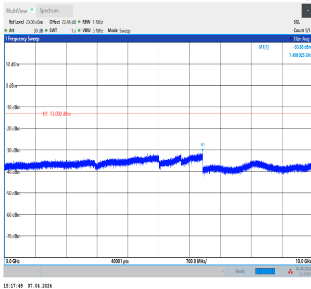
Band5_1.4MHz_QPSK_20643_1RB#0_3000~10000_3000~10000
