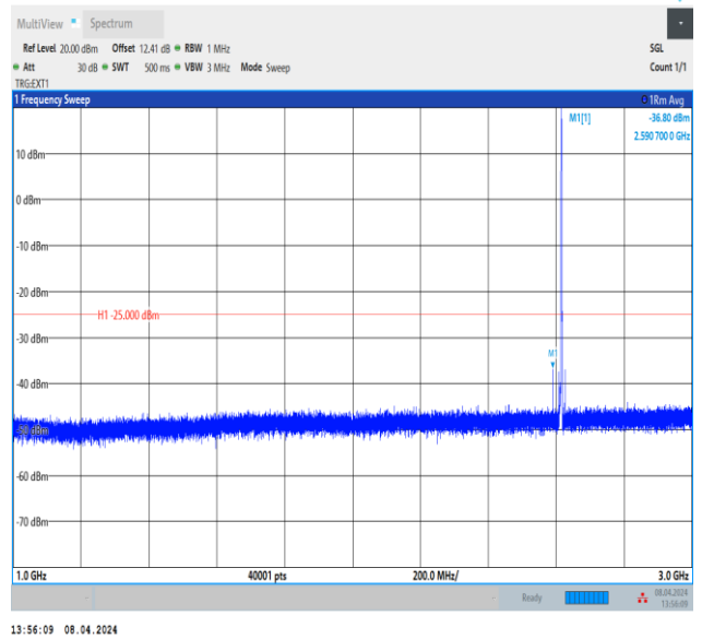
Band38_5MHz_QPSK_38225_1RB#0_1000~3000_1000~3000 00
