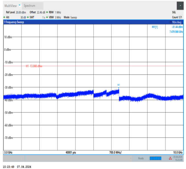
Band5_10MHz_QPSK_20600_1RB#0_3000~10000_3000~10000
