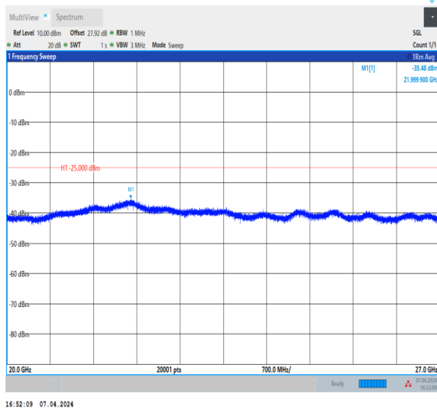
Band7_20MHz_QPSK_21100_1RB#0_20000~27000_20000~27000
