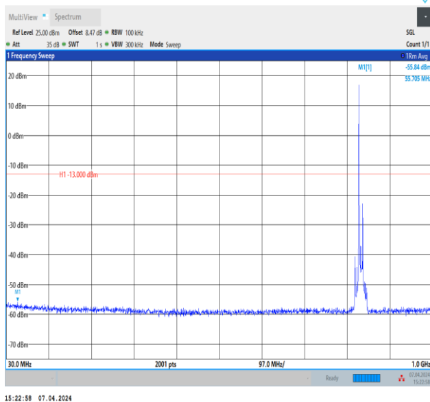
Band5_10MHz_QPSK_20525_1RB#0_30~1000_30~1000
