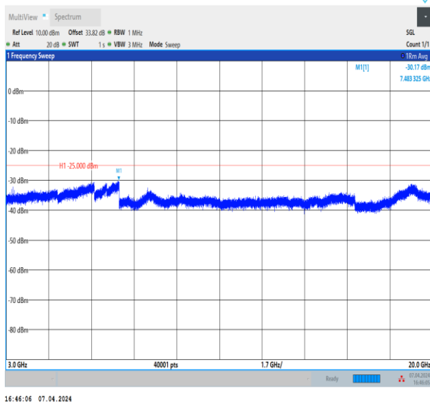
Band7_10MHz_QPSK_20800_1RB#0_3000~20000_3000~20000
