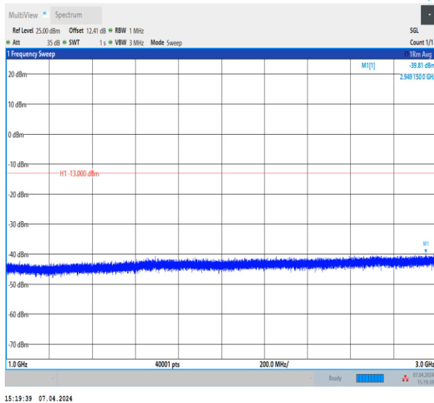
Band5_3MHz_QPSK_20635_1RB#0_1000~3000_1000~300 0
