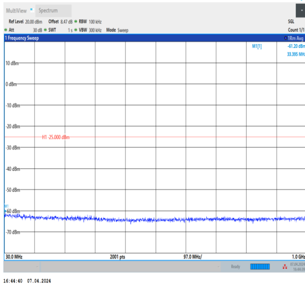
Band7_5MHz_QPSK_21425_1RB#0_30~1000_30~1000
