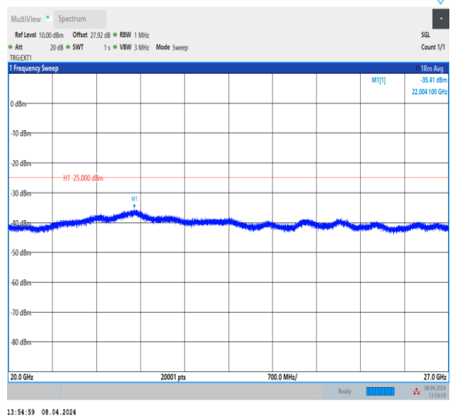
Band38_5MHz_QPSK_37775_1RB#0_20000~27000_20000~27000
