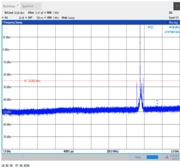
Band7_20MHz_QPSK_21350_1RB#0_1000~3000_1000~3000
