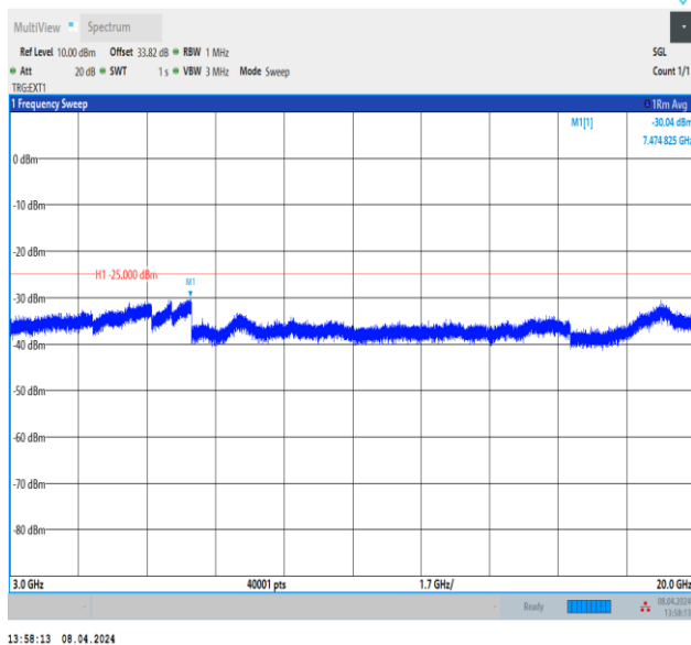
Band38_10MHz_QPSK_38000_1RB#0_3000~20000_3000~20000
