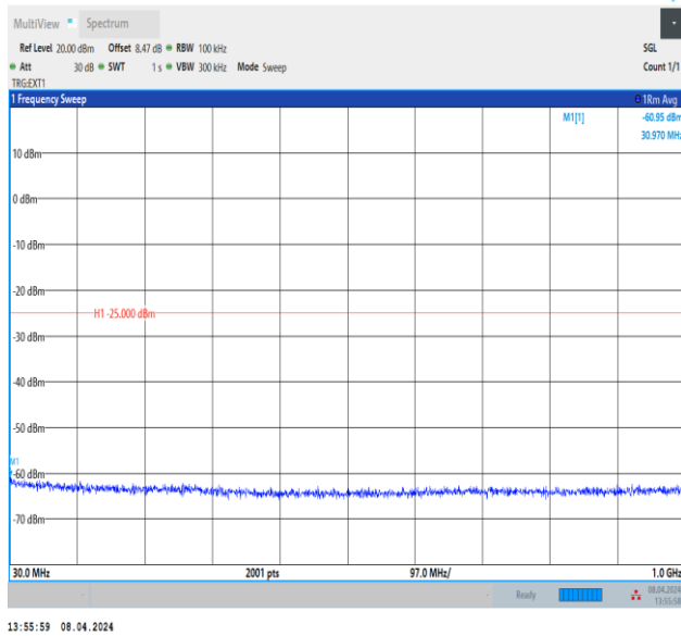
Band38_5MHz_QPSK_38225_1RB#0_30~1000_30~1000
