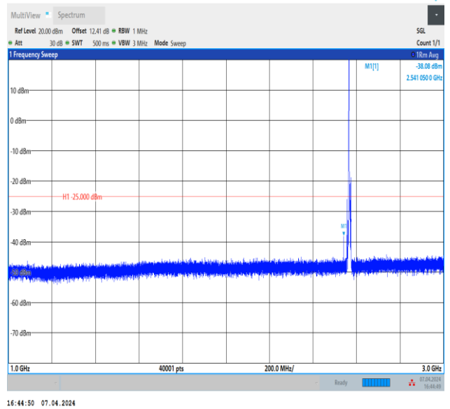
Band7_5MHz_QPSK_21425_1RB#0_1000~3000_1000~300 0
