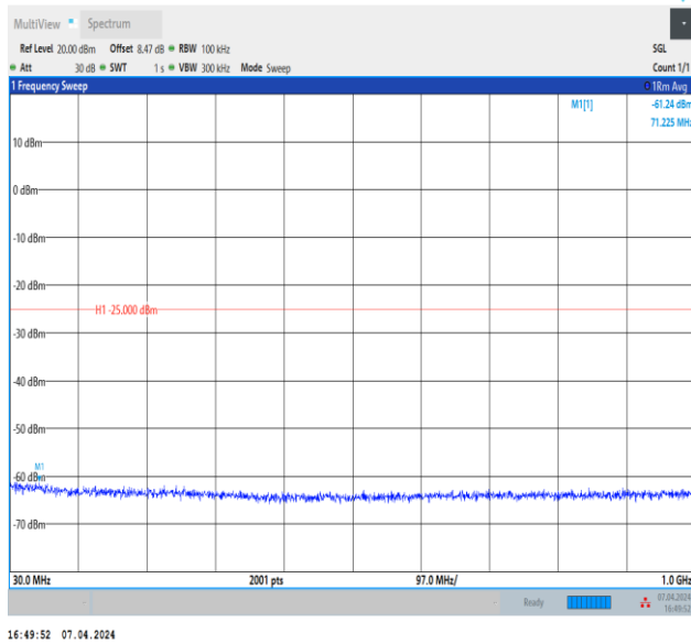
Band7_15MHz_QPSK_21375_1RB#0_30~1000_30~1000
