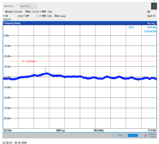
Band38_10MHz_QPSK_38000_1RB#0_20000~27000_20000~27000
