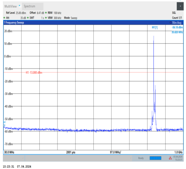
Band5_10MHz_QPSK_20600_1RB#0_30~1000_30~1000
