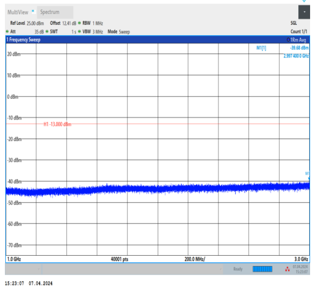
Band5_10MHz_QPSK_20525_1RB#0_1000~3000_1000~3000
