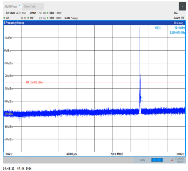
Band7_5MHz_QPSK_20775_1RB#0_1000~3000_1000~300 0
