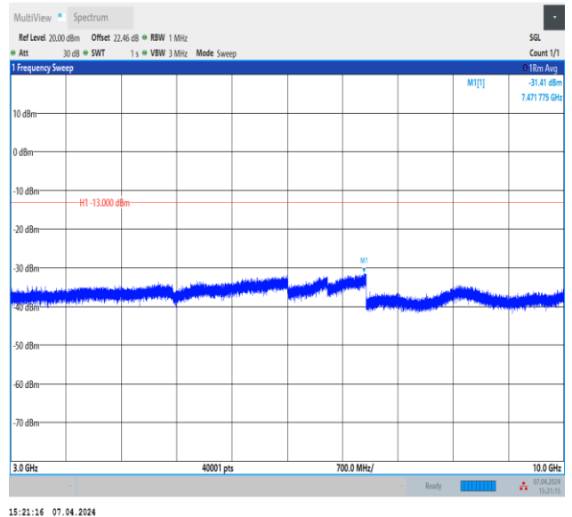
Band5_5MHz_QPSK_20525_1RB#0_3000~10000_3000~10000
