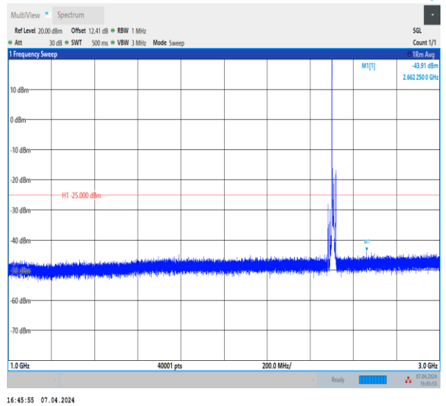
Band7_10MHz_QPSK_20800_1RB#0_1000~3000_1000~3000
