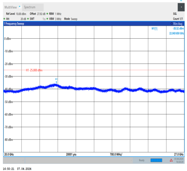
Band7_15MHz_QPSK_21375_1RB#0_20000~27000_20000~27000
