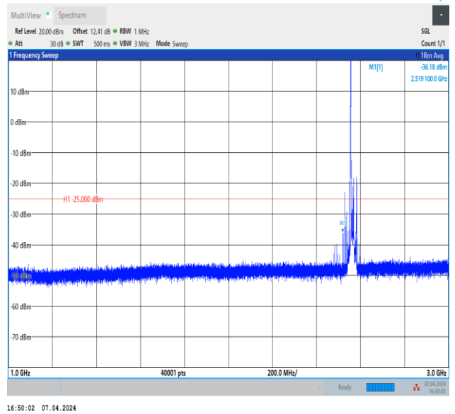
Band7_15MHz_QPSK_21375_1RB#0_1000~3000_1000~3000
