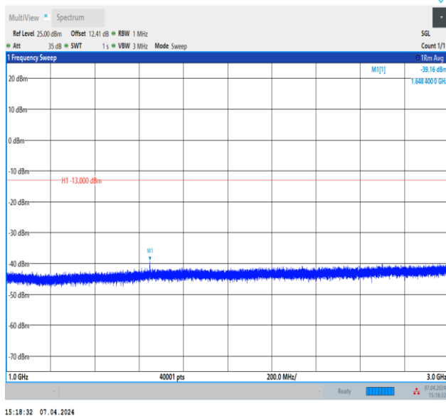
Band5_3MHz_QPSK_20415_1RB#0_1000~3000_1000~300 0
