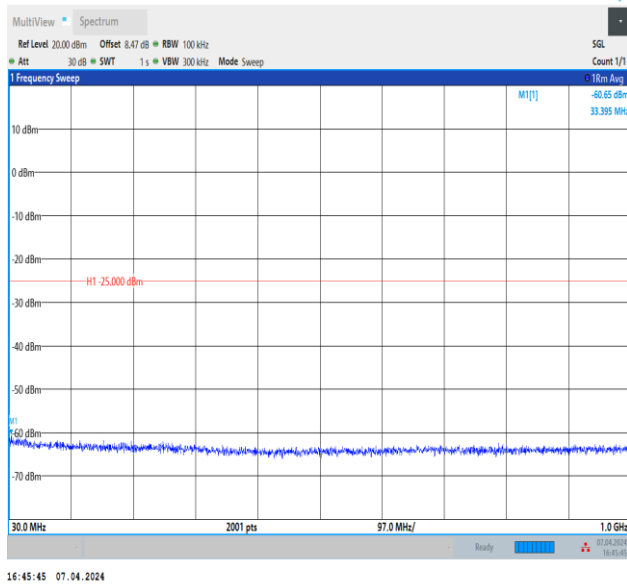
Band7_10MHz_QPSK_20800_1RB#0_30~1000_30~1000
