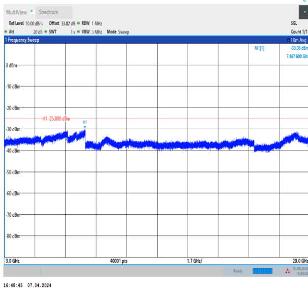
Band7_15MHz_QPSK_20825_1RB#0_3000~20000_3000~20000
