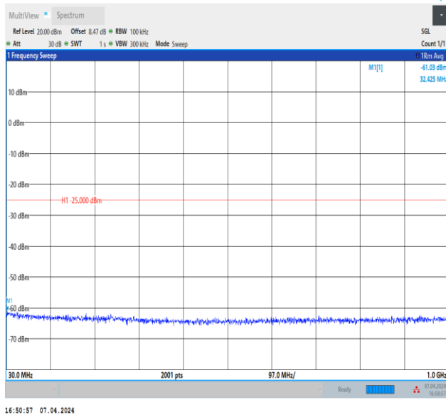
Band7_20MHz_QPSK_20850_1RB#0_30~1000_30~1000
