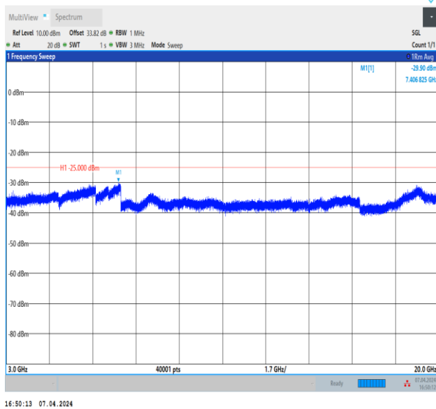
Band7_15MHz_QPSK_21375_1RB#0_3000~20000_3000~20000
