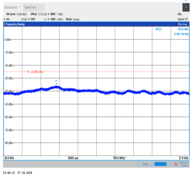
Band7_10MHz_QPSK_20800_1RB#0_20000~27000_20000~27000
