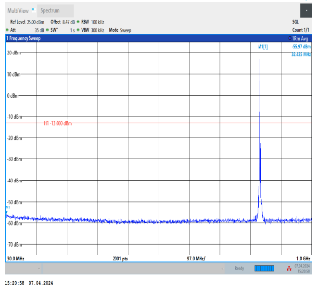
Band5_5MHz_QPSK_20525_1RB#0_30~1000_30~1000
