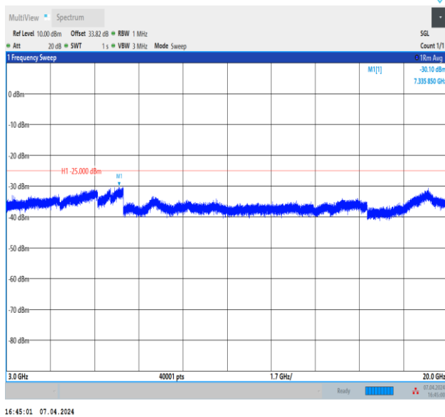
Band7_5MHz_QPSK_21425_1RB#0_3000~20000_3000~20 000
