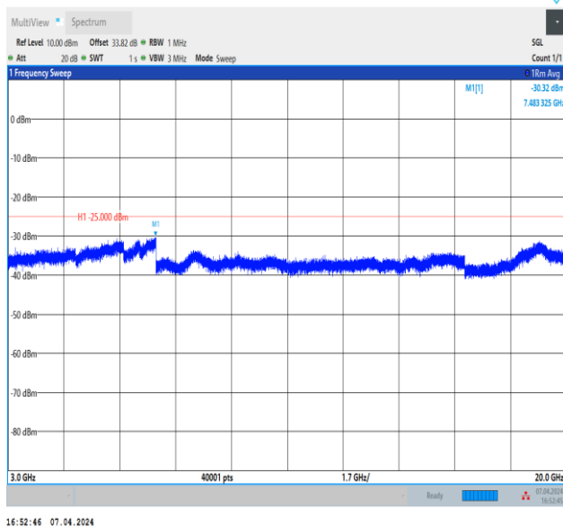
Band7_20MHz_QPSK_21350_1RB#0_3000~20000_3000~20000
