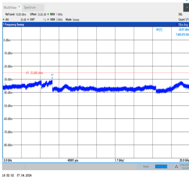
Band7_20MHz_QPSK_21100_1RB#0_3000~20000_3000~20000 0000
