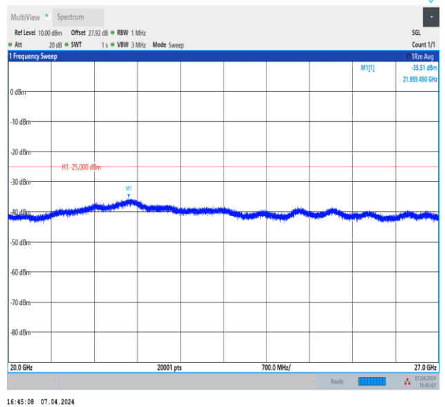
Band7_5MHz_QPSK_21425_1RB#0_20000~27000_20000~ 27000
