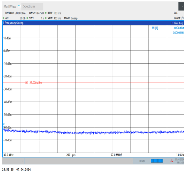
Band7_20MHz_QPSK_21350_1RB#0_30~1000_30~1000
