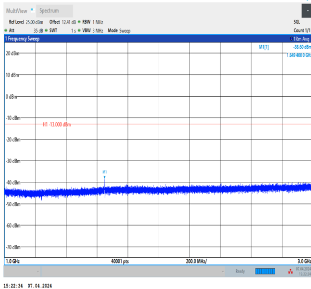
Band5_10MHz_QPSK_20450_1RB#0_1000~3000_1000~3000
