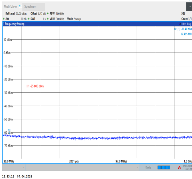
Band7_5MHz_QPSK_20775_1RB#0_30~1000_30~1000
