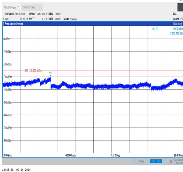
Band7_5MHz_QPSK_20775_1RB#0_3000~20000_3000~20 000
