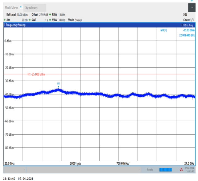
Band7_5MHz_QPSK_20775_1RB#0_20000~27000_20000~ 27000
