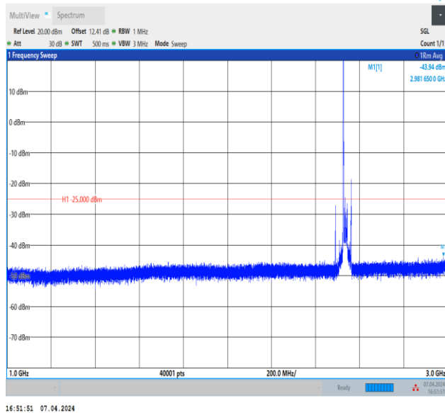
Band7_20MHz_QPSK_21100_1RB#0_1000~3000_1000~3000 00
