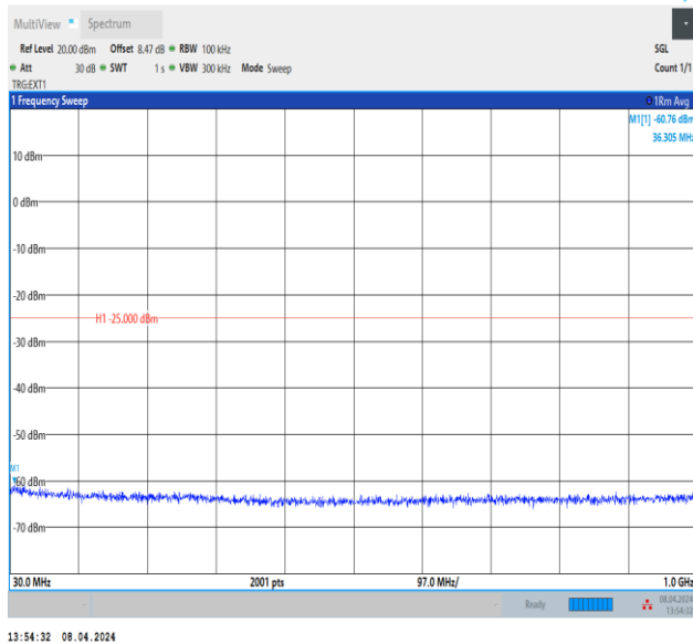
Band38_5MHz_QPSK_37775_1RB#0_30~1000_30~1000
